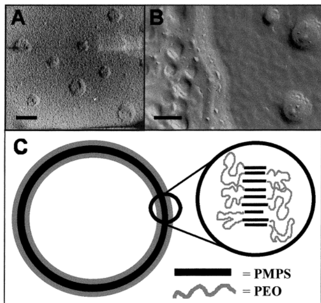
Figure 3. (a, b) TEM images of vesicle dispersions of \text{PMPS}_n\text{-PEO}_m showing (a) a replica of intact (freeze fracturing) and (b) collapsed vesicles (platinum shadowing); bars represent 200 nm. (c) Schematic representation of the proposed structure of the vesicles showing the hydrophobic PMPS interior (black) shielded from the aqueous phase by the hydrophilic PEO layers (gray).
