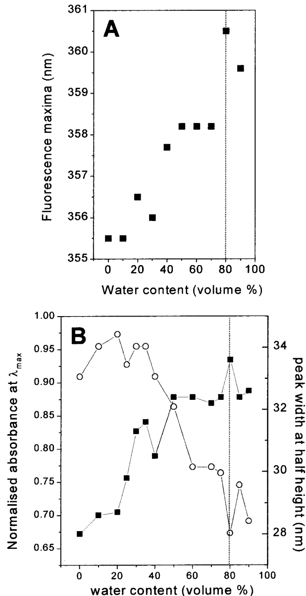
Figure 4. Changes of the fluorescence and UV spectra of \text{PMPS}_n\text{-PEO}_m in various THF/water mixtures. (a) The position of fluorescence maxima and (b) the intensity (O) and peak width (■) of the \sigma\text{-}\sigma^* transition band as a function of the water concentration.
