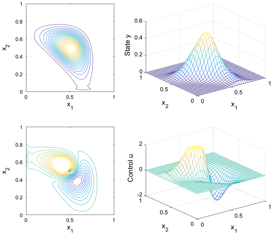
Fig. 2 Contour and mesh plots of the solution to the convection-diffusion control example with state and control constraints, for state variable y (top) and control variable u (bottom), with \beta = 10^{-2}
