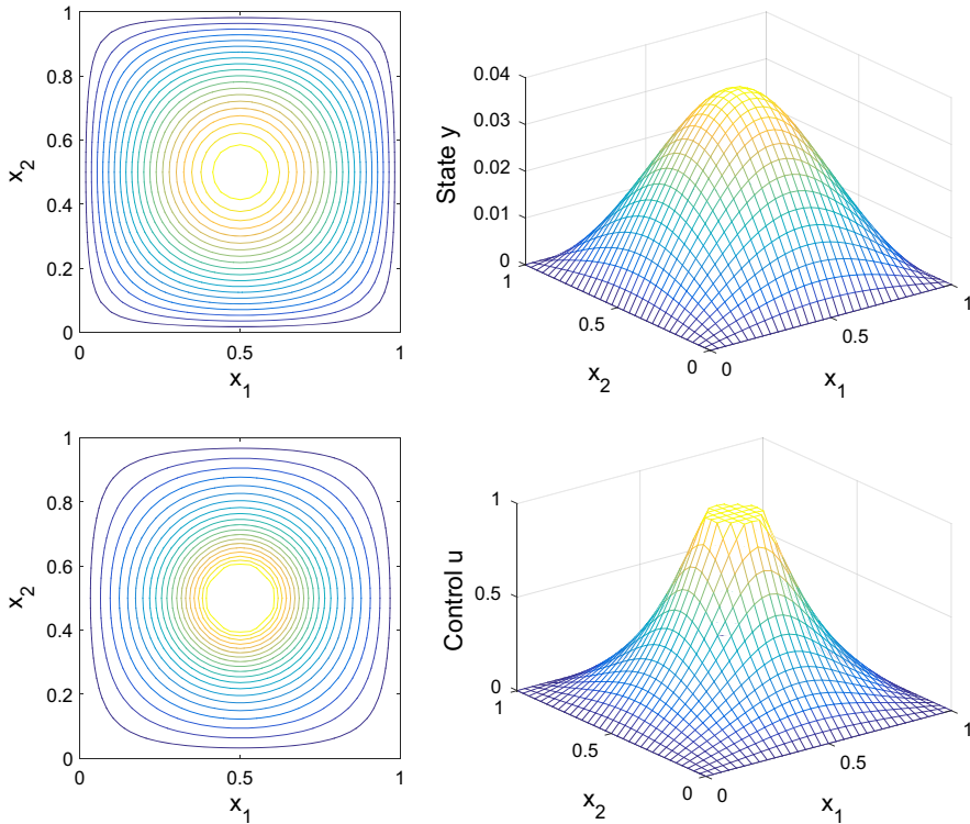
Fig. 1 Contour and mesh plots of the solution to the Poisson control example with control constraints, for state variable y (top) and control variable u (bottom), with \beta = 10^{-2}
