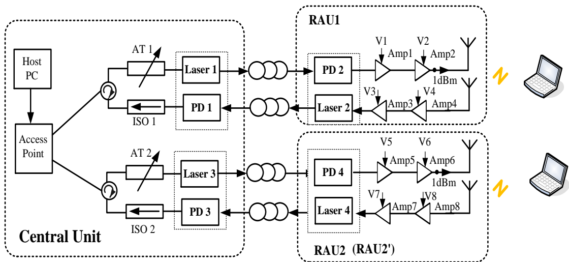
Figure 3.2 The experiment set-up. PD=Photodetector, AT=Attenuator, V=Voltage, ISO=Isolator, Amp=Amplifier.
