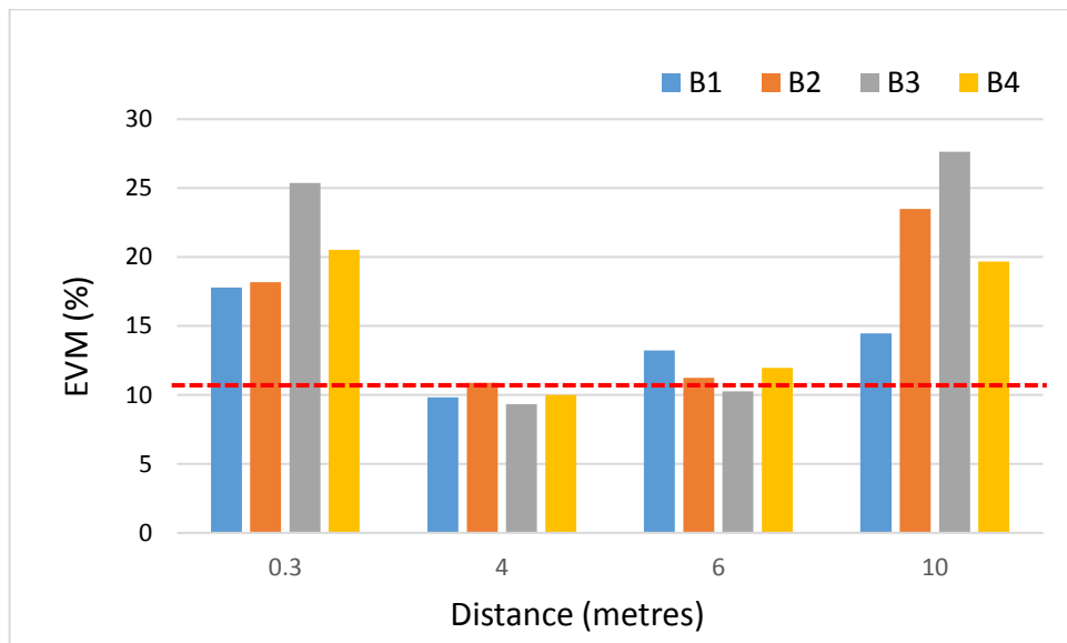
Figure 4.25 EVM of downlink 2x2 ZF-MIMO measured at inter-RAU distance of 0.3m, 4-m, 6-m and 10-m at different positions A1-A4 (top) and B1-B4 (bottom).
