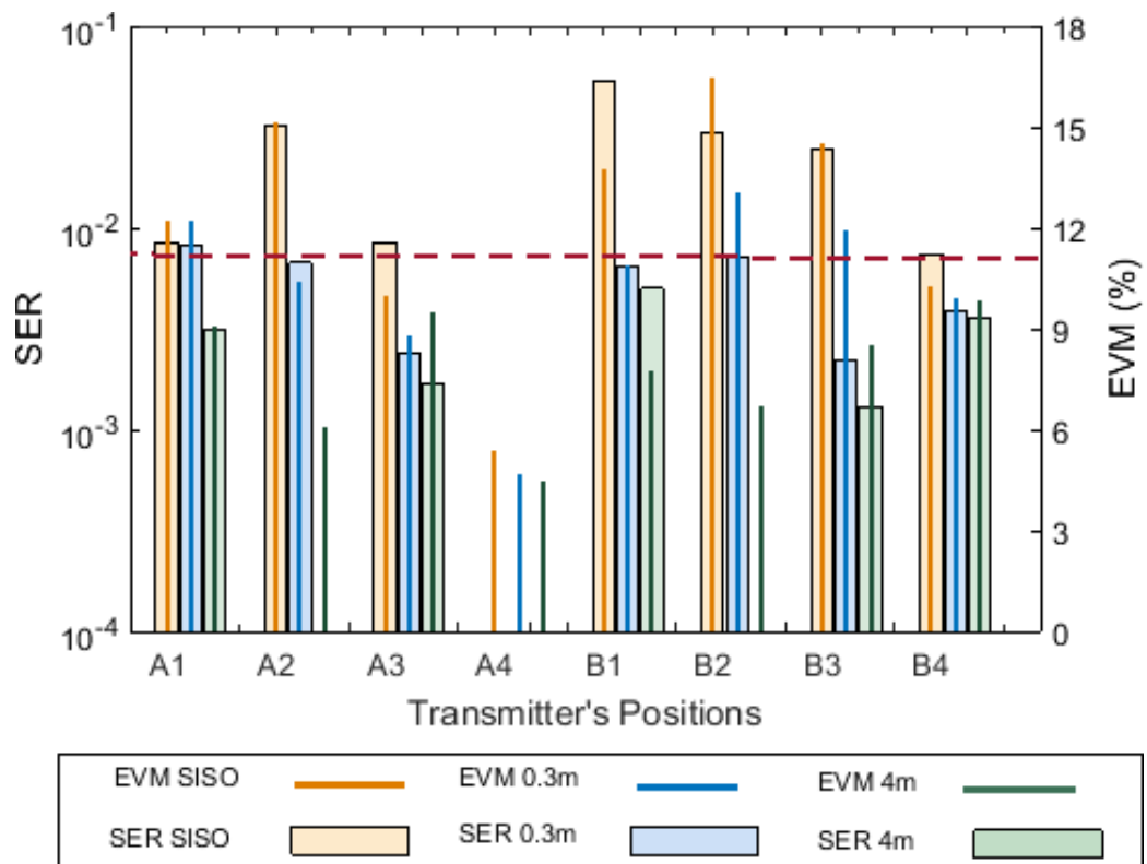
Figure 4.6 SER and EVM of uplink 1x2 SC-SIMO measured at inter-RAU distance of 0.3m and 4m at different positions compared to SISO
