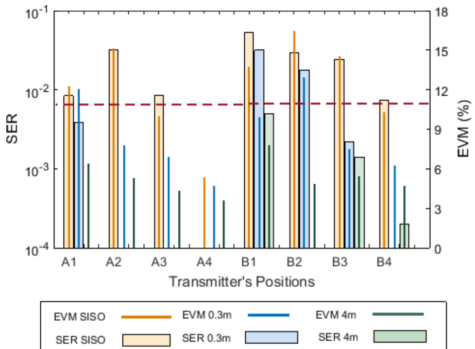
Figure 4.8 SER and EVM of uplink 1x2 MRC-SIMO measured at inter-RAU distance of 0.3m and 4m at different positions compared to SISO .
