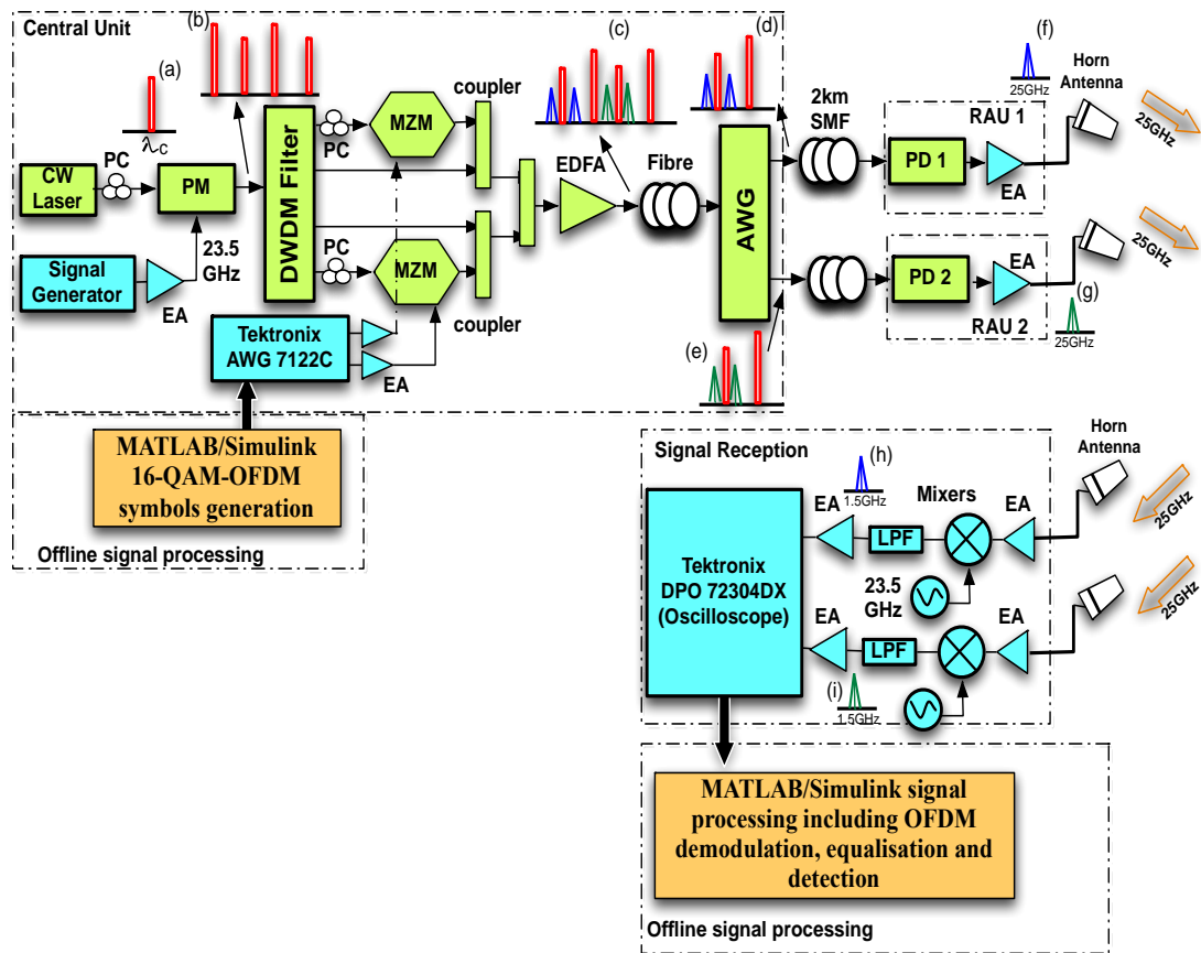
Figure 5.2 Experimental set-up for 25GHz RoF-transported 2x2 MIMO system CW Laser – Continuous-wave Laser, PM- phase modulator, DWDM filter – dense wavelength division multiplexing filter, EA= Electric amplifiers, MZM –Mach-Zehnder modulator, EDFA- Erbium Doped Fibre Amplifier, AWG - Array Waveform Grating, PD=Photo-detector, RAU=Remote antenna unit, LPF – low pass filter
