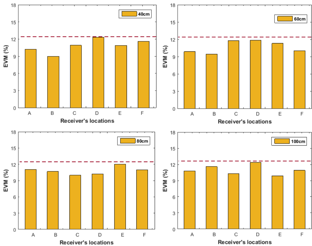
Figure 5.13 EVM result of 2x2 spatial diversity-MIMO at receiver location A to F for 40cm, 60cm, 80cm and 100cm transmit antenna separation distances at 3m wireless transmission distance.
