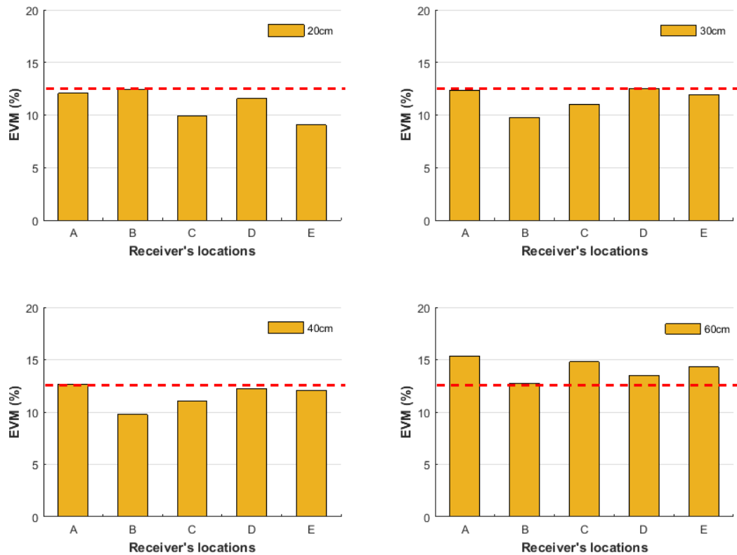
Figure 5.22 EVM result of 60GHz experiment at 20cm, 30cm, 40cm and 60cm transmit antenna separation distances using zero-forcing spatial multiplexing algorithm.
