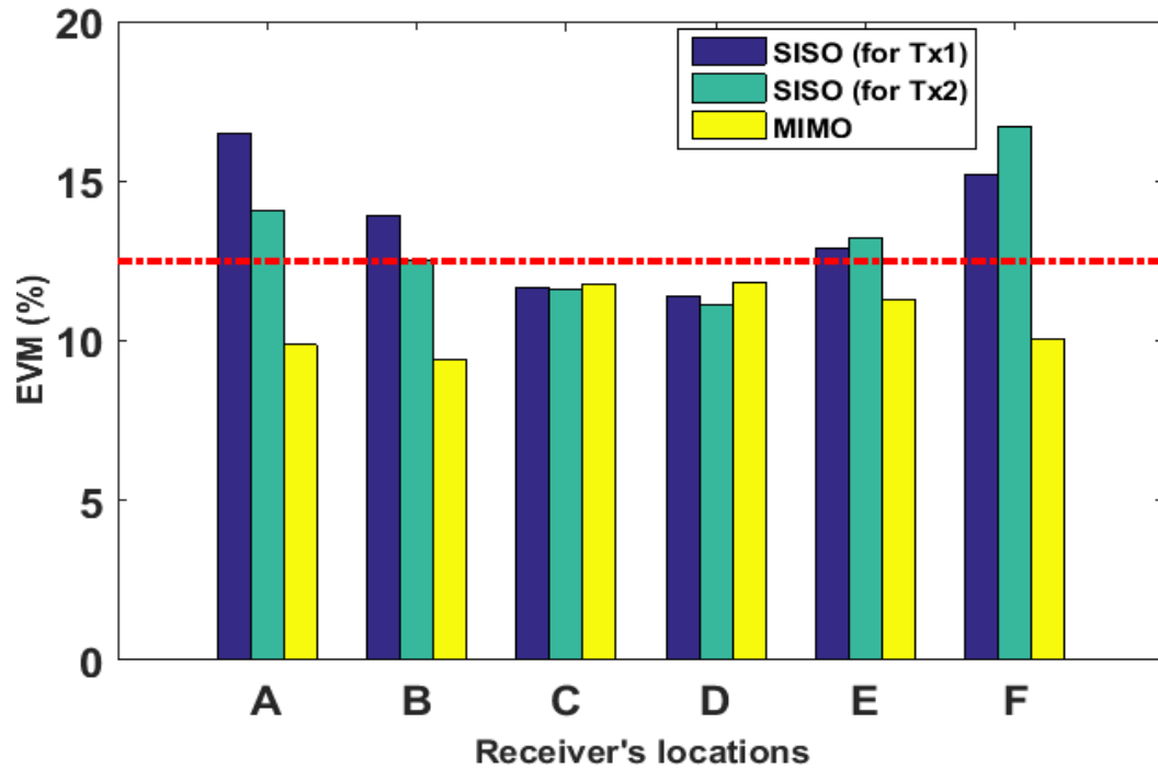
Figure 5.16 EVM results of 2x2 spatial diversity-MIMO using Alamouti STBC at different user locations compared with the performance of SISO system.
