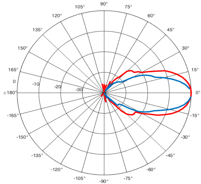
Figure 5.12 Radiation pattern of the two transmitting horn antennas.
