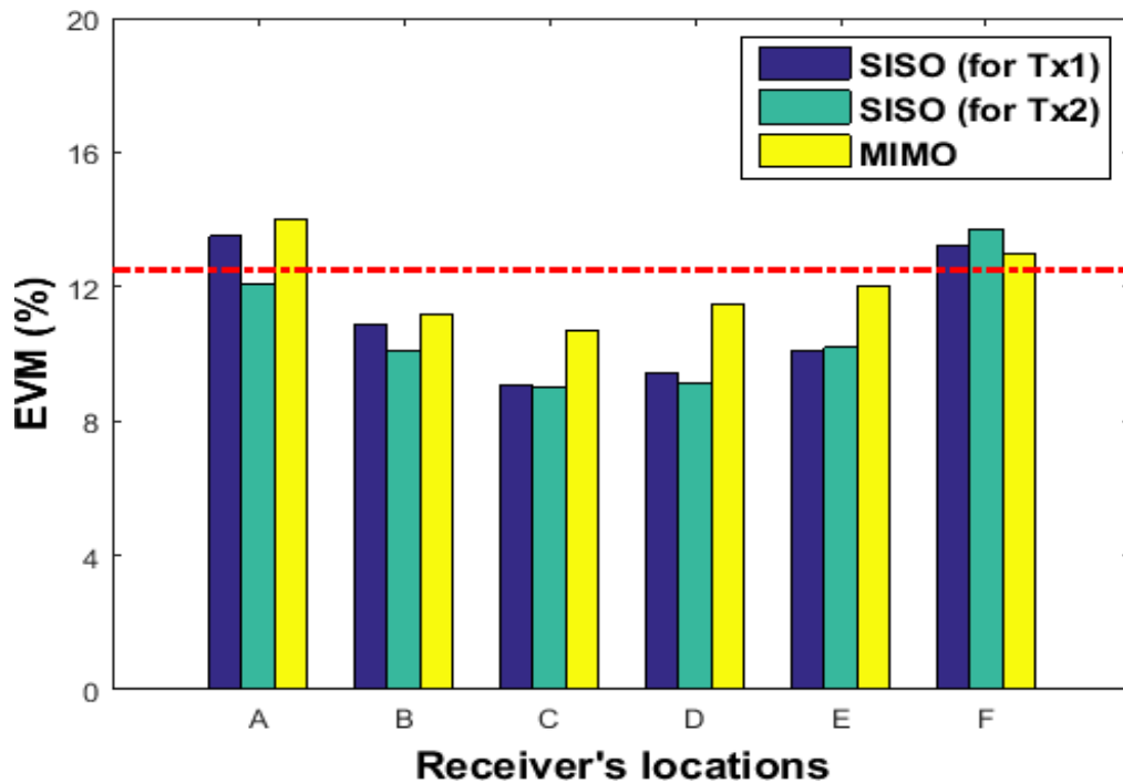
Figure 5.19 EVM of SISO with 0.5Gb/s at different receiver locations compared to spatial multiplexing-MIMO with each antenna transmitting 0.5Gbps.
