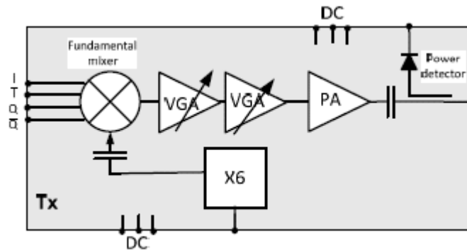
Figure 5.7 gTSC0020 60GHz integrated transmitter circuit [12].
