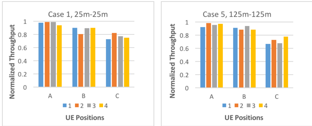
Figure 3.9 MIMO-supported downlink throughput with the equal fibre link lengths (a) Case 1, 25m-25m (b) Case 5, 125m-125m
