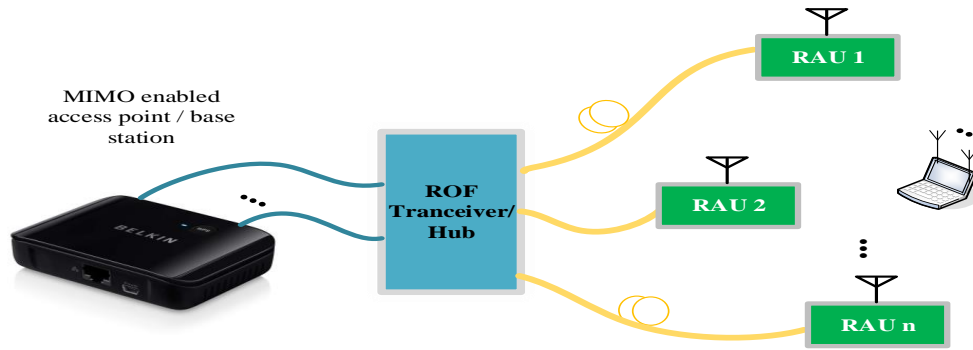
Figure 2.14 Diagram showing 2x2 MIMO over RoF DAS.
