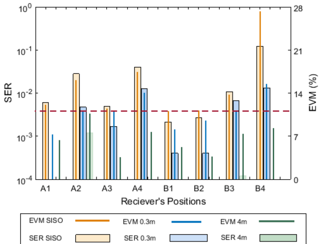
Figure 4.10 SER and EVM of downlink 2x1 Alamouti STBC-MISO measured at inter-RAU distance of 0.3m and 4m at different positions compared to SISO
