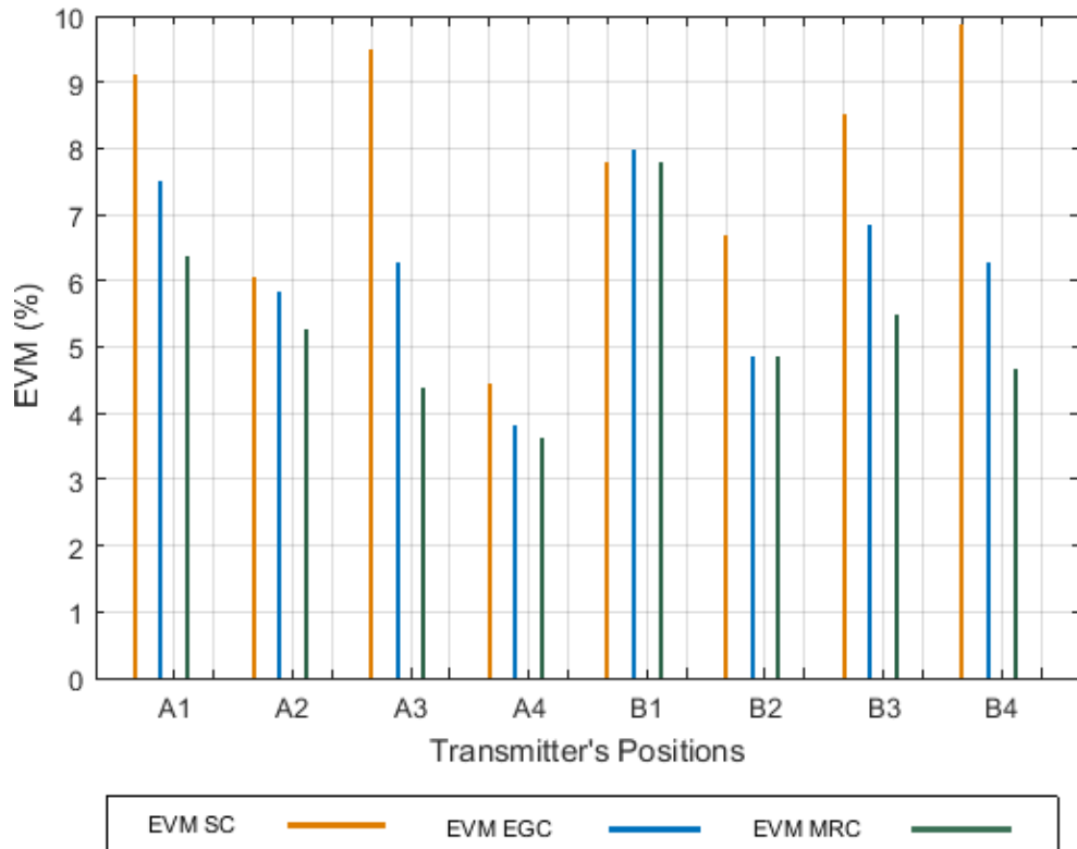
Figure 4.9 EVM of SC, EGC and MRC SIMO scheme measured at inter-RAU distance 4m at different positions A, B (1-4)
