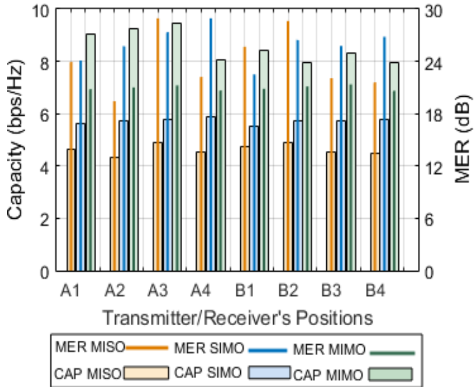
Figure 4.22 Capacity and MER of Alamouti STBC-MISO, MRC-SIMO and ZF-MIMO measured at inter-RAU distance of 4m at different positions.
