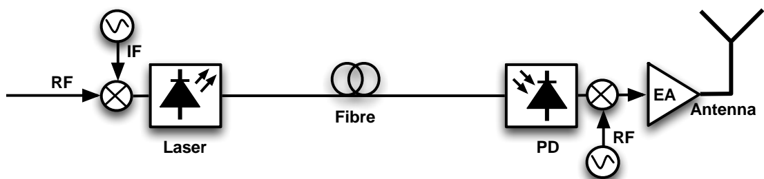
Figure 2.4 IF-over-fibre link.
