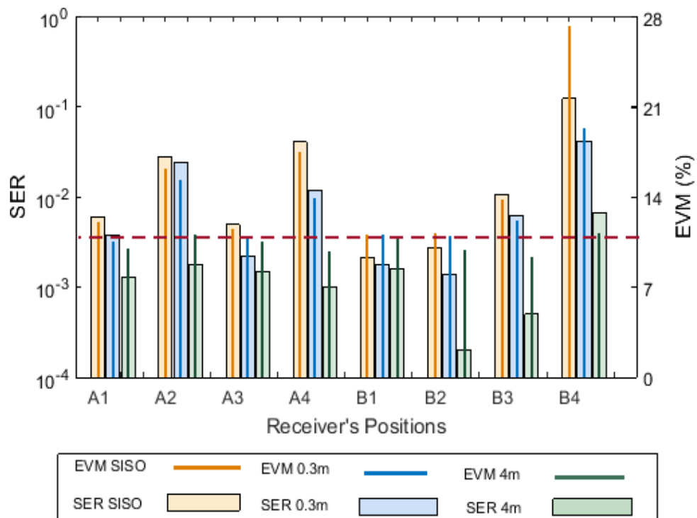
Figure 4.12 SER and EVM of downlink 2x1 DD-MISO measured at inter-RAU distance of 0.3m and 4m at different positions compared to SISO
