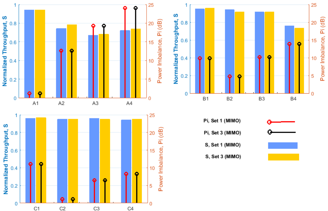
Figure 3.13 Throughput S and power imbalance P_i results of MIMO using set 1 and set 3
