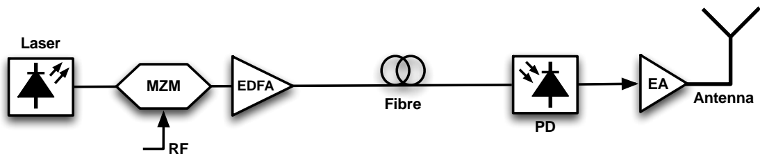
Figure 2.6 Diagram showing RoF link using external Mach Zehnder modulator.
