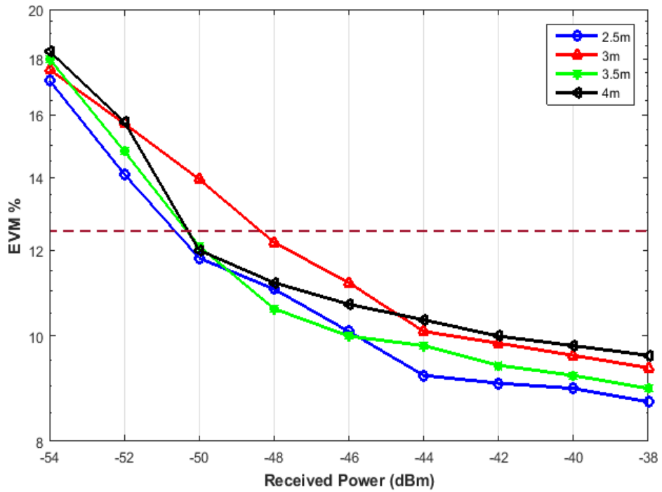
Figure 5.17 EVM results of 2x2 spatial diversity-MIMO using Alamouti STBC algorithm as the received power is increased for 2.5m, 3m, 3.5m and 4m wireless transmission distances at 80cm transmit antenna separation distance.
