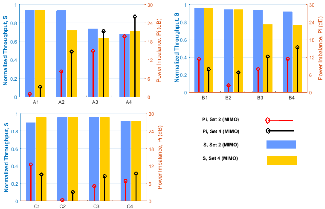
Figure 3.14 Throughput S and power imbalance Pi results of MIMO using set 2 and set 4
