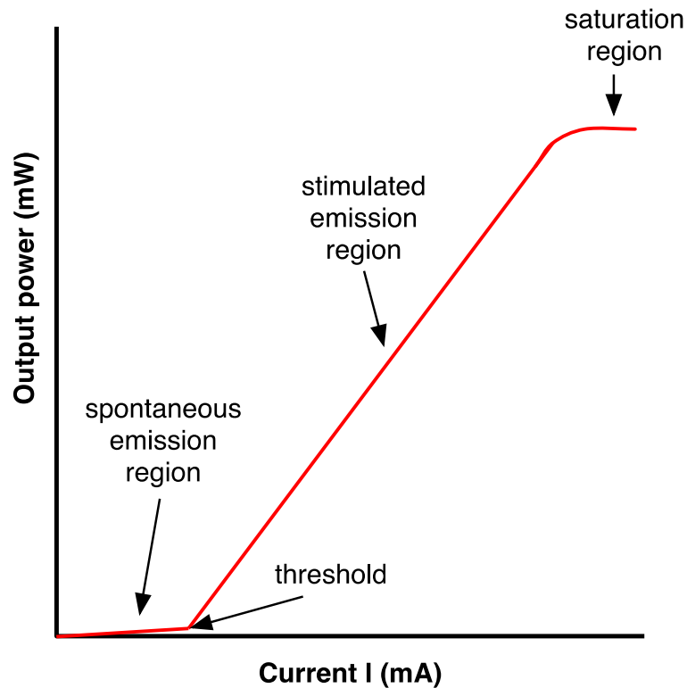
Figure 2.7 Laser P-I curve.
