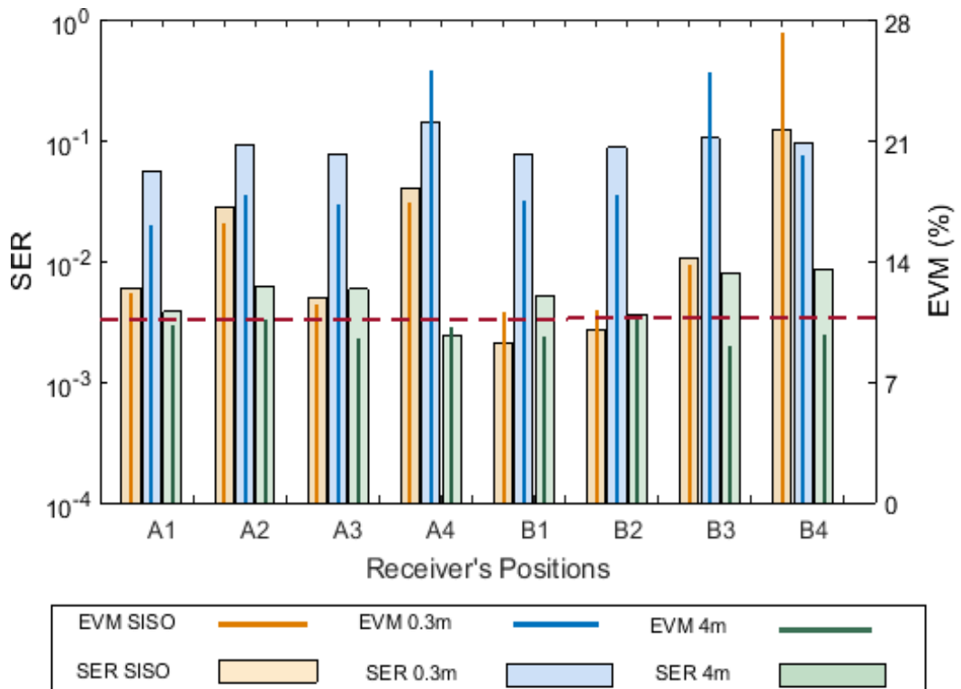
Figure 4.14 SER and EVM of downlink 2x2 ZF-MIMO measured at inter-RAU distance of 0.3m and 4m at different positions compared to SISO.
