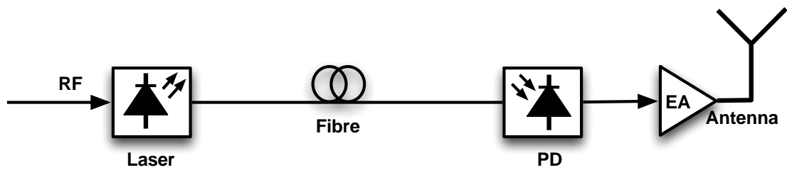
Figure 2.3 RF-over-fibre link.
