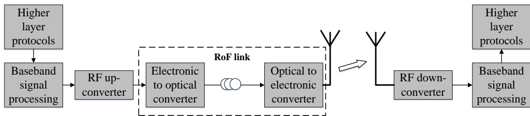
Figure 2.2 Radio-over-fibre link.
