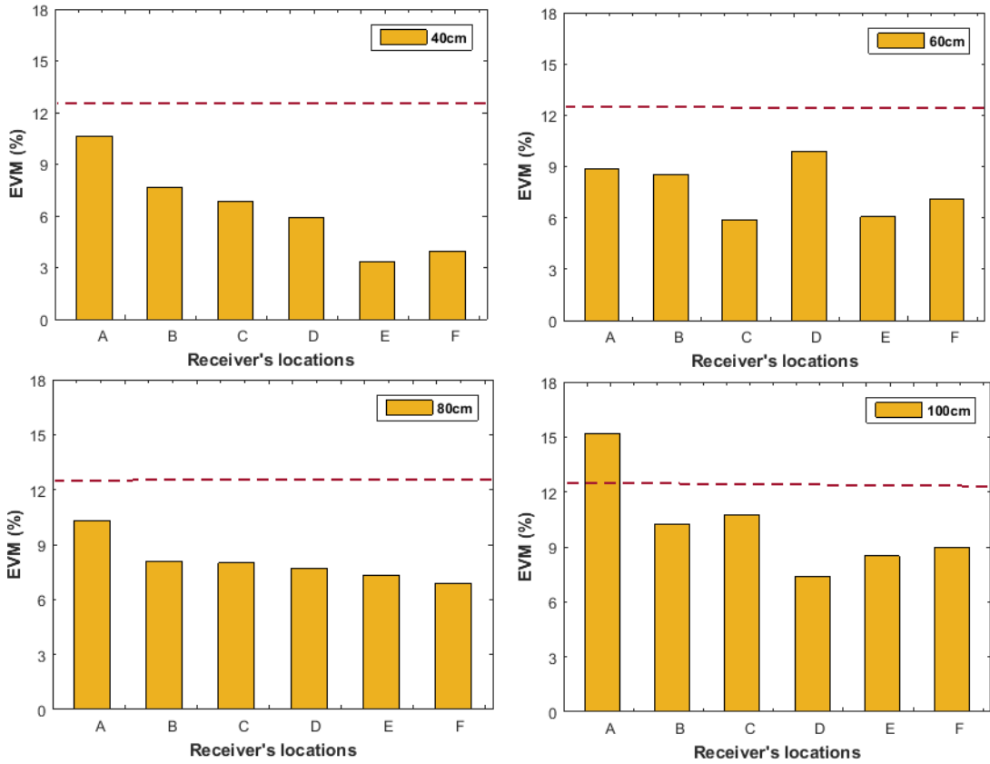
Figure 5.15 EVM result of 2x2 spatial diversity-MIMO at receiver location A to F for 40cm, 60cm, 80cm and 100cm transmit antenna separation distances at 4m wireless transmission distance.
