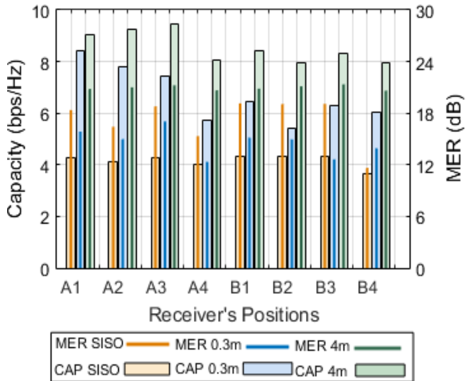
Figure 4.21 Capacity and MER of downlink 2x2 ZF-MIMO measured at inter-RAU distance of 0.3m and 4m at different positions compared to SISO .
