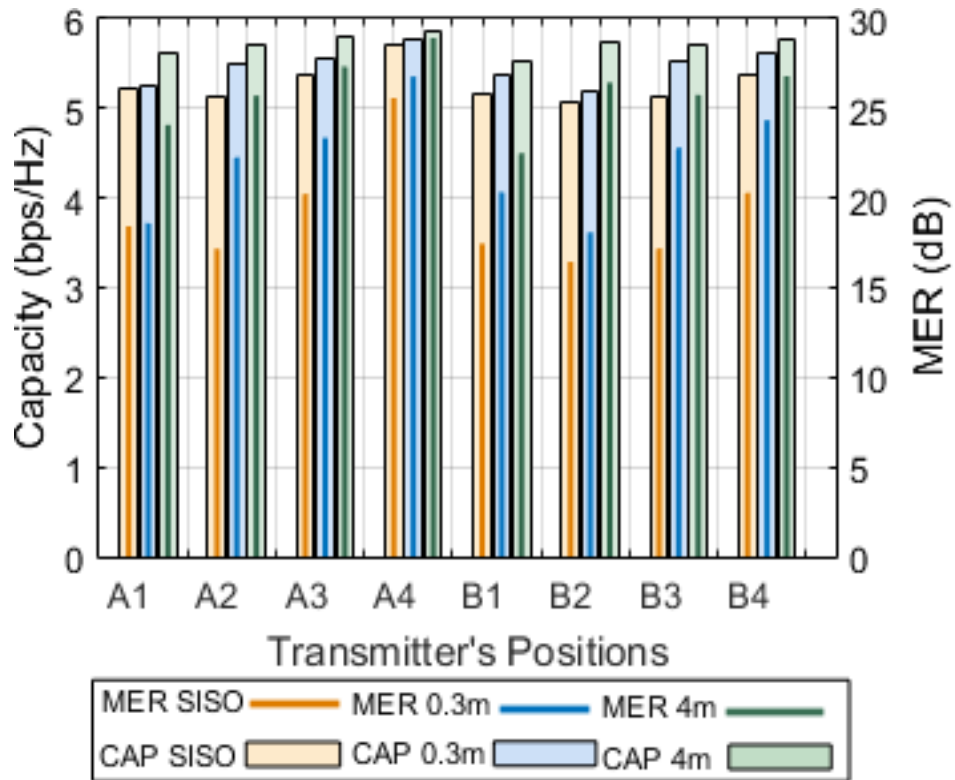
Figure 4.20 Capacity and MER of downlink 1x2 MRC-SIMO measured at inter-RAU distance of 0.3m and 4m at different positions compared to SISO .
