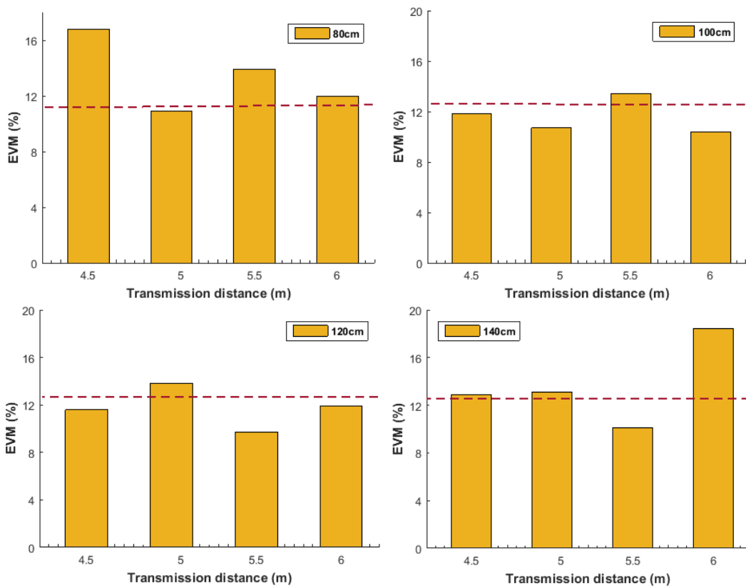
Figure 5.18 EVM result of 2x2 spatial multiplexing-MIMO for 80cm, 100cm, 120cm and 140cm transmit antenna separation distances at 4.5m, 5m, 5.5m and 6m wireless transmission distance.
