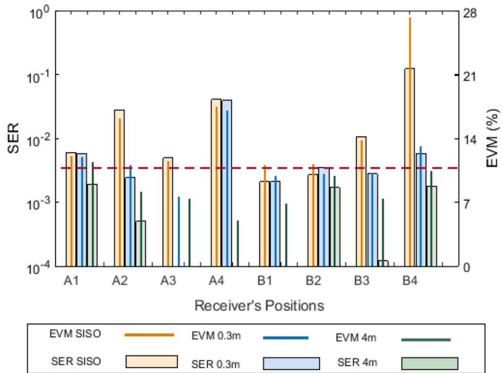
Figure 4.11 SER and EVM of downlink 2x1 TAS-MISO measured at inter-RAU distance of 0.3m and 4m at different positions compared to SISO .
