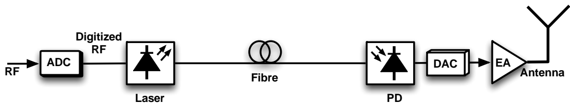
Figure 2.5 Digitized-RF-over-fibre link.
