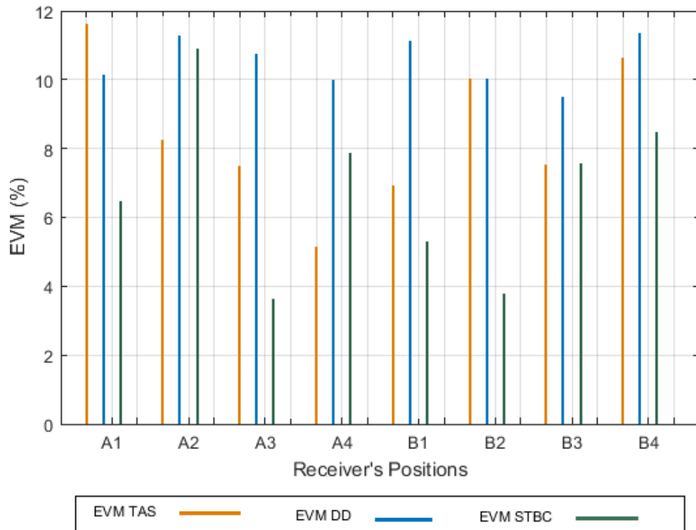
Figure 4.13 EVM of TAS , DD and Alamouti STBC-MISO scheme measured at inter-RAU distance 4m at different positions A, B (1-4)
