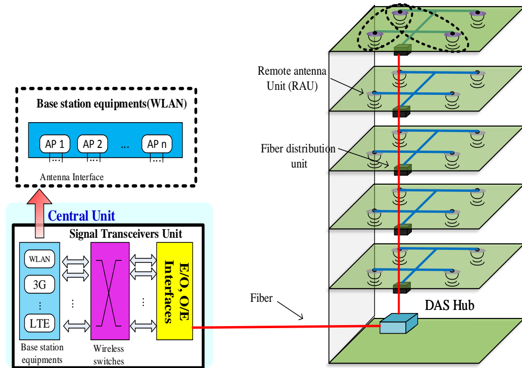
Figure 1.2 RoF-based DAS
