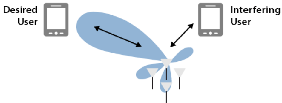
Figure 2.12 Smart antenna system - beamforming [22].
