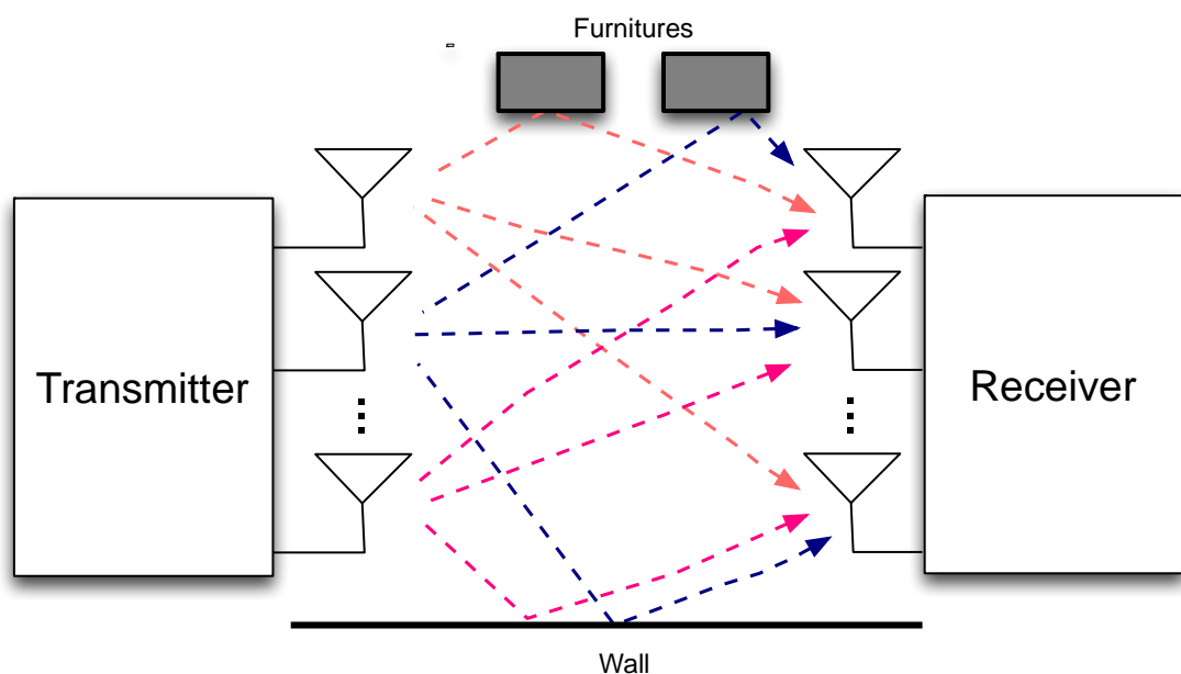
Figure 2.9 MIMO with multipath fading.
