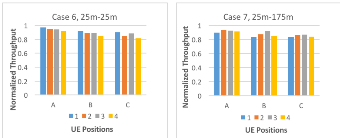
Figure 3.10 Spatial Diversity-supported downlink throughput with different fibre link lengths (a) Case 6, 25m-25m (b) Case 7, 25m-175m
