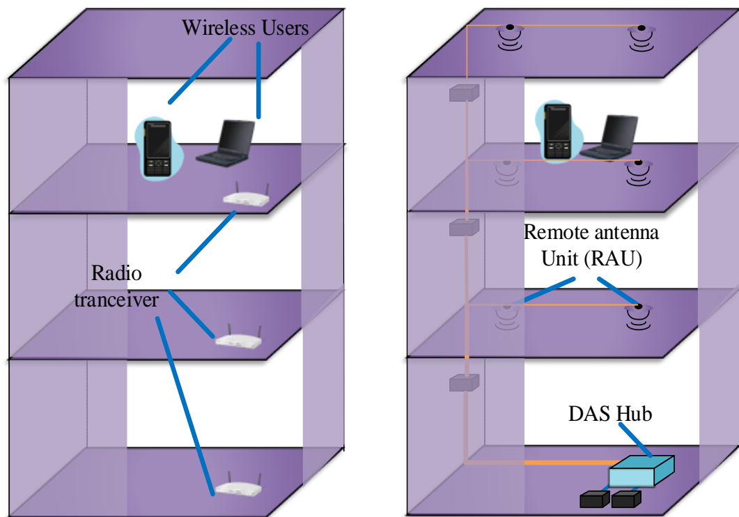
Figure 2.1 (a) Conventional co-located antenna system (CAS) (b) Distributed antenna system (DAS)
