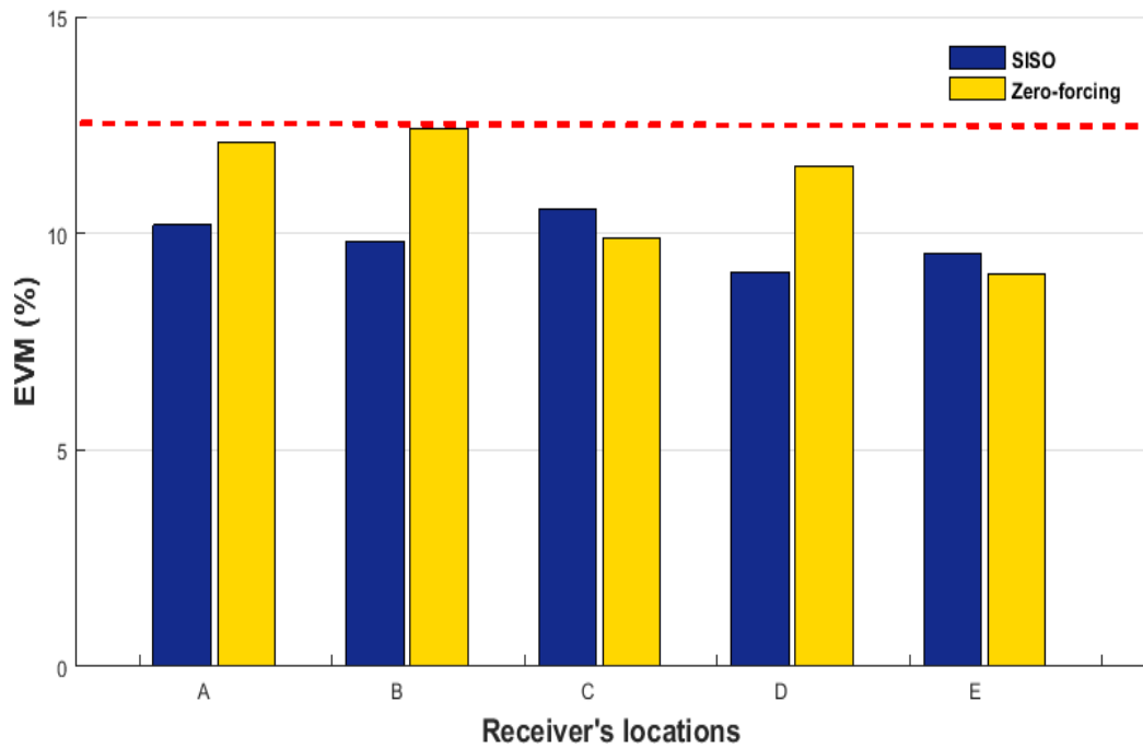
Figure 5.23 EVM result of SISO compared with the emulated 2x2 MIMO for 20cm transmit antenna separation at different receiver's locations using zero-forcing spatial multiplexing algorithm.
