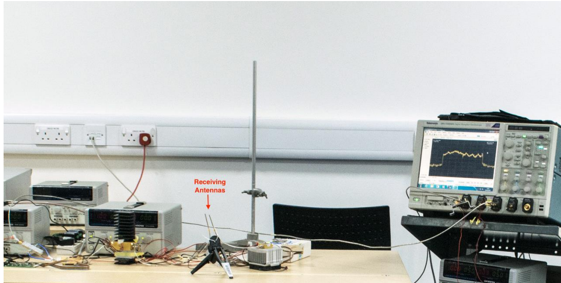
Figure 5.9 Receiving antenna connected to the differential baluns that produces I , \bar{I} signal for the gRSC0016 60GHz receiver circuit and the signal captured at the Oscilloscope for offline processing.
