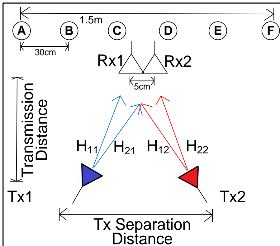
Figure 5.3 Measurement layout of the testing room.
