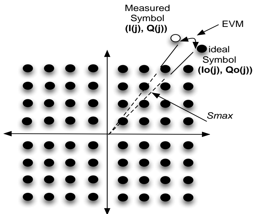
Figure 2.13 Constellation diagram of 64-QAM.
