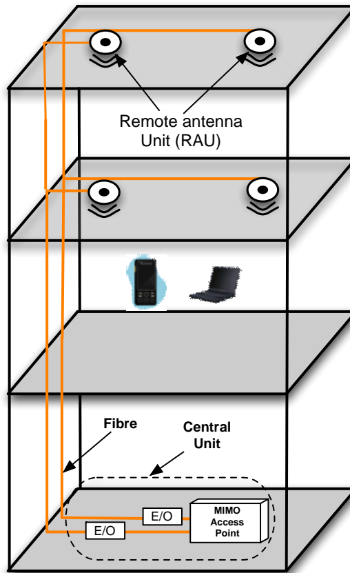
Figure 3.1 2x2 MIMO AP in RoF-DAS
