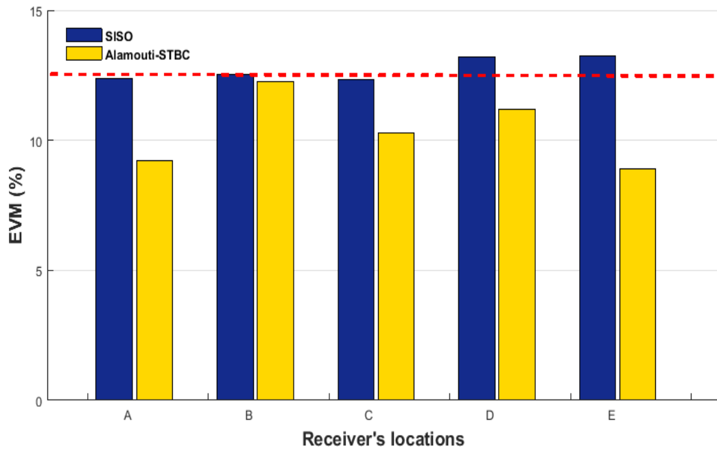
Figure 5.21 EVM result of SISO compared with the emulated 2x2 MIMO for 20cm transmit antenna separation at different receiver’s locations using Alamouti STBC spatial diversity algorithm.
