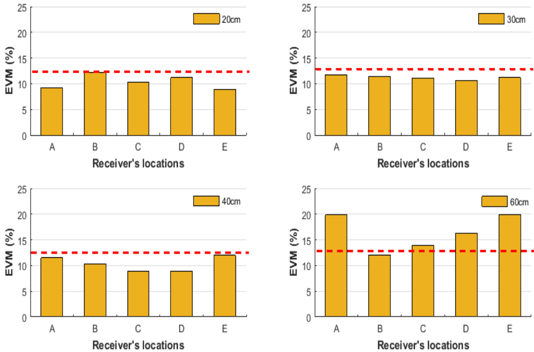
Figure 5.20 EVM result of 60GHz experiment at 20cm, 30cm, 40cm and 60cm transmit antenna separation distances using Alamouti STBC spatial diversity algorithm.
