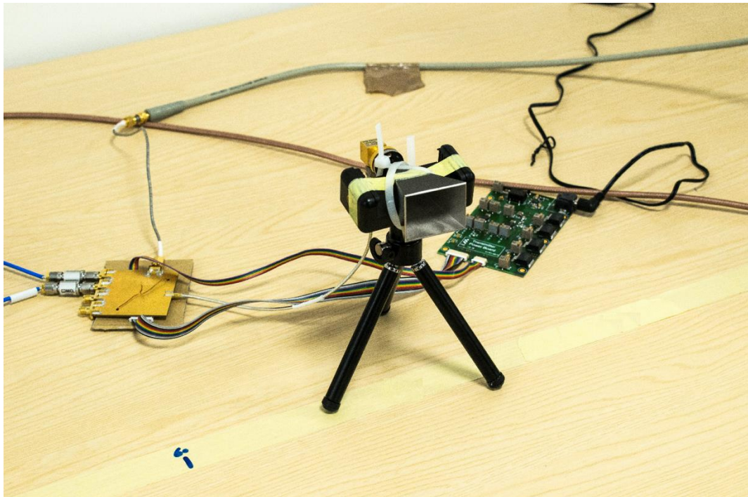
Figure 5.6 IF signal fed into a differential baluns that produces I , \bar{I} , for the gTSC0020 60GHz integrated transmitter circuit and wirelessly transmitted through an horn antenna.
