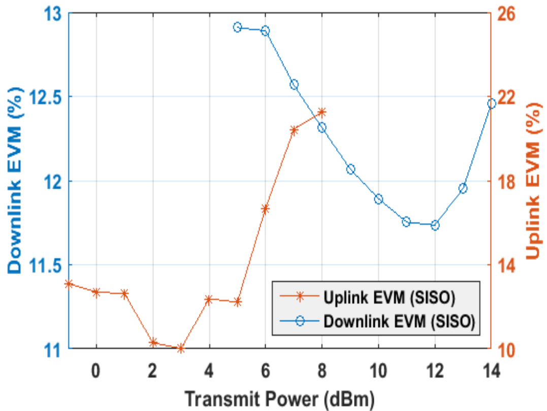
Figure 4.5 EVM of downlink and uplink signal transmitted from the RAU as the transmit power is increased to determine the optimum transmit power for measurement.
