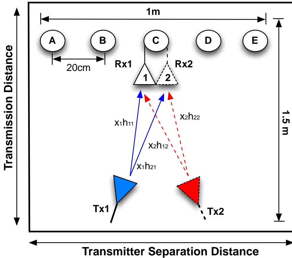
Figure 5.11 Measurement layout of 60GHz experiment
