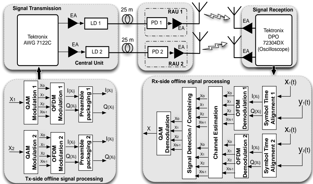
Figure 4.2 The downlink Experimental setup for 2x2 MIMO over Fiber EA= Electric amplifiers PD=Photodetector, LD=Laser diode, RAU=Remote antenna unit
