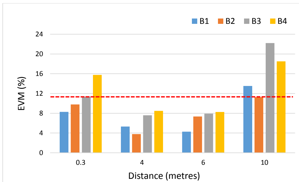
Figure 4.23 EVM of downlink 2x1 STBC Alamouti-MISO measured at inter-RAU distance of 0.3m, 4m, 6m and 10m at different positions A1-A4 (top) and B1-B4 (bottom).
