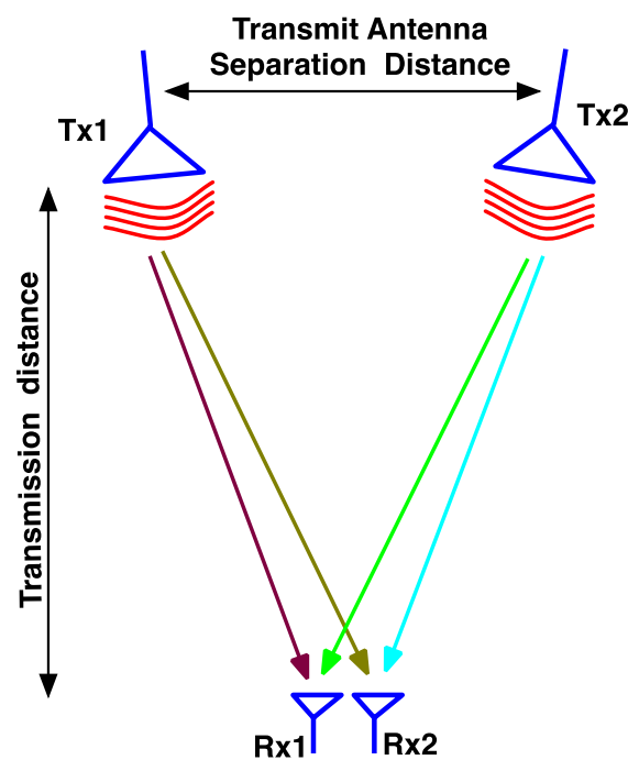
Figure 5.1 MIMO in Line-of-sight (LOS) propagation.
