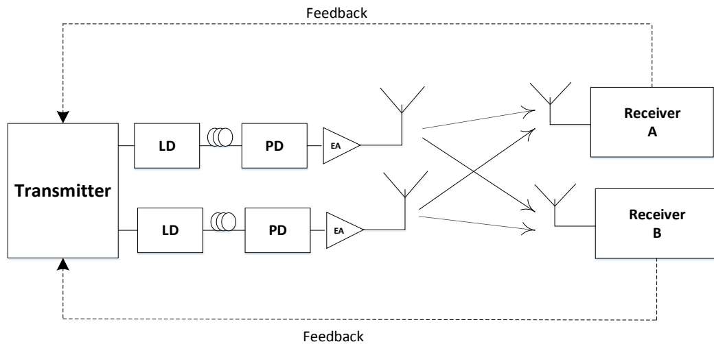
Figure 6.1 An example of the experimental setup of a multi-user pre-coding MIMO in RoF-DAS.
