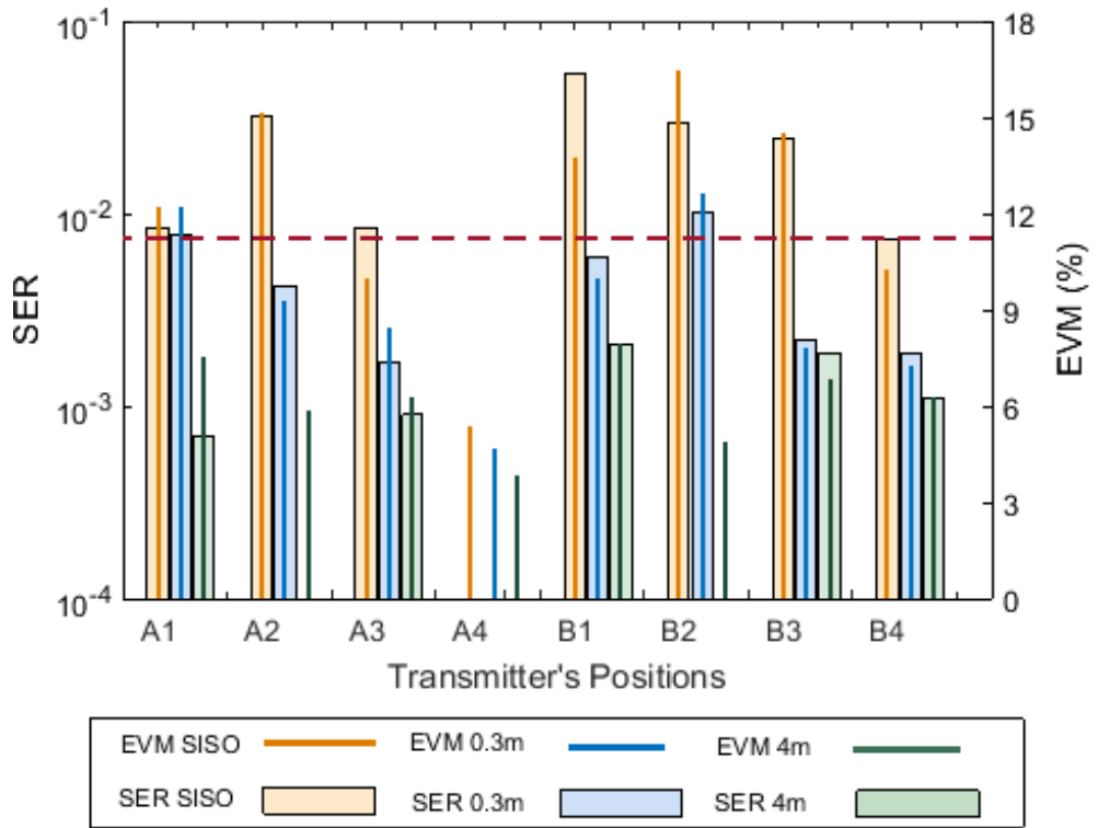
Figure 4.7 SER and EVM of uplink 1x2 EGC-SIMO measured at inter-RAU distance of 0.3m and 4m at different positions compared to SISO .
