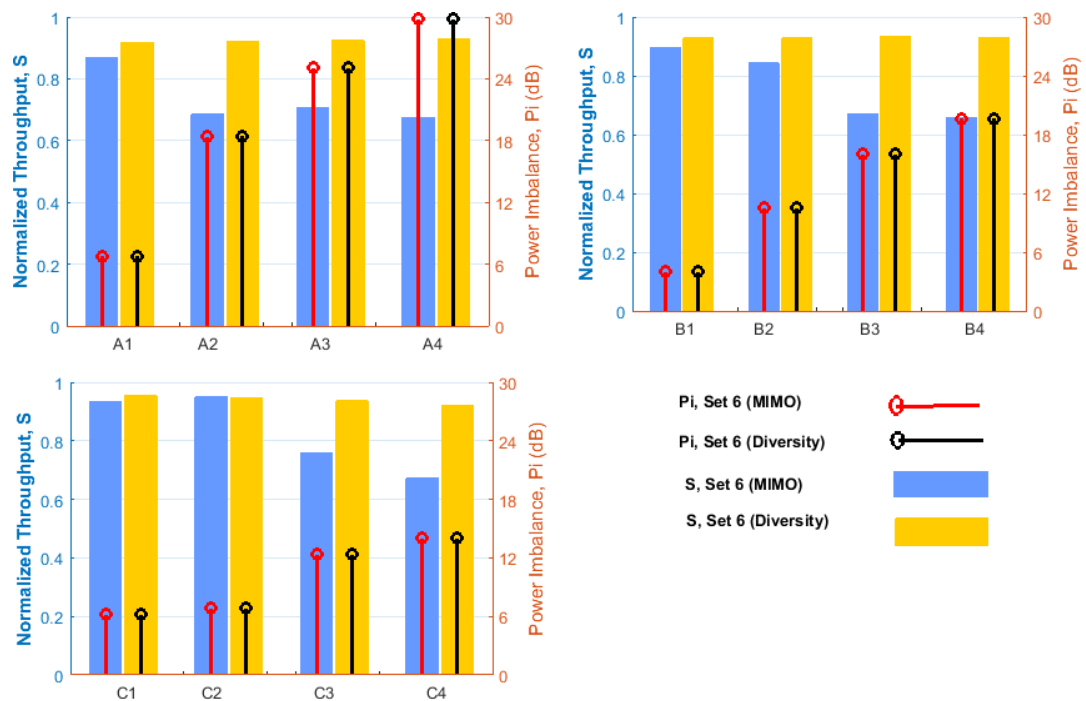
Figure 3.15 Throughput S and power imbalance Pi results of MIMO using set 6 and spatial diversity using set 6.
