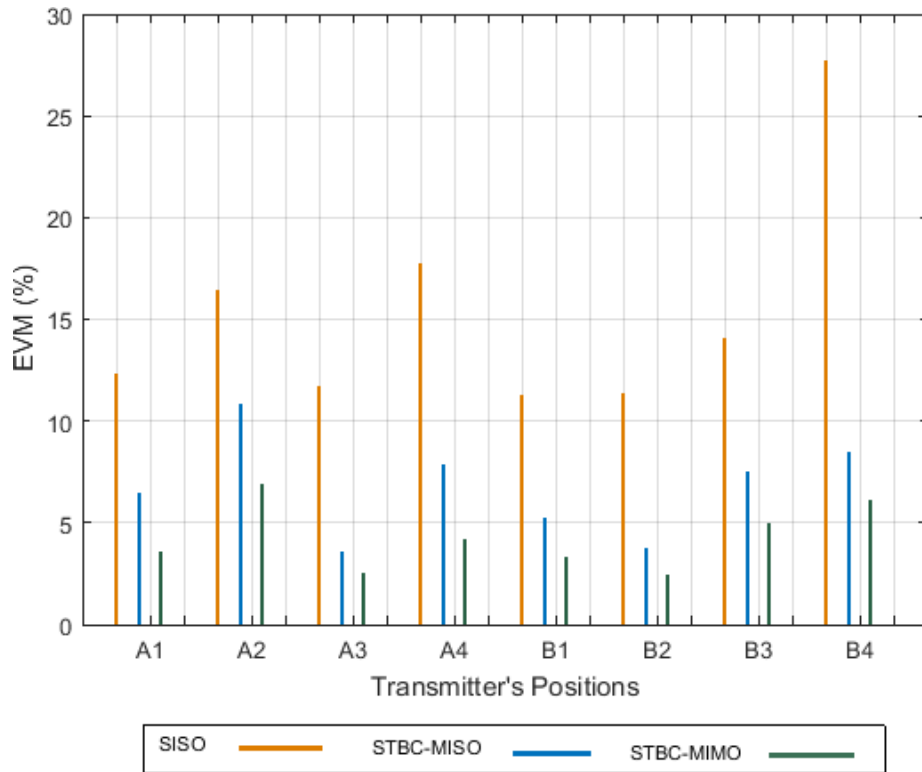
Figure 4.16 EVM of SISO , Alamouti STBC-MISO and Alamouti STBC-MIMO scheme measured at inter-RAU distance 4m at different positions A, B (1-4).
