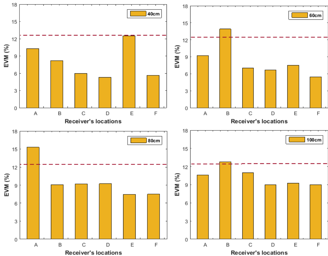
Figure 5.14 EVM result of 2x2 spatial diversity-MIMO at receiver location A to F for 40cm, 60cm, 80cm and 100cm transmit antenna separation distances at 3.5m wireless transmission distance.
