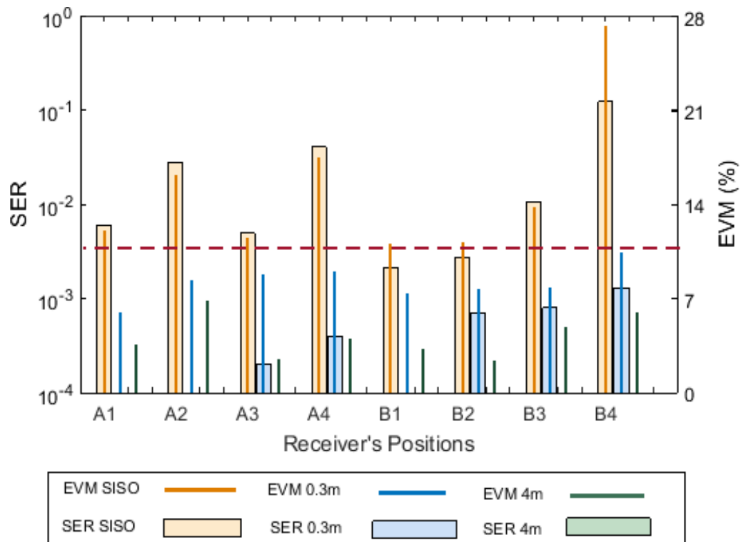
Figure 4.15 SER and EVM of downlink 2x2 Alamouti STBC-MIMO measured at inter-RAU distance of 0.3m and 4m at different positions compared to SISO .
