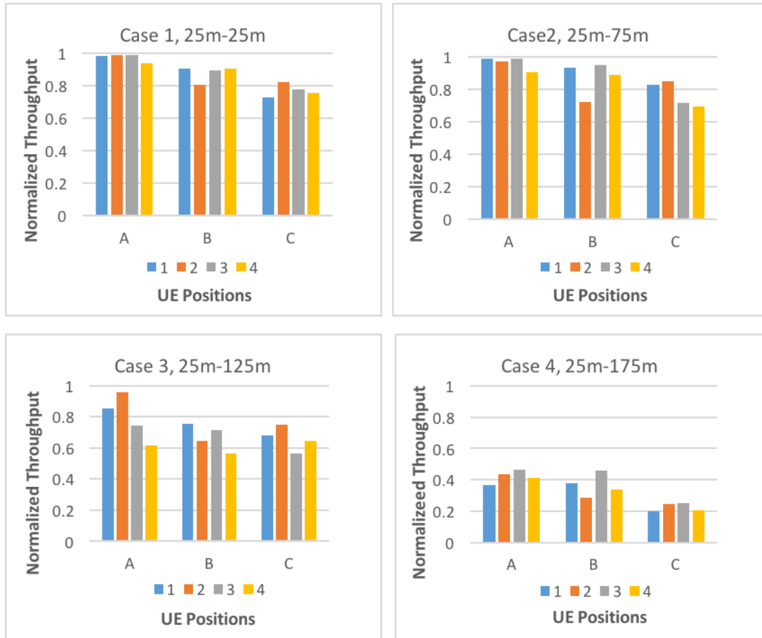
Figure 3.8 MIMO-supported downlink throughput with different fibre links (a) Case 1, 25m-25m (b) Case 2, 25m-75m (c) Case 3, 25m-125m (d) Case 4, 25m-175m.
