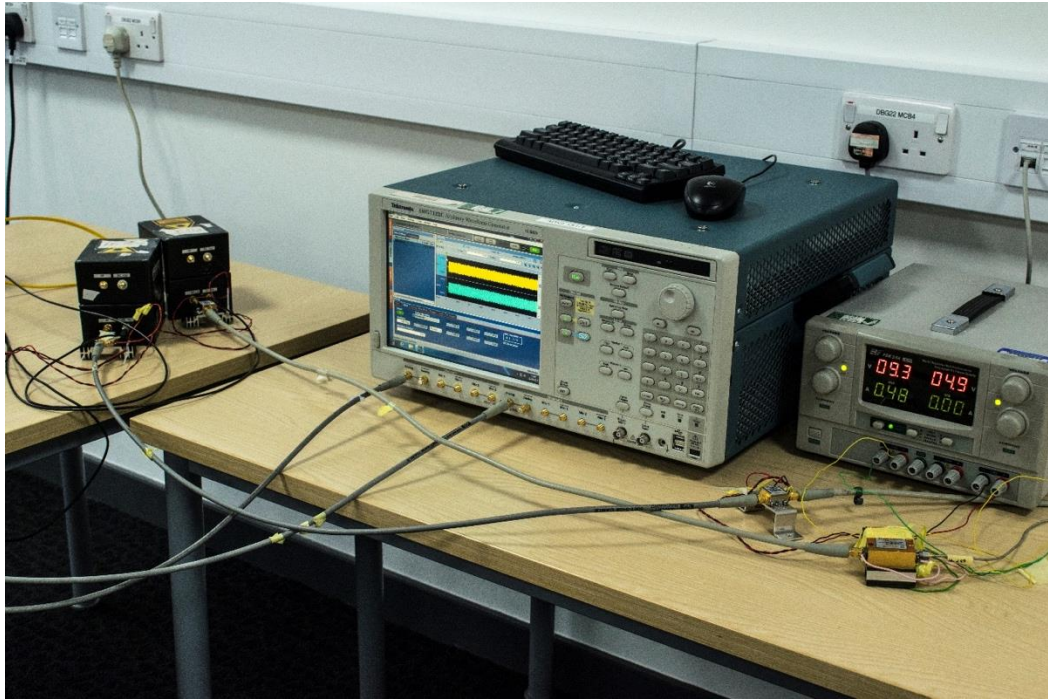
Figure 5.5 Arbitrary Waveform generator (AWG) upconverting baseband signal to an intermediate frequency (IF) and modulating it onto a DFB laser diode.
