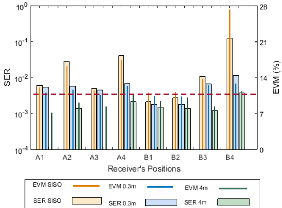
Figure 4.17 SER and EVM of downlink 2x2 DD/MRC-MIMO measured at inter-RAU distance of 0.3m and 4m at different positions compared to SISO .
