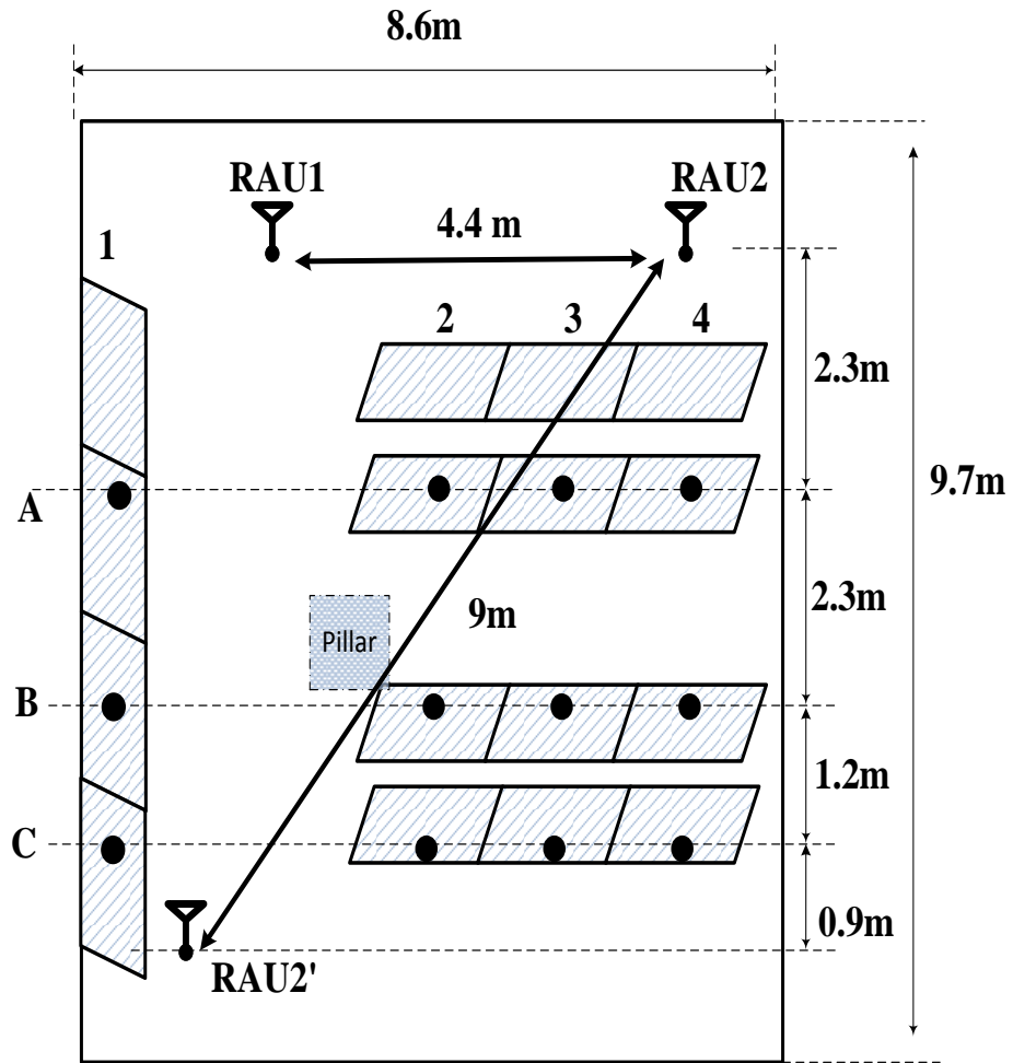
Figure 3.5 Experiment layout. The large black dots are the locations of the mobile devices.
