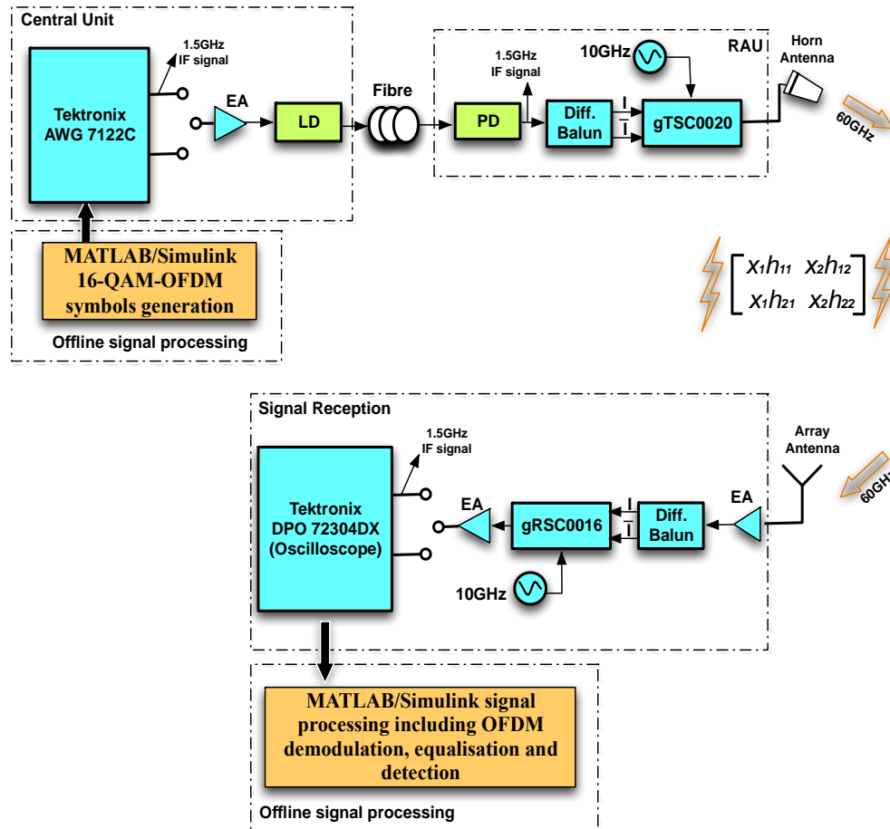
Figure 5.4 Experimental setup for 60GHz Radio-over-Fibre system using integrated transmitter/receiver circuits.
