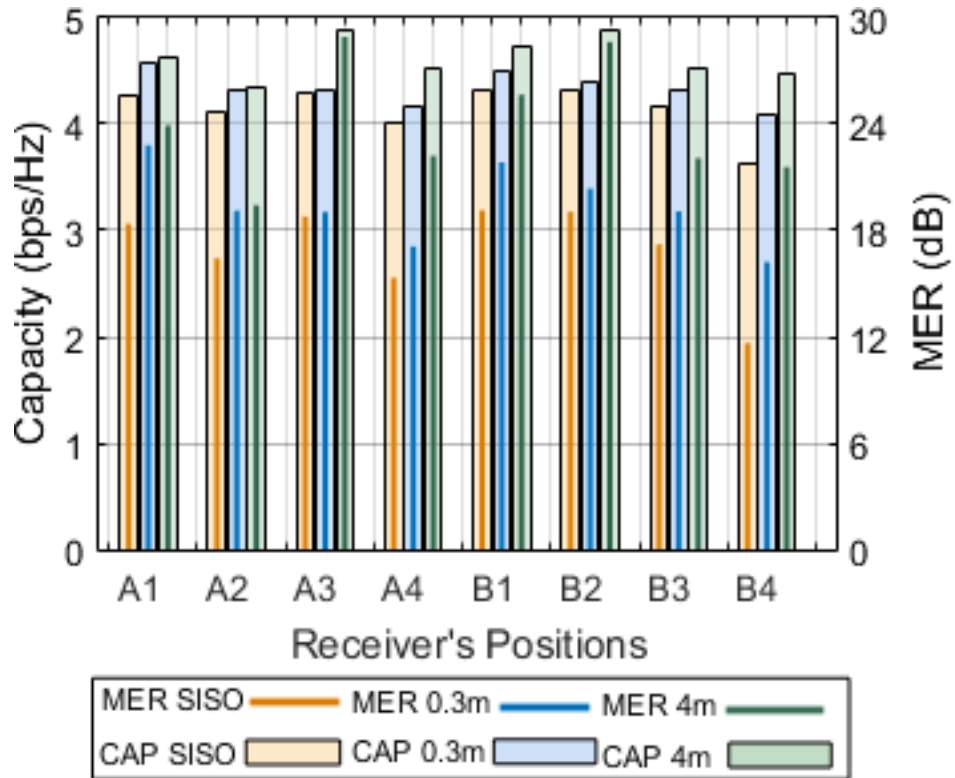
Figure 4.19 Capacity and MER of downlink 2x1 Alamouti STBC-MISO measured at inter-RAU distance of 0.3m and 4m at different positions compared to SISO .
