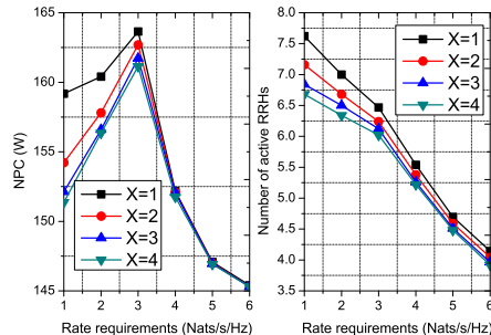
Fig. 15. (a) NPC versus the rate requirements; (b) The corresponding number of active RRHs versus the rate requirements.
