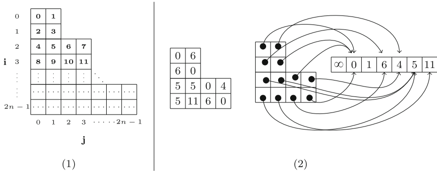
Fig. 16 (1) Representing a DBM as an array; (2) representing a DBM as a CoDBM
