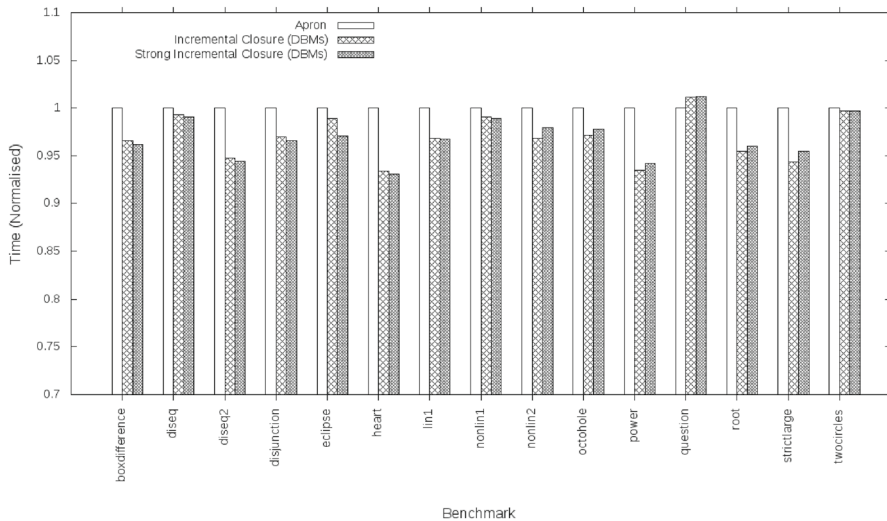
Fig. 19 Normalised timings for the absolute constraint solver (doubles)
