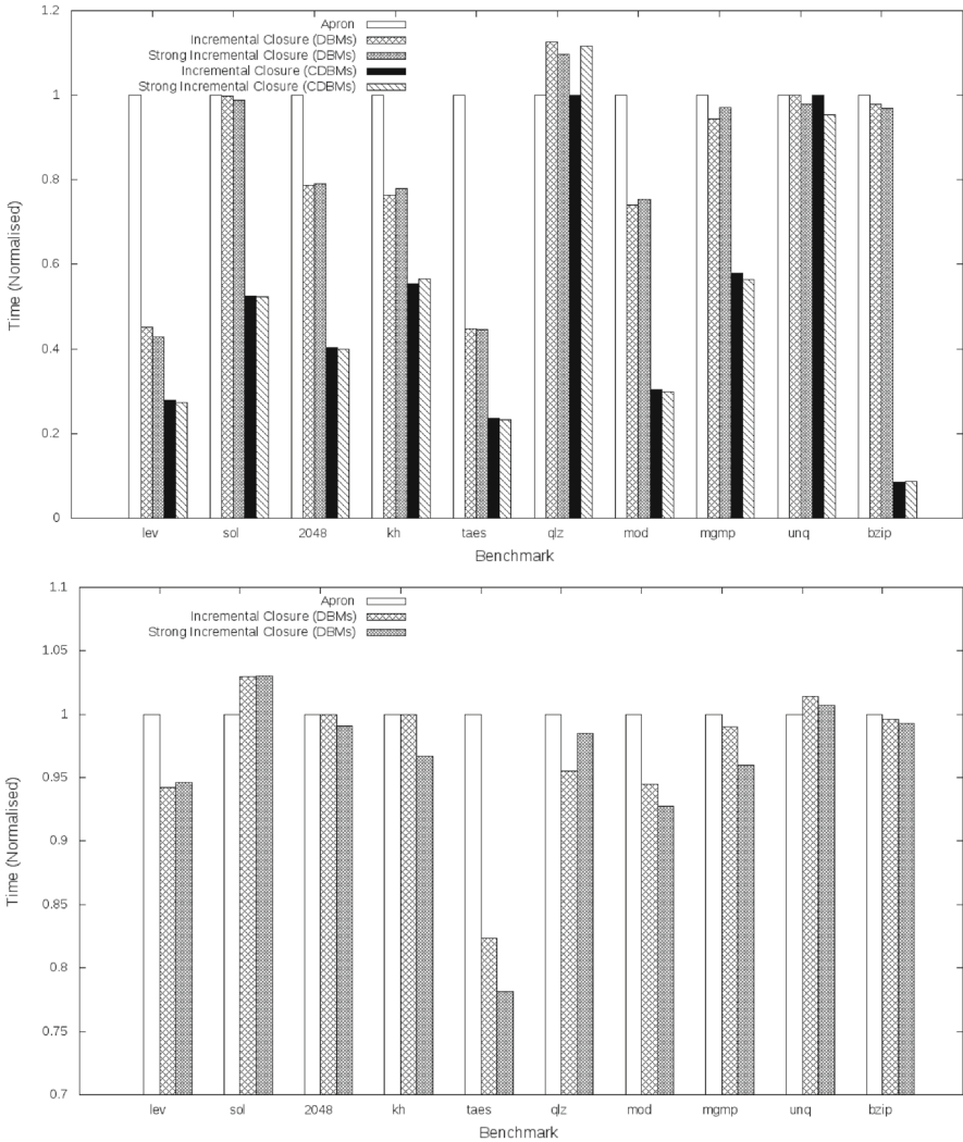
Fig. 18 Normalised timings of Frama-C for rationals (above) and floating point (below)
