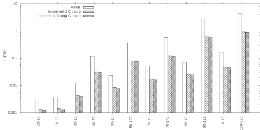
Fig. 17 Micro-benchmark timings for rationals
