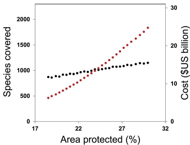
Figure 2. The number of globally threatened vertebrates that reach our adequacy targets (black), and the agricultural opportunity cost of establishing new protected areas (red), as the proportion of global land areas protected increases above 17%.
