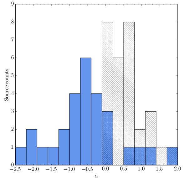
Figure 7. A histogram of all the spectral indices derived for those sources determined to exhibit jet-like characteristics (hatched). The solid blue bars are for the associated lobes. Binning starts at \alpha = -2.5 and bin widths are set at 0.3 due to the sample size.
