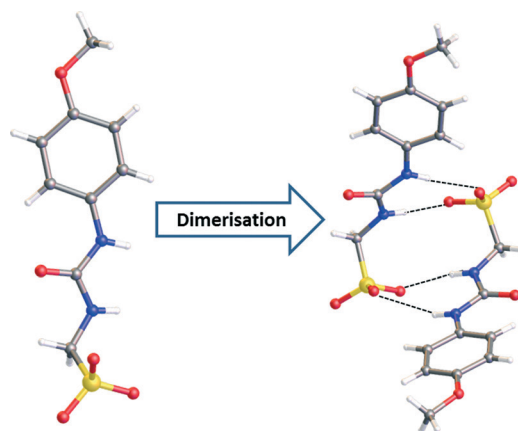
Fig. 4 Ball and stick representation of the hydrogen bonded dimer formed with 1. In this instance the minor component of disorder has been omitted for clarity. Atomic colour scheme: carbon = grey; oxygen = red; nitrogen = blue; sulfur = yellow; hydrogen = white.
