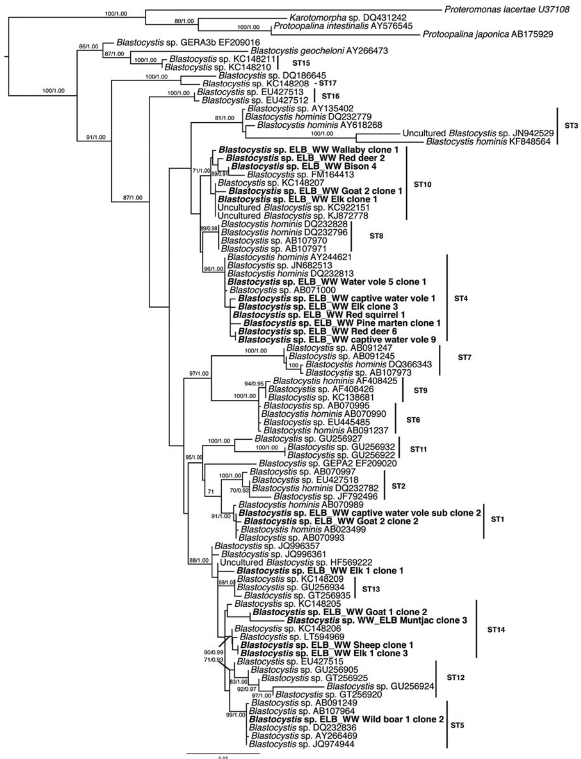
Fig. 1. Maximum likelihood phylogenetic tree inferred from 90 SSUrRNA sequences and 1163 sites. Newly generated sequences are shown in bold. Numerical values on the branches indicate bootstrap percentages and posterior probabilities in this order. Only bootstrap support values greater than 70 are shown. The accession numbers of all newly generated sequences are presented in online Supplementary Table S1.
