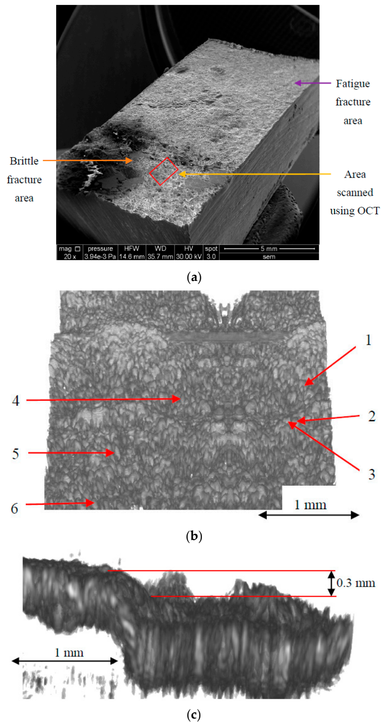
Figure 10. Images of a fracture in a T10NiCr180 stainless steel sample: (a) SEM overview of the entire sample, with the selected area for OCT imaging; (b) OCT image of the selected area, obtained with the improved MS/SS-OCT system—with a 10 \mu\text{m} lateral resolution; (c) OCT image of the step from the fatigue area to the one of the brittle fracture.
