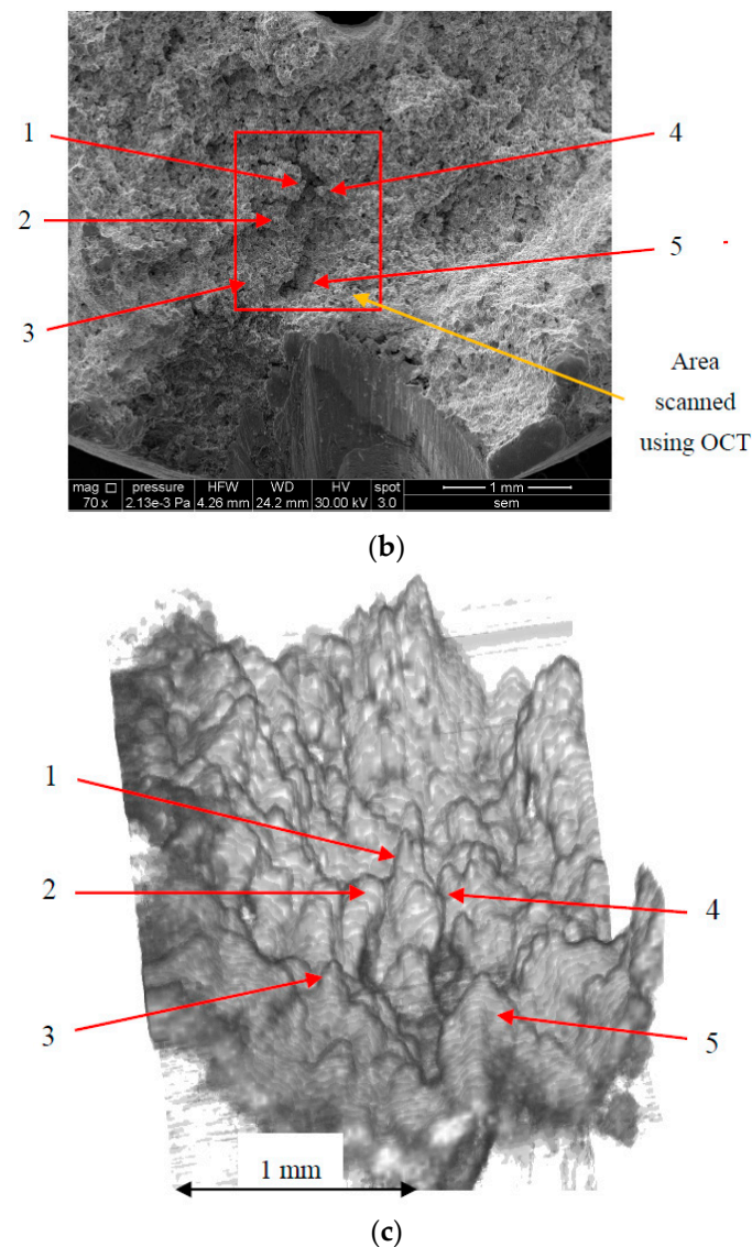
Figure 8. Images of a fracture in a Sn-Sb-Cu antifriction alloy: (a,b) frontal SEM overview of the entire sample, the latter with a zoom to mark the area for OCT imaging; (c) OCT image ( 1 \times 1.5 \text{ mm}^2 ) of the selected area, obtained with the MS/SS-OCT system—with the improved 4 \mu\text{m} transversal resolution.
