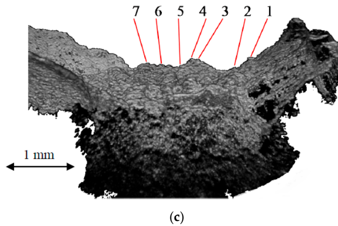
Figure 4. Images of a fracture in OL 44 steel: (a) frontal SEM overview of the entire sample, with an area selected for SEM and OCT imaging; (b) SEM image of the marked area; (c) OCT image of the same area (with a 10 \mu\text{m} transversal resolution), with the same grains as in (b) numbered on the surface—also presented in [36].
