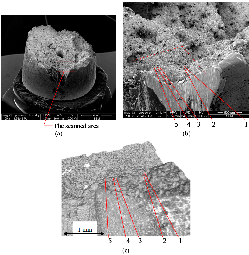
Figure 7. Images of a fracture in a Sn-Sb-Cu antifriction alloy: (a) frontal SEM overview of the entire sample, with a marked area for the OCT investigation; (b) SEM image of the selected area; (c) OCT image of the same area with a 10 µm transversal resolution, with the same grains as in (b) numbered on the surface.
