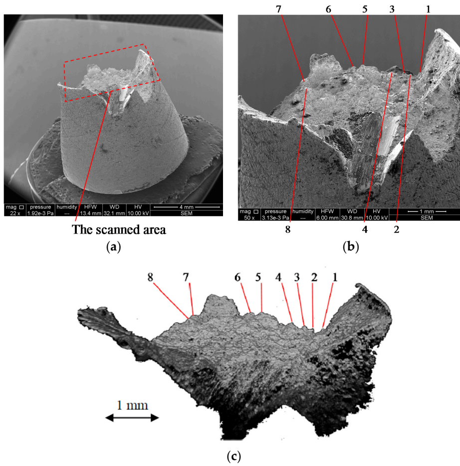
Figure 3. Images of a fracture in OL 37 steel: (a) frontal SEM overview of the entire sample, with an area selected for SEM and OCT imaging; (b) SEM image of the marked area; (c) OCT image of the same area, with a 10 \mu\text{m} transversal resolution, with the same grains as in (b) numbered on the surface.
