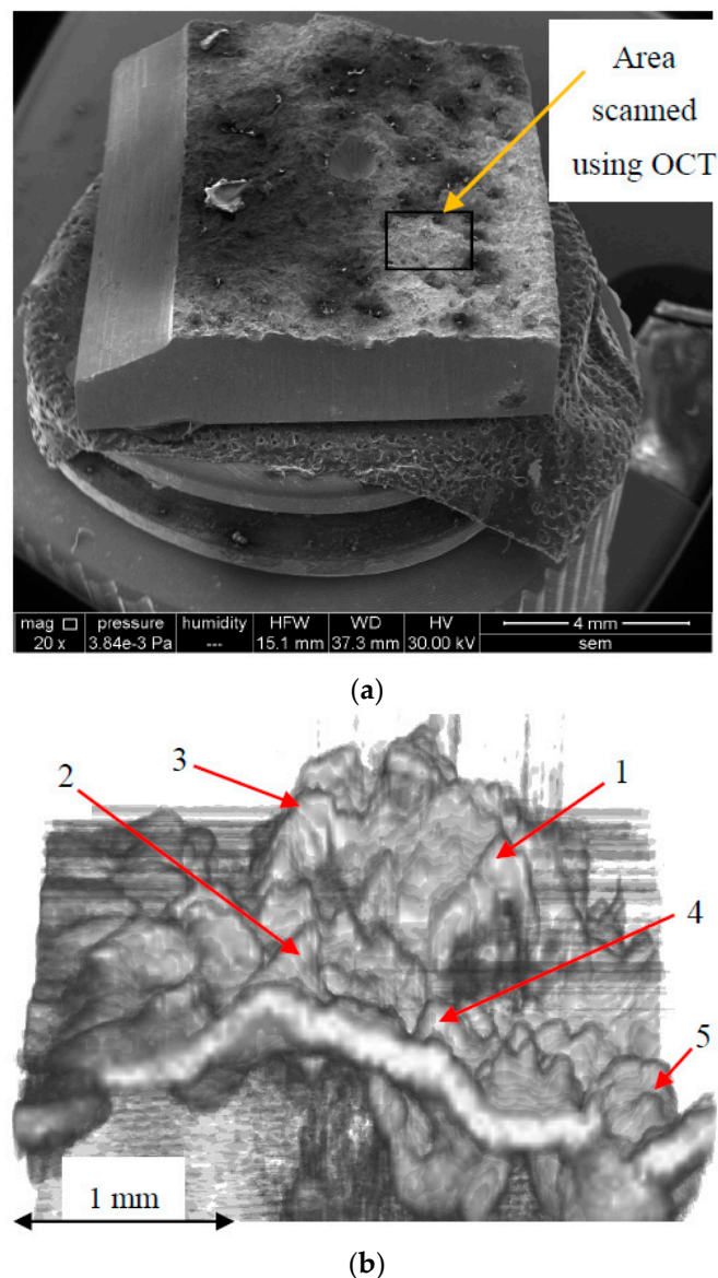
Figure 9. Images of a fracture in an OLC 45 steel: (a) SEM overview of the entire sample, with the marked area for OCT imaging; (b) OCT image of the selected area, obtained with the MS/SS-OCT system with the improved 4 \mu\text{m} transversal resolution, with several grains numbered on the surface.
