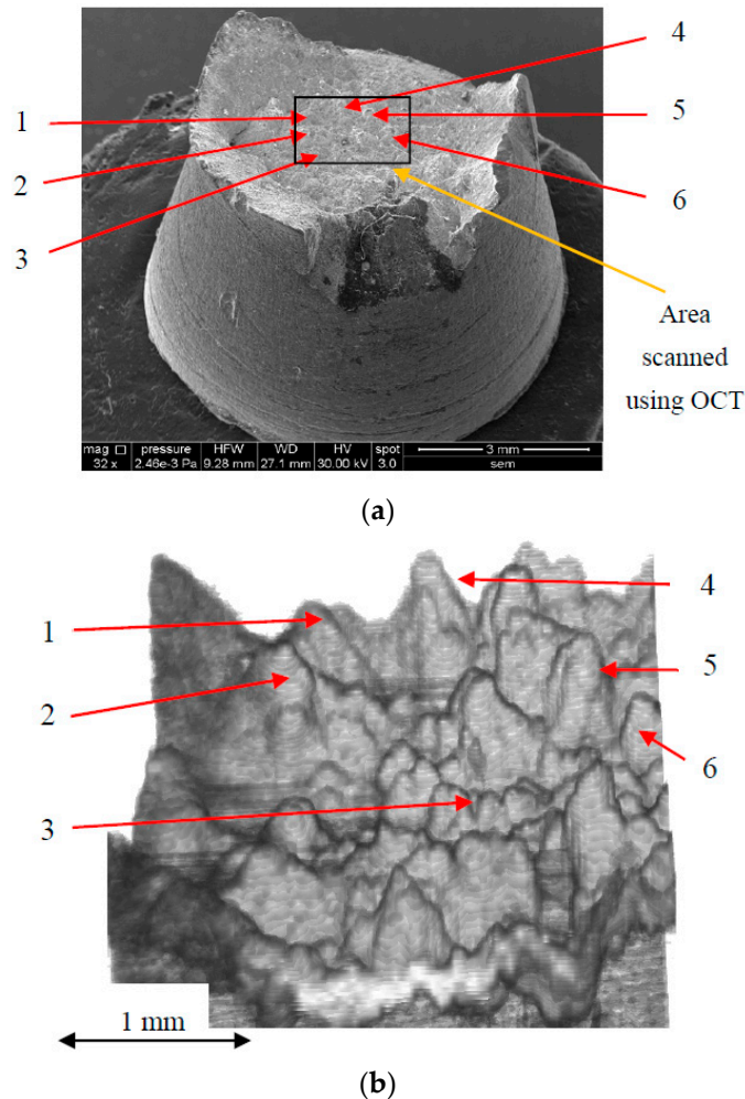
Figure 5. Images of a fracture in OL 44 steel: (a) frontal SEM overview of the entire sample, with a marked area for the OCT investigation; (b) OCT image ( 1.5 \times 1.5 \text{ mm}^2 ) obtained with the novel MS/SS-OCT system—with an improved, 4 \mu\text{m} transversal resolution—with the same grains as in (a) numbered on the surface after a 5\times magnification of the area of interest.
