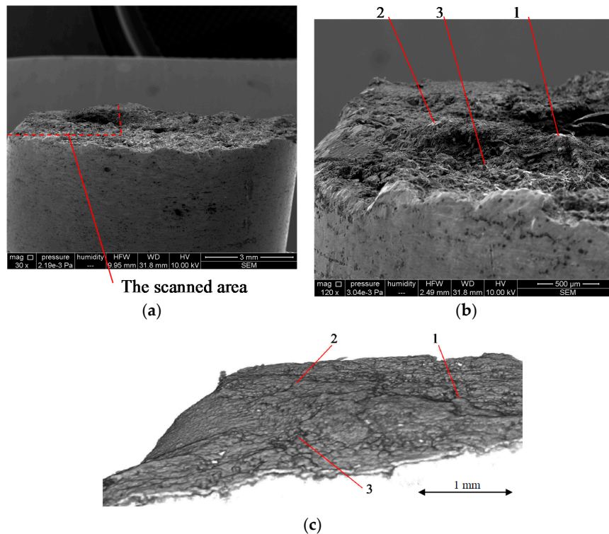
Figure 6. Images of a fracture in a lamellar cast iron EN-GJL 250: (a) frontal SEM overview of the entire sample, with a marked area for the OCT investigation; (b) SEM image of the selected area shown in (a); (c) OCT image of the same area with a 10 \mu\text{m} transversal resolution, with the same grains as in (b) numbered on the surface.
