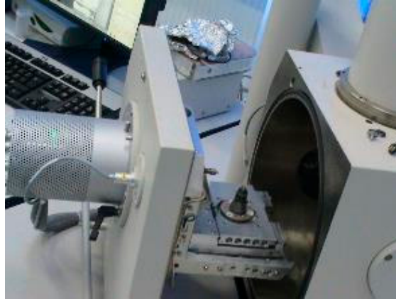
Figure 2. FEI Quanta 250 Scanning Electron Microscope (SEM) utilized in the investigations, with a metallic sample positioned in its holder.
