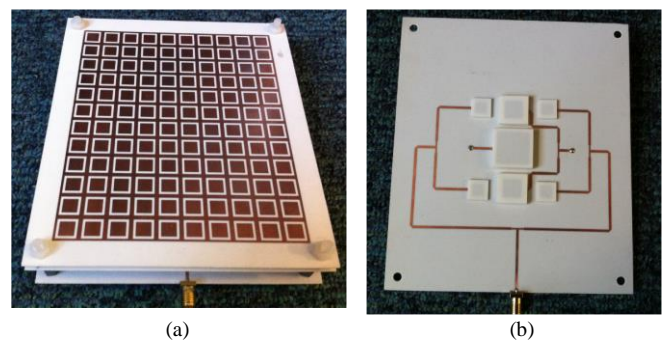
Fig. 12 The prototype of the proposed antenna: (a) the whole antenna; (b) the feed antenna
