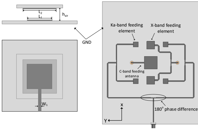
Fig. 9 The configuration of the feed unit and feed arrays
