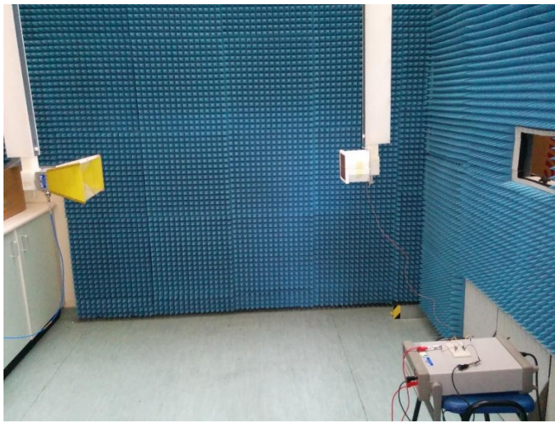
Fig. 2 The experimentation apparatus
