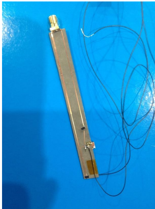
Fig. 34 The matching network chip consisting of microstrip phase shifters and the low-pass filter
