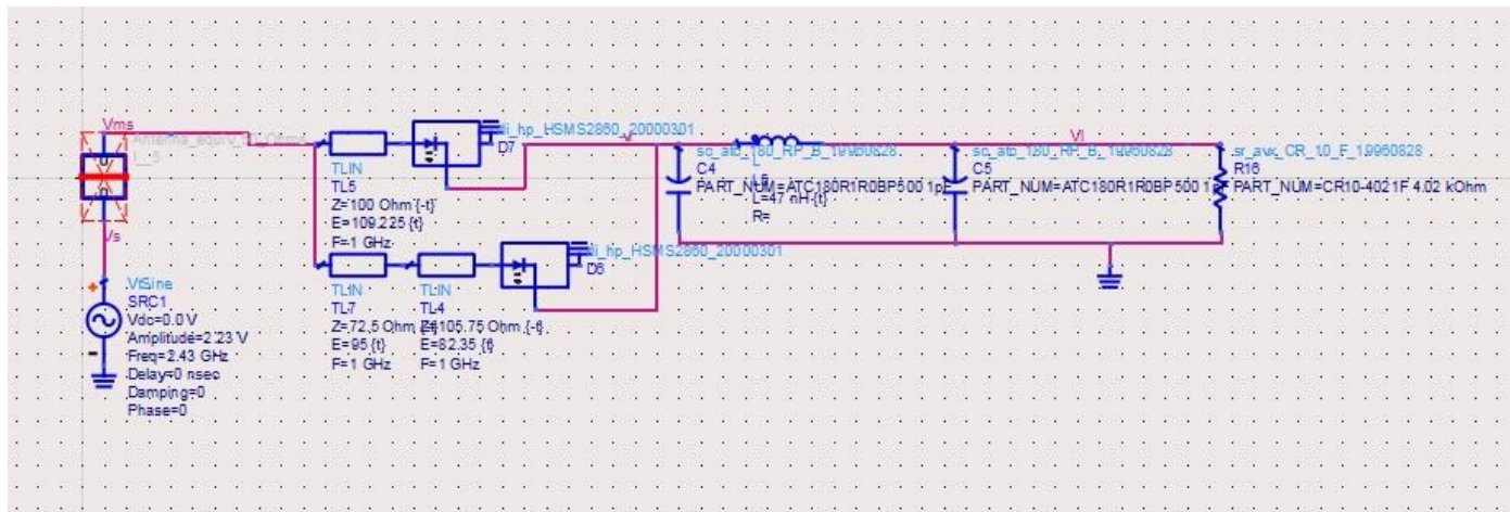
Fig.11 Schematic with disabled antenna component and tuned microstrips
