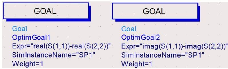
Fig. 10 The goals for the real and the imaginary parts in ADS
