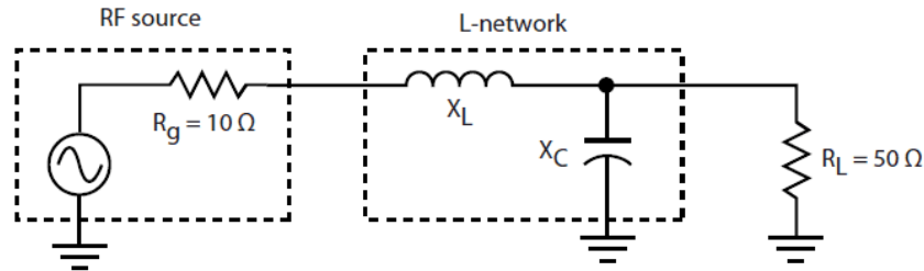
Fig. 10 Circuit diagram of a matching circuit designed [14]
