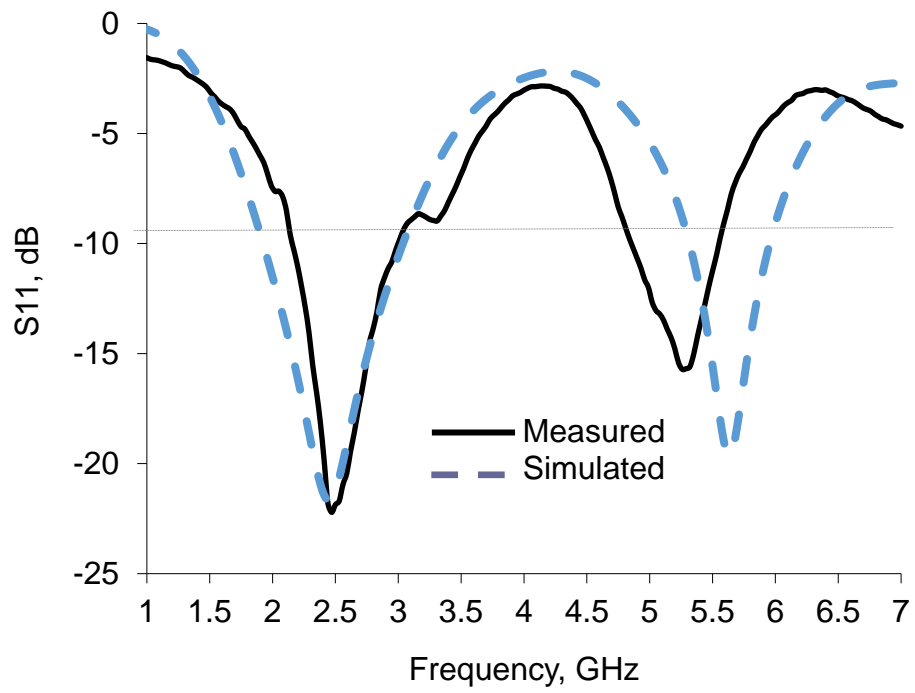
Fig. 10 Simulation vs result graph for the slot antenna with an SMA connector
