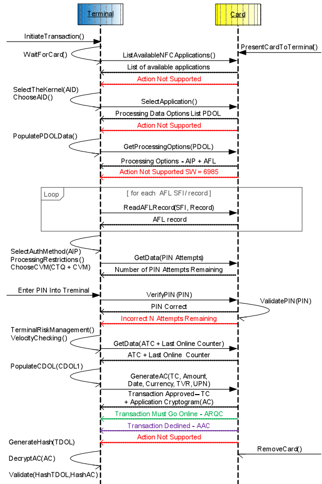
Figure 6. Chip & PIN Transaction Protocol
