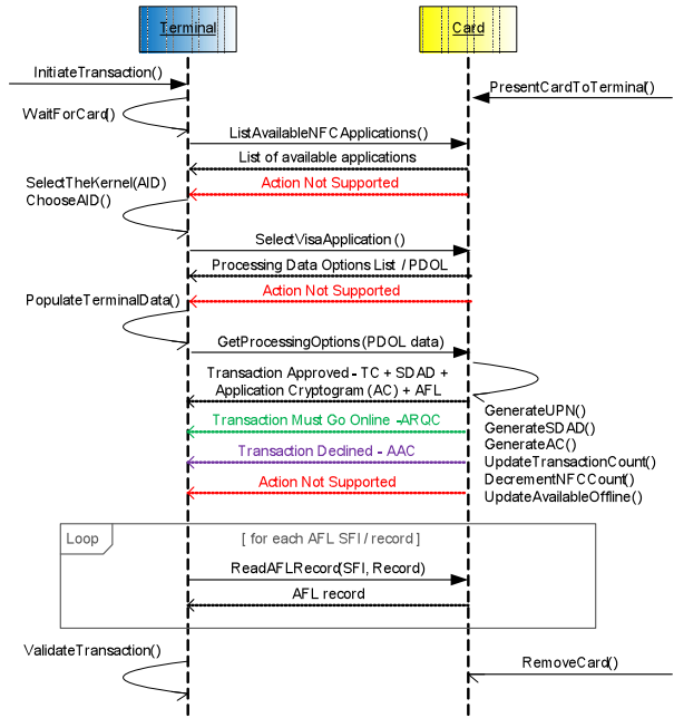
Figure 3. Visa fDDA Protocol Sequence
