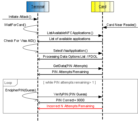
Figure 1. Visa fDDA Transaction Protocol
