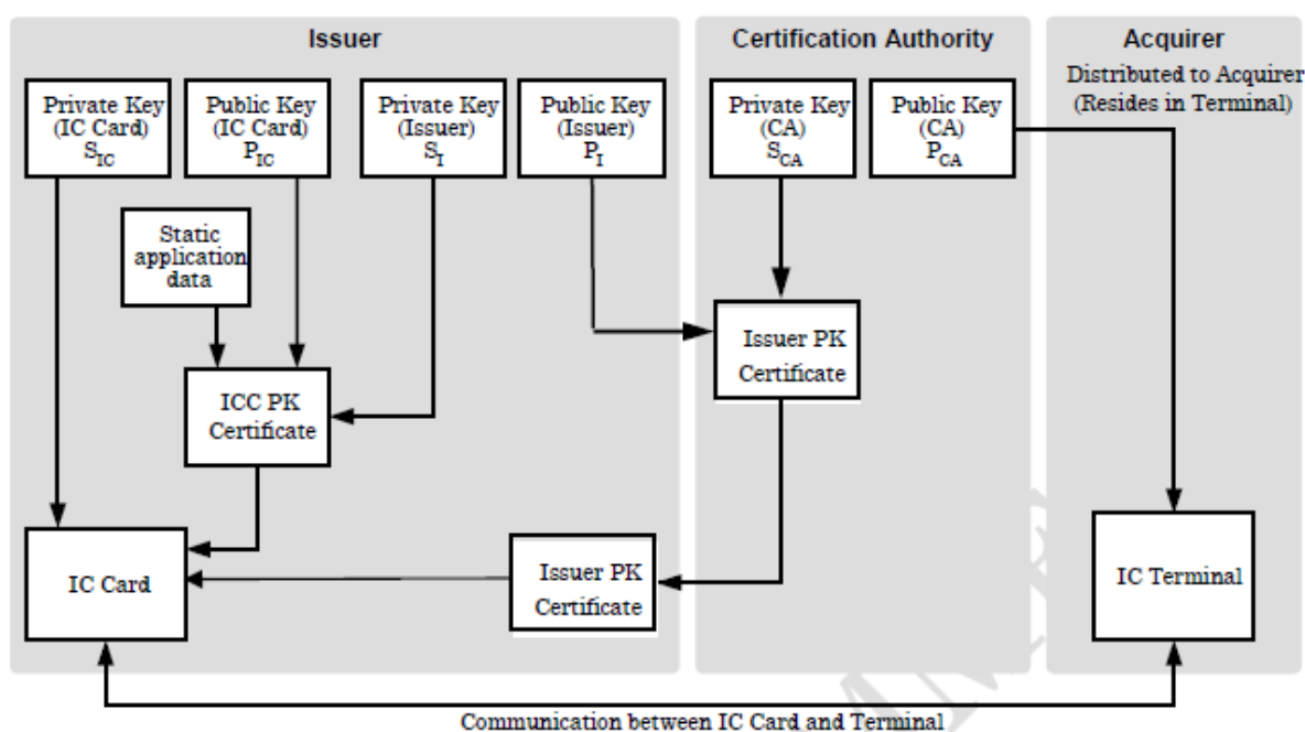
Figure 1 – EMV Public Key Infrastructure (source: [1] page 52)
