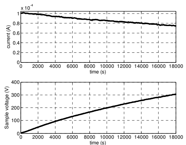
Fig. 2. Electrical data
