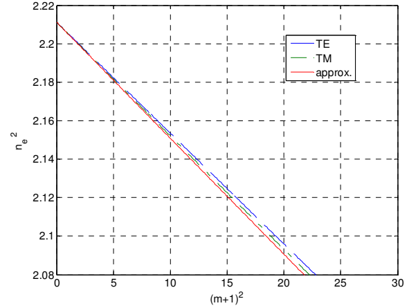
Fig. 6. Plot based on calculation comparing approximation (solid) with exact solution of eqn. (2) for TE and TM modes. d=3.5\mu\text{m} , n_{\text{poled}}=1.487 , (colour on-line).
