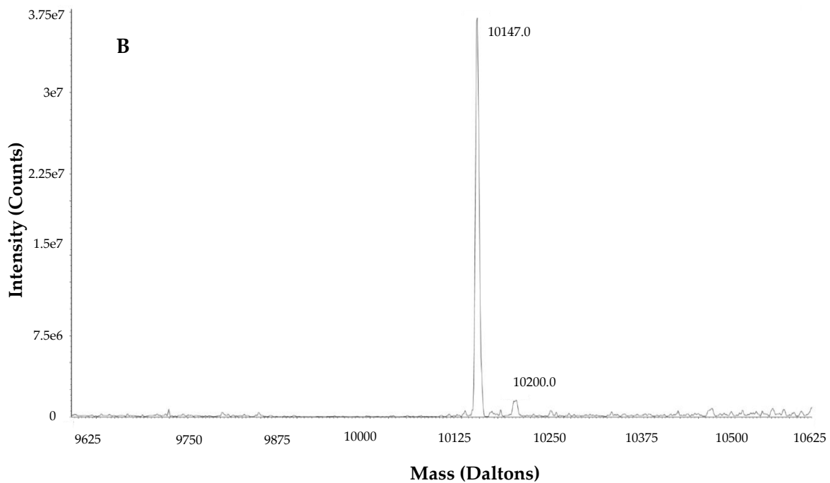
Figure 2.23 Mass spectrometry data for GB1 (A) and GB1- \Delta -somatostatin (B)
