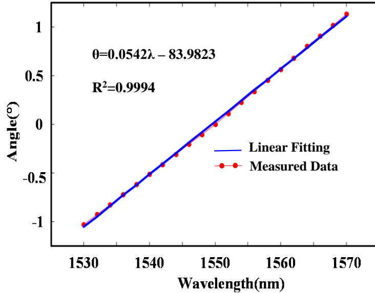
Figure 2. Measured diffraction angle as a function of illuminating wavelength for the fabricated 45^\circ TFG (red-dotted line). Linear fitting result is also shown (blue line) to estimate the angular dispersion.
