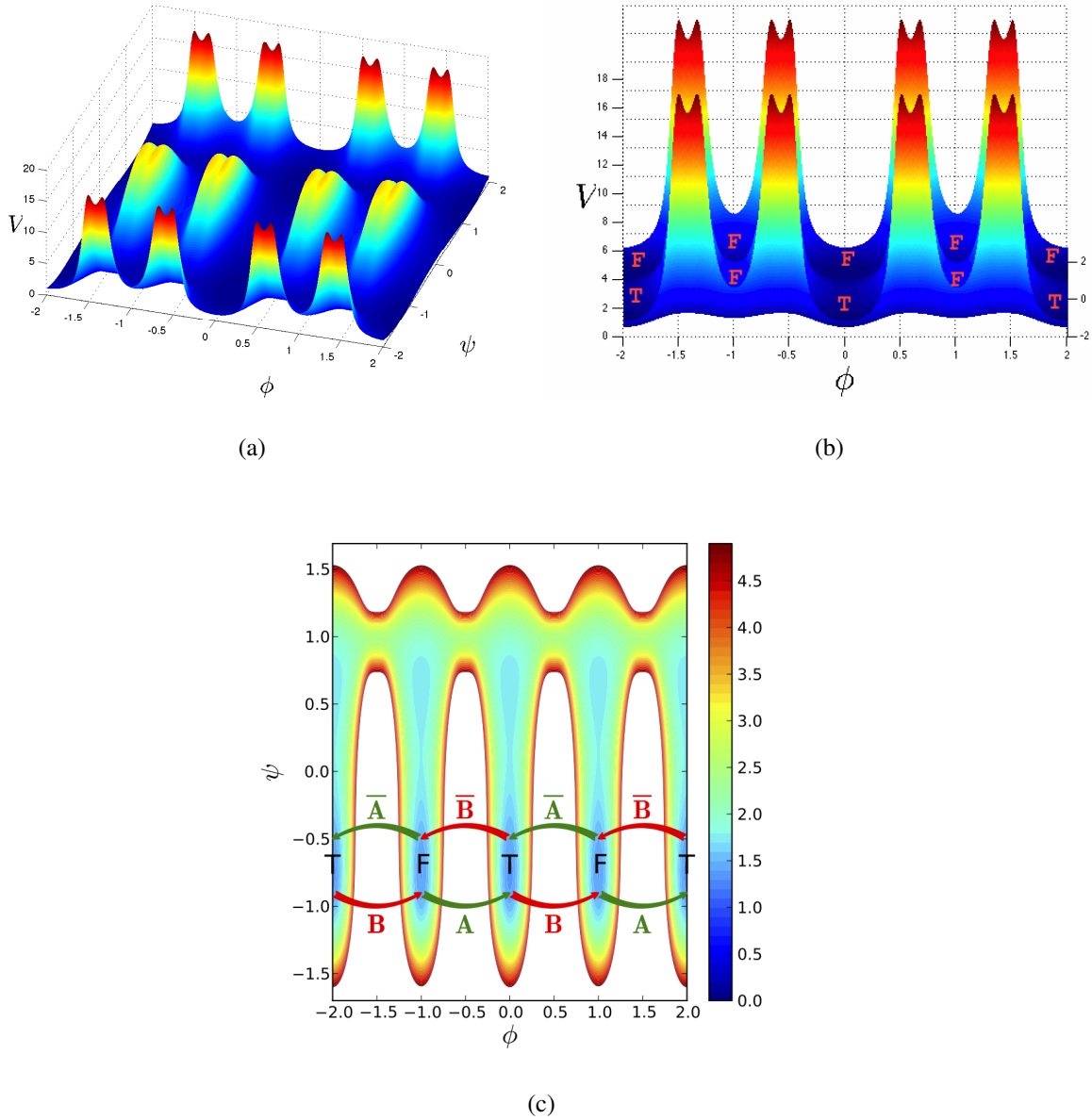
FIG. 1. (a), (b) Surface plots for two different viewing angles and (c) contour plot of the full scalar potential (2) for the parameter choice (6), but with \gamma set to 0.1 for illustrative purposes. Here, the true (T) vacua correspond to \{\psi = -0.7593, \phi = 2k\} , while false vacua (F) occur at \{\psi = -0.7552, \phi = 2k + 1\} . The white regions in the contour plot indicate the insurmountable energy barriers separating true and false vacua. The green and red arrows illustrate the kinks we call of type A and B, respectively. Note that the vacua at \{\psi = 0.6396, \phi = 2k\} and \{\psi = 0.6463, \phi = 2k + 1\} (see (b)) are all raised in energy and hence they are false vacua.
