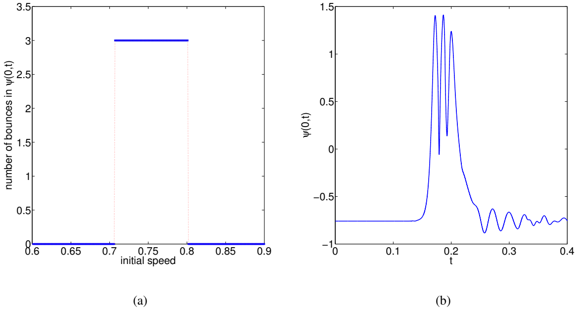
FIG. 5. We display for a AB collision: (a) Number of bounces vs initial velocity. Here, the bounce number measures the number of times the shepherd field \psi oscillates at the origin before the kinks separate. (b) Shepherd field \psi(0, t) at the center-of-mass versus time t for the initial velocity v = 0.750 . The three-bounce collision is clearly visible. For reasons of clarity, time is divided by 100.
