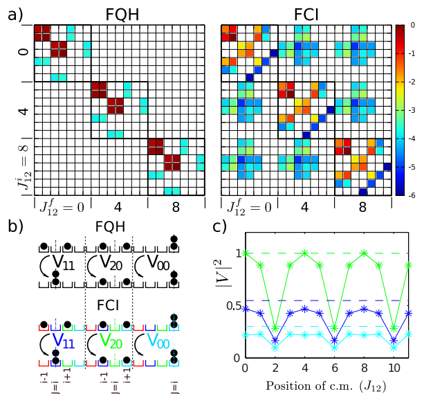
FIG. 2. (a) Magnitudes of matrix elements for the two-body delta interaction between pairs of particles with incoming (outgoing) momenta J_{12}^{(f)} = [(J_1 + J_2) \pmod{N_{\text{cell}}}] in a finite size geometry for the FQHE on the torus with N_\phi = 12 (left) and for the FCI in the lowest band of the Haldane model for a 3 \times 4 lattice (right). (b) Schematic showing some short range interactions, including a ‘squeezing’ process V_{11} as well as two diagonal interaction terms V_{20}, V_{00} . Panel (c) shows how the magnitude of these processes depends on the centre of mass position for the FCI (solid) as compared to FQH (dashed).
