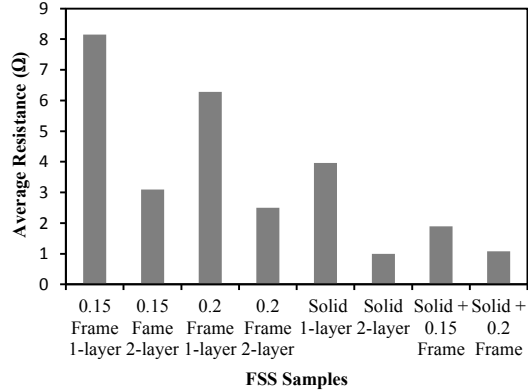
(b) Comparison of resistance values
