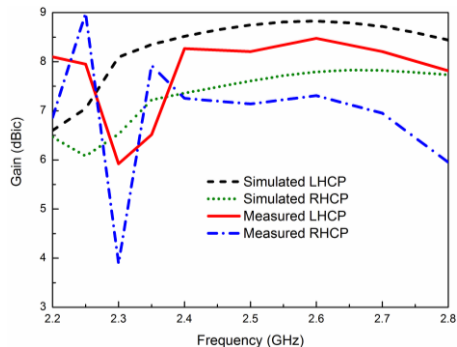
Fig. 8. Simulated and measurement gain under LHCP and RHCP states.
