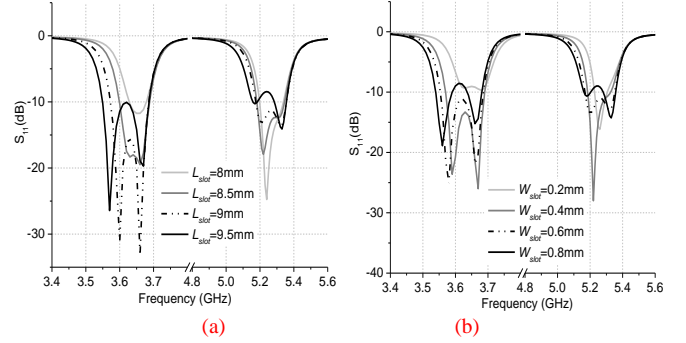
Fig. 3. The variation of bandwidth with different: (a) L_{slot} , (b)
