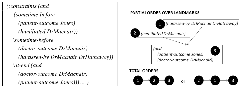
Figure 3 Example Landmarks: the left-hand side contains a selection of landmark facts represented using the PDDL3 modal operators sometime-before and at-end ; on the right-hand side the order specified over the landmarks is represented graphically. The ordered landmarks are used in a decomposition-based planning approach to narrative generation: first, if the landmarks are partially ordered they are linearised to form a total order (the figure shows the consistent total orders, one of which is non-deterministically selected by the system); then each landmark in turn is used as a sub-goal and the narrative is built up incrementally from the sequence of sub-narratives (see text for more detail).
