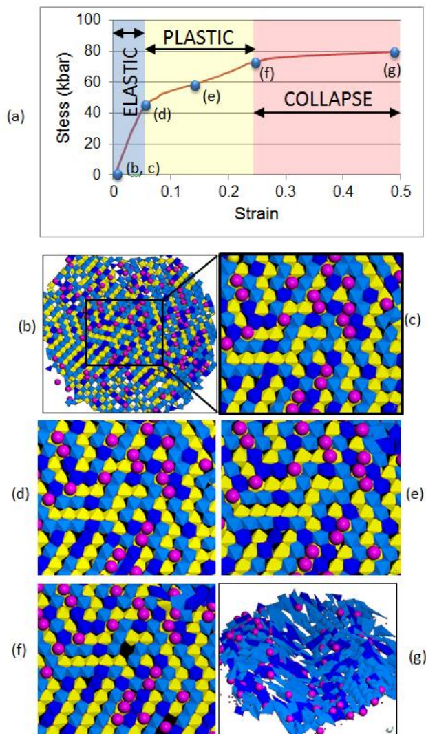
Figure 3 (a) Calculated compressive stress-strain curve for \text{Li}_{0.24}\text{MnO}_2 . (b)-(g) slices cut through the mesoporous Li-MnO 2 showing the retention of structural integrity of the 1D tunnels within the walls of the mesoporous material under compression. Images (b-g) correspond to the stress-strain curve (a). (b-d) elastic deformation, (d-f) plastic deformation, (g) structural collapse. \text{Mn}^{4+} is coloured light blue, \text{Mn}^{3+} is dark blue and Li is pink; manganese surrounded by six oxygen species are represented by polyhedra. The polyhedra coloured yellow correspond to the atomic plane below the blue polyhedra to show more clearly the 1D tunnels and twinning of the \text{MnO}_2 host.
