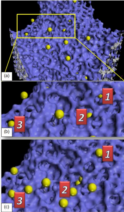
Figure 10 (a) Segment of the surface of a pore within the mesoporous \text{MnO}_2 shown part way through the MD simulation after a number of Li ions have deintercalated out of the \text{MnO}_2 . An enlarged segment of (a) is shown in (b). (c) is the same as (b) but after a few more cycles of MD simulation showing Li that has moved from just inside the surface (b), to just outside the surface (c). Labels 1,2 and 3 help identify the particular Li ion that deintercalates. Li is coloured yellow, mesoporous \text{MnO}_2 is shown using surface rendering.
