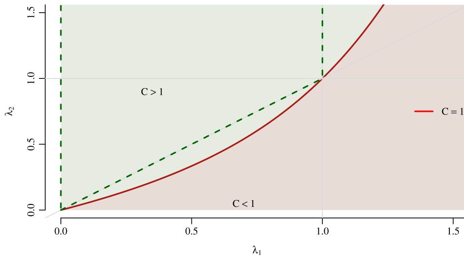
Fig. 3. Curve demarcating the regions where loss coverage ratio is greater than and less than 1 when (\mu_1, \mu_2) = (0.01, 0.04) and (\alpha_1, \alpha_2) = (0.8, 0.2) .
