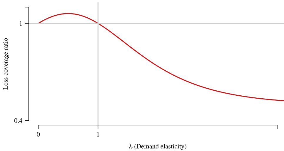
Fig. 2. Loss coverage ratio as a function of demand elasticity for iso-elastic demand.
