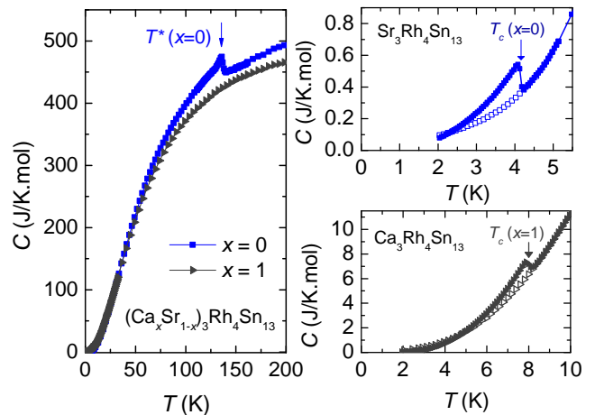
FIG. 2. (Color online) (Left) The specific heat of \text{Sr}_3\text{Rh}_4\text{Sn}_{13} ( x = 0 ) and \text{Ca}_3\text{Rh}_4\text{Sn}_{13} ( x = 1 ) as a function of temperature at zero external magnetic field (closed symbols). T^* indicates the temperature at which a structural transition takes place. (Right) A closeup of the specific heat at low temperatures. The midpoint of the jump defines T_c , which can be suppressed by applying external magnetic field (open symbols).
