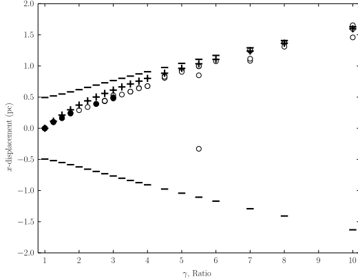
Figure 11. The x displacement of condensed core in G1200 series with an inclination of \varphi = 45^\circ for varied \gamma . The short ‘-’ indicates x_{\max} , ‘+’ x_{\min} , ‘o’ for the cores with 10^6 \leq n_{\text{peak}} \leq 10^{12} \text{ cm}^{-3} , and ‘•’ for the extremely high density cores with n_{\text{peak}} > 10^{12} \text{ cm}^{-3} .
