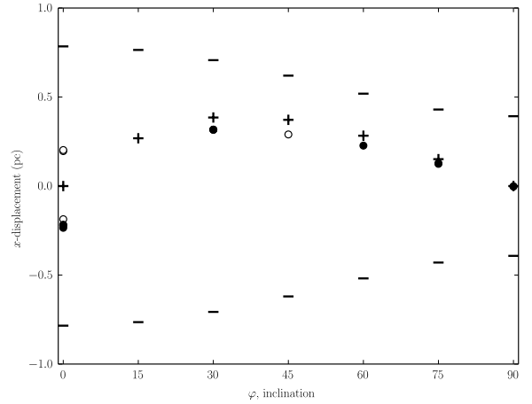
Figure 7. The x displacement of the cores formed in G1200(5) with different initial inclination angles. The short ‘-’ indicates x_{\max} , ‘+’ x_p , ‘o’ for the cores with 10^8 \leq n_{\text{peak}} \leq 10^{12} \text{ cm}^{-3} , and ‘•’ for the extremely high density cores with n_{\text{peak}} > 10^{12} \text{ cm}^{-3} .
