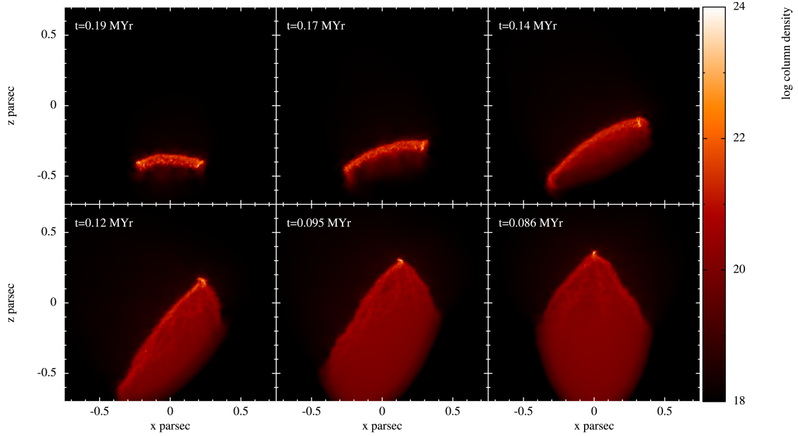
Figure 6. The final snapshot of the column density from six simulations of G1200(5) with different initial inclination angles; left to right then up to bottom are per: 0, 15, 30, 60, 75, 90 °.
