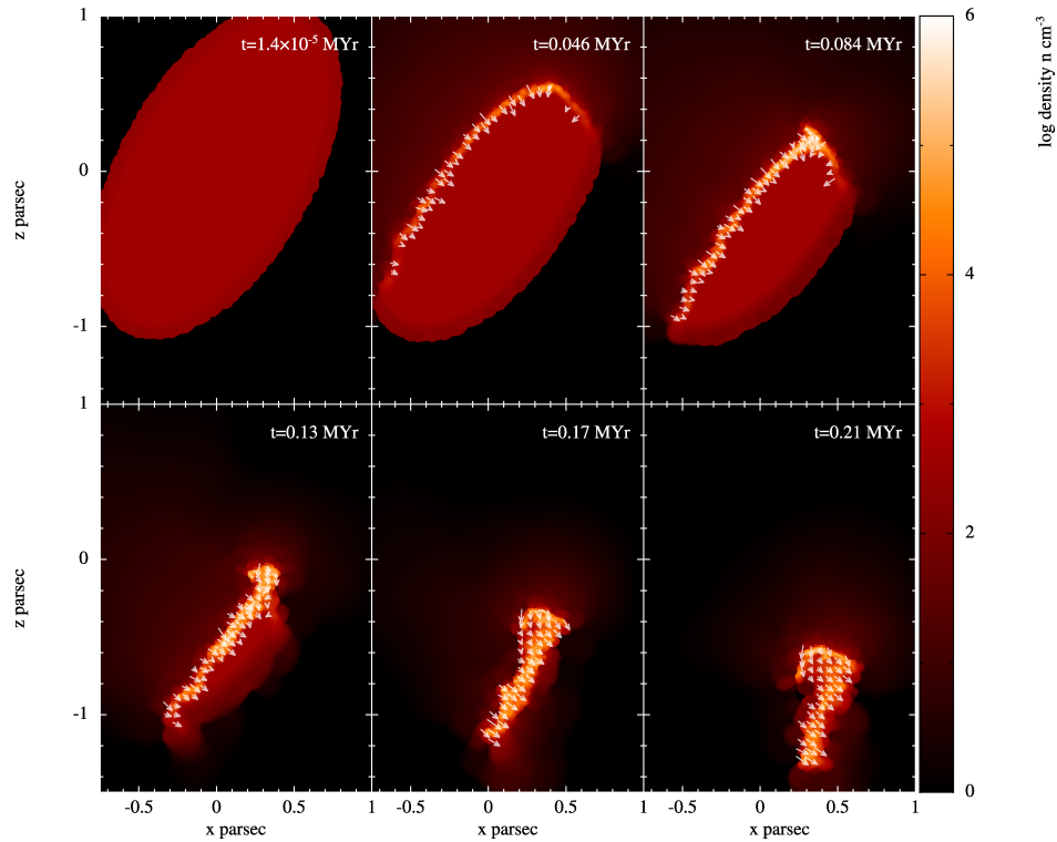
Figure 18. The evolution of the RDI induced shock velocity of cloud G400( F_2 ) overlapped in the corresponding cross-section density snapshot. The magnitude of the velocity is between 2 and 12 \text{ km s}^{-1} .
