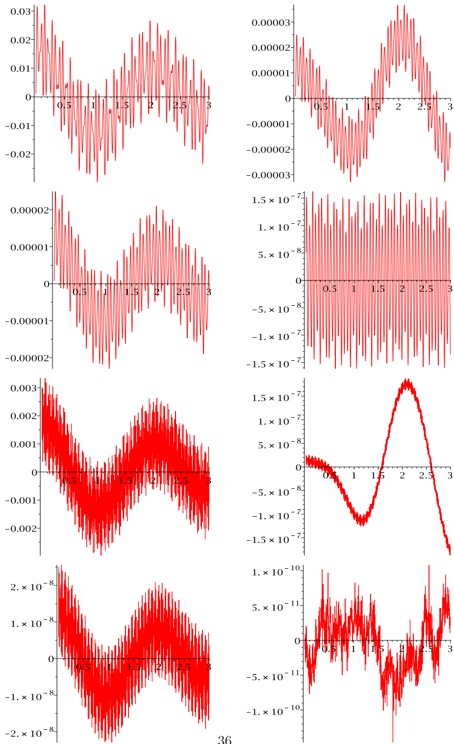
Figure 4.10: The top row: the real parts of error function with s = 0 (the left) and s = 1 (the right) for y_5 with \omega = 100 . The middle row: the real parts of error function with s = 2 (the left) and s = 3 (the right) for y_5 with \omega = 100 . The third row: the real parts of error function with s = 0 (the left) and s = 1 (the right) for y_5 with \omega = 1000 . The fourth row: the real parts of error function with s = 2 (the left) and s = 3 (the right) for y_5 with
