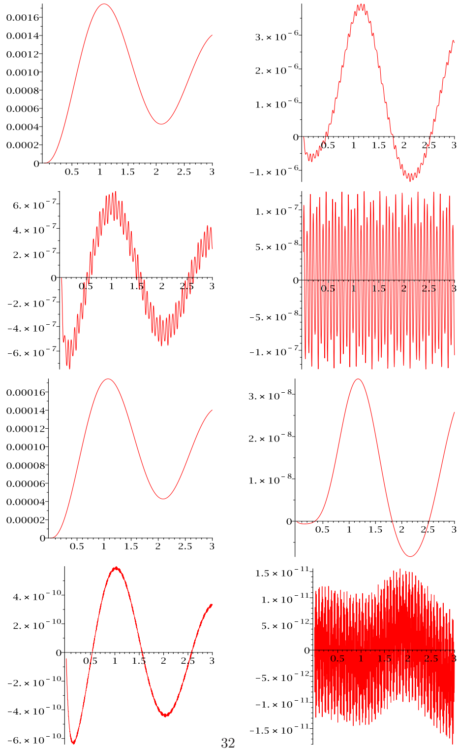
Figure 4.6: The top row: the real parts of error function with s = 0 (the left) and s = 1 (the right) for y_1 with \omega = 100 . The middle row: the real parts of error function with s = 2 (the left) and s = 3 (the right) for y_1 with \omega = 100 . The third row: the real parts of error function with s = 0 (the left) and s = 1 (the right) for y_1 with \omega = 1000 . The fourth row: the real parts of error function with s = 2 (the left) and s = 3 (the right) for y_1 with
