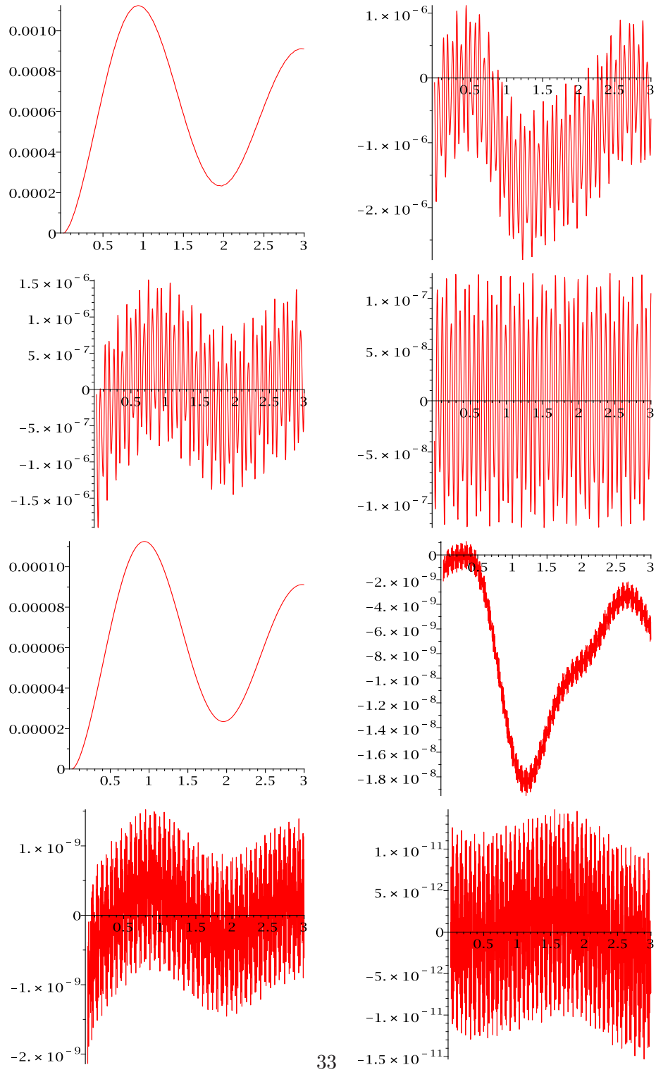
Figure 4.7: The top row: the real parts of error function with s = 0 (the left) and s = 1 (the right) for y_2 with \omega = 100 . The middle row: the real parts of error function with s = 2 (the left) and s = 3 (the right) for y_2 with \omega = 100 . The third row: the real parts of error function with s = 0 (the left) and s = 1 (the right) for y_2 with \omega = 1000 . The fourth row: the real parts of error function with s = 2 (the left) and s = 3 (the right) for y_2 with
