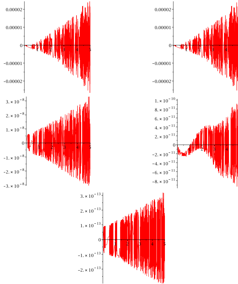
Figure 4.1: The real part of the error in x committed by the asymptotic expansion, as applied to the linear system (4.1) with \omega = 500 for s = 0, 1, 2, 3, 4 (from top left onwards).
