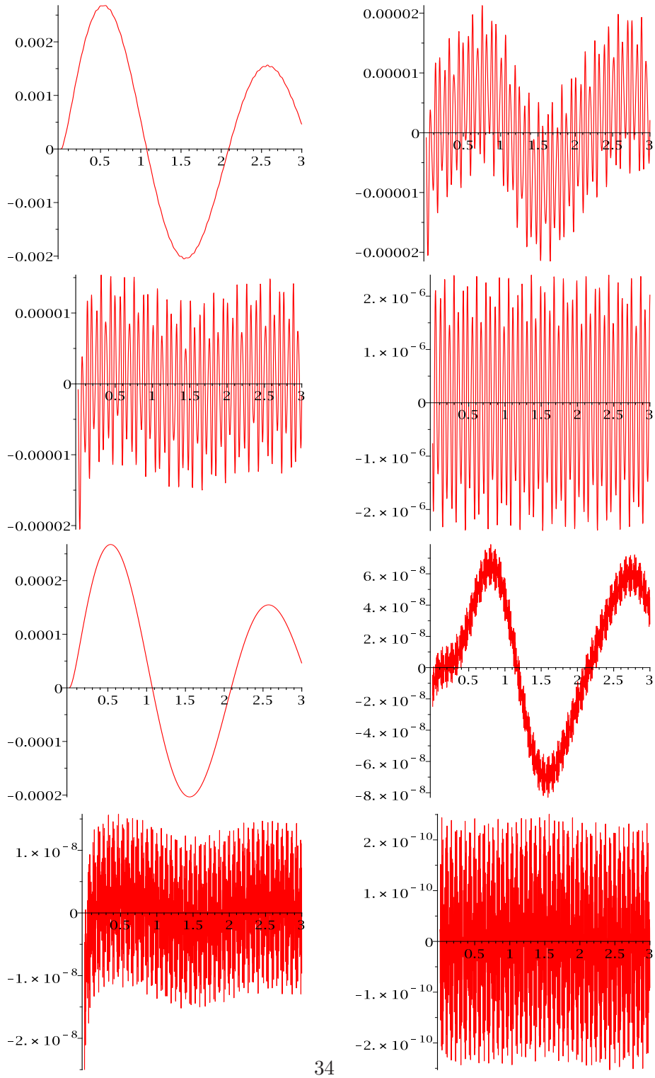
Figure 4.8: The top row: the real parts of error function with s = 0 (the left) and s = 1 (the right) for y_3 with \omega = 100 . The middle row: the real parts of error function with s = 2 (the left) and s = 3 (the right) for y_3 with \omega = 100 . The third row: the real parts of error function with s = 0 (the left) and s = 1 (the right) for y_3 with \omega = 1000 . The fourth row: the real parts of error function with s = 2 (the left) and s = 3 (the right) for y_3 with
