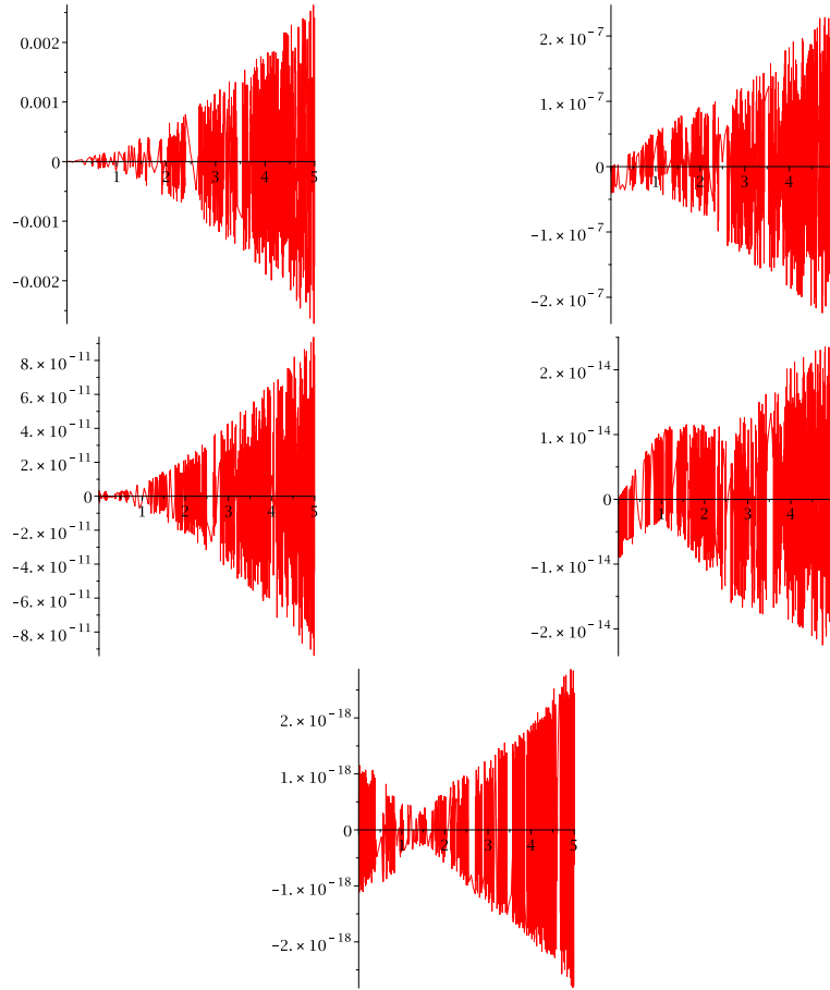
Figure 4.4: The real part of the error in \dot{x} committed by the asymptotic expansion, as applied to the linear system (4.1) with \omega = 5000 for s = 0, 1, 2, 3, 4 (from top left onwards).
