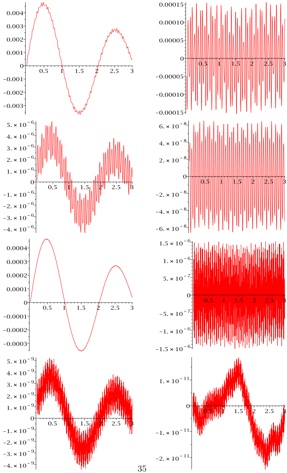
Figure 4.9: The top row: the real parts of error function with s = 0 (the left) and s = 1 (the right) for y_4 with \omega = 100 . The middle row: the real parts of error function with s = 2 (the left) and s = 3 (the right) for y_4 with \omega = 100 . The third row: the real parts of error function with s = 0 (the left) and s = 1 (the right) for y_4 with \omega = 1000 . The fourth row: the real parts of error function with s = 2 (the left) and s = 3 (the right) for y_4 with
