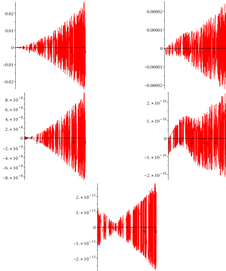
Figure 4.2: The real part of the error in \dot{x} committed by the asymptotic expansion, as applied to the linear system (4.1) with \omega = 500 for s = 0, 1, 2, 3, 4 (from top left onwards). It is shown that the error decreases once s is increased from 0 to 1.
