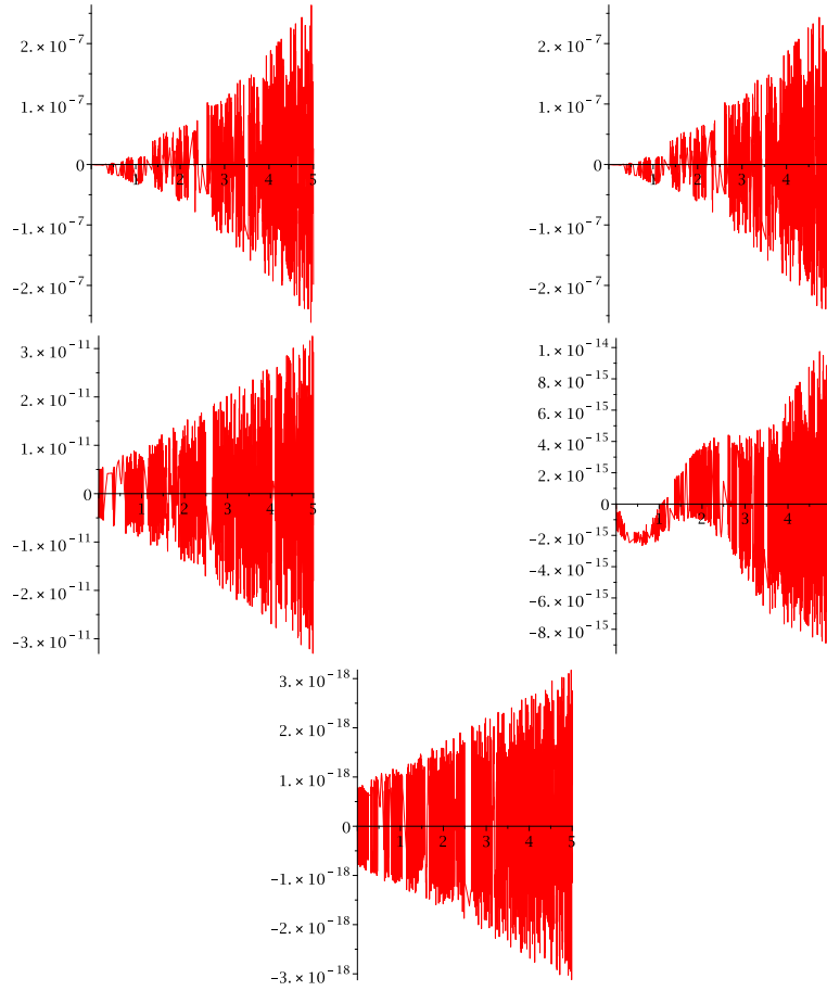
Figure 4.3: The real part of the error in x committed by the asymptotic expansion, as applied to the linear system (4.1) with \omega = 5000 for s = 0, 1, 2, 3, 4 (from top left onwards).
