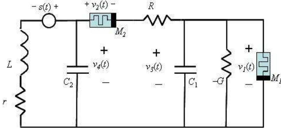
Figure 4.5: The Memristor circuits.
