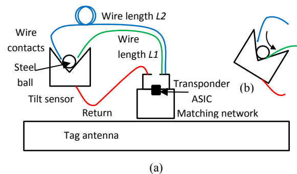
Figure 1: (a) tilt sensing tag schematic showing 2 of 4 wire connections, (b) tilt sensor tilted in one axis.
