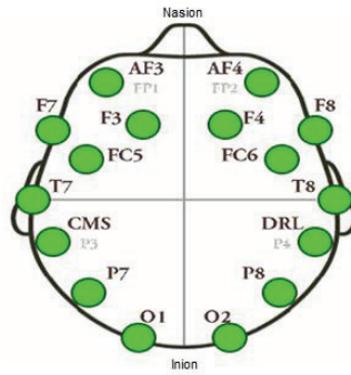
Fig. 1 (d) Electrode positions, according to the 10-20 system, of the Emotiv EPOC device used for EEG acquisition.
