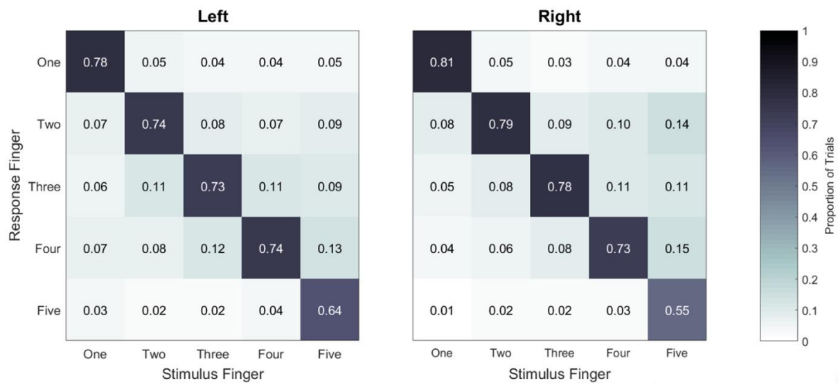
Figure 2: Grand average confusion matrices showing the proportion of stimuli judged as located on each of the five digits as a function of which digit was actually stimulated. Digits were identified by numbers one (thumb) through five (little finger). Data from the left hand is shown in the left panel, and from the right hand in the right panel. The proportion of correct responses for each digit is shown along the diagonal from the top-left to the bottom-right. The off-diagonal cells represent mislocalisations between the digits.
