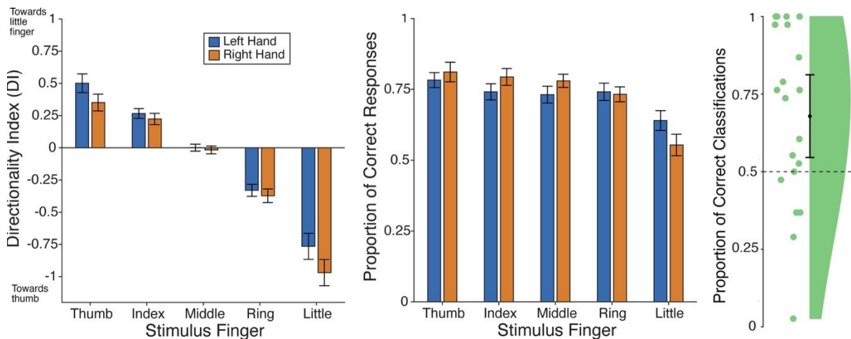
Figure 3: The left panel shows the grand average directionality index (DI) scores for each finger, on the left and right hands. The centre panel shows the grand average percentage of correct responses made to each finger, on both hands. Error bars represent the standard error of the mean. Similar patterns of results were found for the two hands, for both DI and accuracy. The right panel shows classification accuracy in the RSA analysis, shown using a raincloud plot (Allen et al. 2021). Points show data from individual participants. The dashed line indicates chance classification performance (i.e., 50%). The black circle and error bar indicate the mean and 95% confidence interval. Classification accuracy was significantly above chance levels, indicating shared individual differences in patterns of confusion between the two hands.
