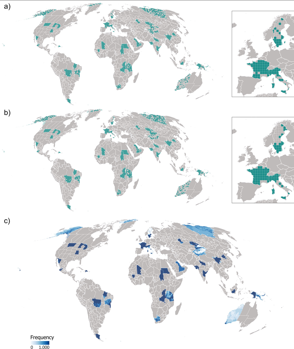
Extended Data Fig. 2 | Details of the 1,000 sets of sampling units used to extrapolate global conservation area coverage. All the sampling units were within a representative set of 25 countries and territories identified in a previous study 8 ; national and subnational units not included in the samples are shown in grey. Map data from ref. 8, under a Creative Commons licence CC BY 4.0. Base maps use United Nations ClearMap/Official United Nations Boundaries from the United Nations Geospatial Network. (a) and (b) illustrate two of the 1,000 sets of sampling units in green, with insets showing Western Europe. Each set of sampling units has a minimum combined area while
