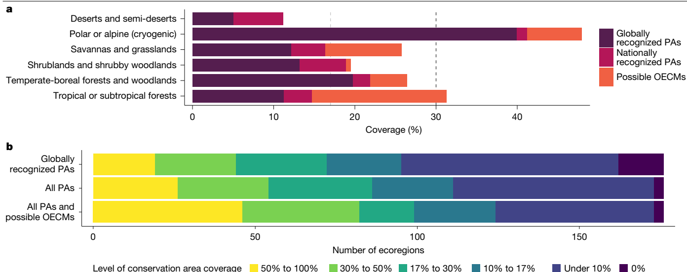
Fig. 2 | Ecological representativeness of the different conservation area types. a , Mean percentage of the six terrestrial functional biomes 30 covered by the three conservation area types in a representative sample of land covering 10% of the terrestrial realm. b , Mean number of ecoregions 33 belonging to different categories of conservation area coverage in the representative sample, showing coverage based on globally recognized PAs, all PAs (globally recognized PAs + nationally recognized PAs) and all conservation areas (globally recognized PAs + nationally recognized PAs + possible OECMs). The analysis only includes ecoregions with more than 10% of their coverage in
