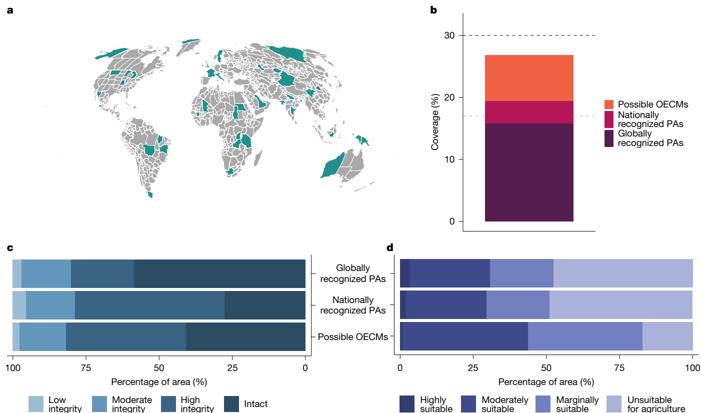
Fig. 1 | Global conservation area type coverage and characteristics. a , Set of 9 countries and territories, plus subnational sections of another 16 countries, from which all available terrestrial conservation area spatial datasets were collected and synthesized. Subsequent analyses were based on 1,000 sets of 100 km × 100 km sampling units; each set was in the area shown in green and met the 10% coverage targets for each of the features known to influence conservation area extent and global biodiversity patterns. b , Mean cumulative coverage of the three different conservation area types, based on combining several different international and national datasets, in the representative sample of land covering 10% of the terrestrial realm. The dotted lines show the 17% and 30% coverage values from previous and continuing global targets.
