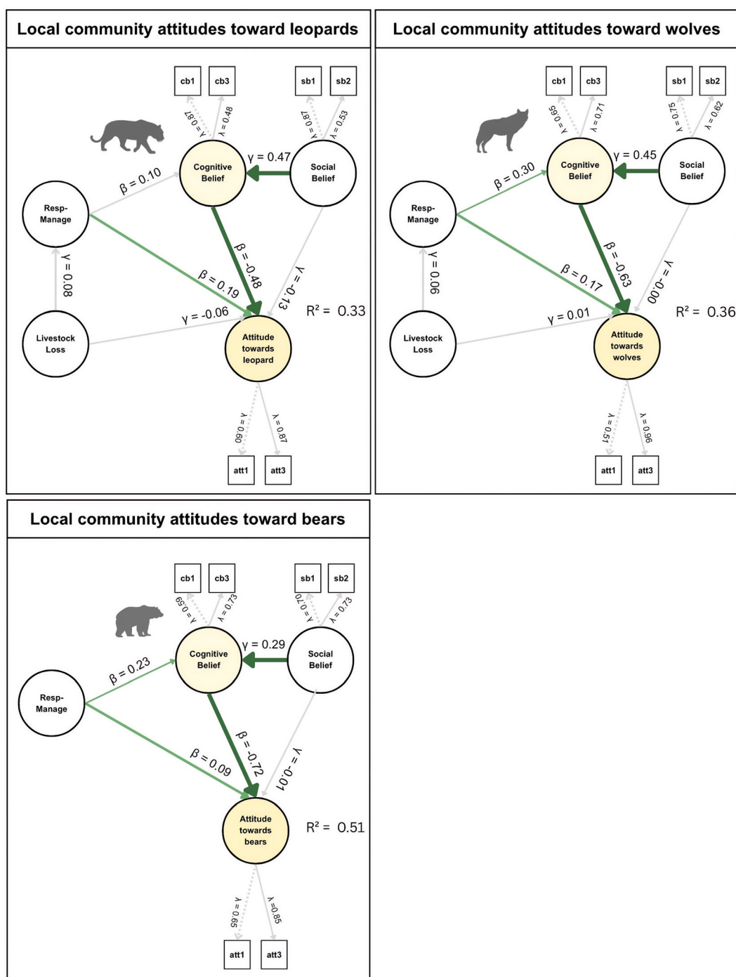
Fig. 3 Bayesian structural equation modelling results of local community attitudes toward leopards, wolves, and bears around Golestan National Park, northeastern Iran. Circles represent latent variables; squares represent observed indicator items. Lambda ( \lambda ) values show standardised factor loadings, indicating the strength of the relationship between each latent variable and its indicators; dotted lines denote the marker indicator fixed to identify each latent variable in the model. Beta ( \beta ) values show standardised path coefficients for regressions between two exogenous items (e.g., Responsibility for Management to Cognitive Beliefs); gamma ( \gamma ) values show standardised path coefficients between one endogenous and one exogenous (Social Belief to Cognitive Belief). Green lines and coefficients indicate a substantial relationship; grey lines and coefficients indicate a non-substantial relationship. Line thickness is scaled to the magnitude of the standardised coefficient. The double-headed grey arrow between Responsibility for Management and Livestock Loss represents the estimated covariance between these two exogenous variables, not a directional or causal relationship. R^2 values indicate the proportion of variance in attitude explained by the model for each species
