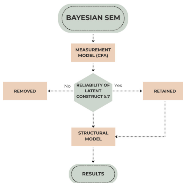
Fig. 2 Flowchart to represent the two-step workflow of Bayesian SEM modelling. CFA is an abbreviation for Confirmatory Factor Analysis
