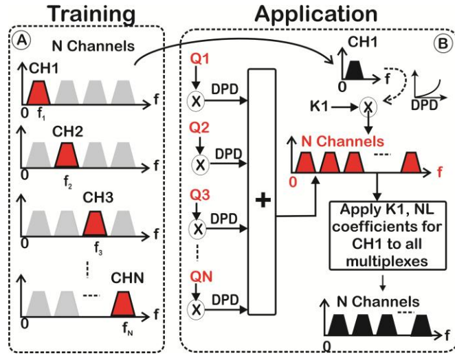
Fig. 3. Conceptual depiction of the hybrid DPD training approach. Q1-QN represents the extracted memory coefficients. Specifically, Q1, Q2, Q3, and QN correspond to the memory coefficients for channels CH1, CH2, CH3, and CHN, respectively, while K1 denotes amplitude nonlinearity coefficients extracted from CH1. The left (A) represents the channels being used for the training, whereas the right (B) represents how the extracted coefficients are applied. Dark red is an active channel; light grey is an inactive channel.
