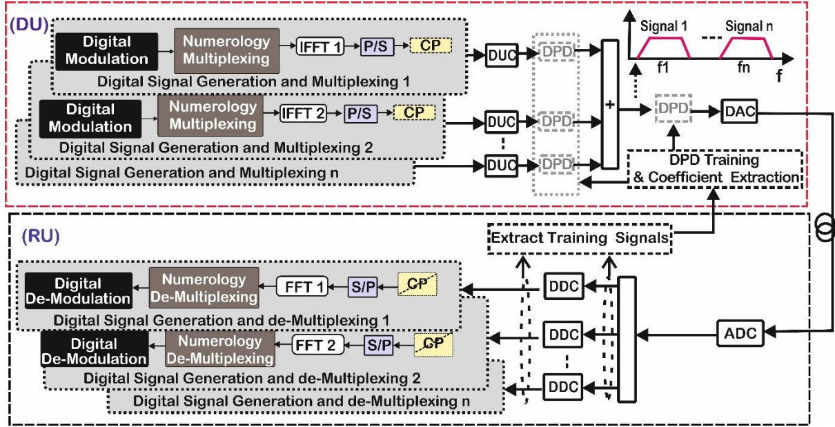
Fig. 1. Conceptual view of Distributed Unit (DU) and Remote Unit (RU) processes for the downlink DSP-assisted optical mobile fronthaul with DPD. DUC, Digital-Up-Converter; DDC, Digital Downconverter; DAC, Digital-to-Analogue Converter; CP, Cyclic Prefix; ADC, Analogue-to-Digital Converter; PS, parallel to serial; S/P, serial to parallel; IFFT, Inverse Fast Fourier Transform; FFT, Fast Fourier Transform.
