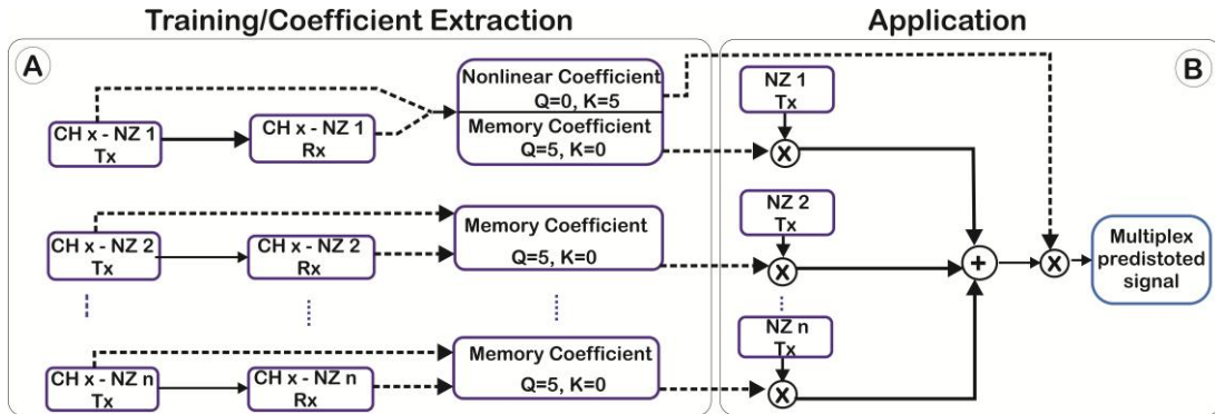
Fig. 9. Conceptual depiction of the NZ-based DPD training approach. Solid lines represent data links; dashed lines represent control information links.
