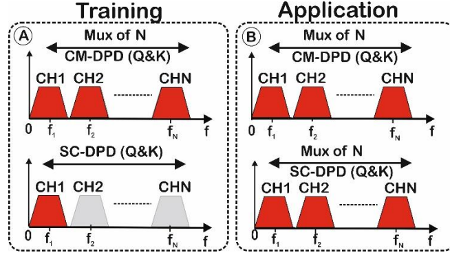
Fig. 2 Conceptual depiction of the CM-DPD and SC-DPD training and application workflows. Left (A): channels used for training (CM-DPD, top; SC-DPD, bottom). Right (B): application of the extracted coefficients to CM-DPD (top) and SC-DPD (bottom). (Q) denotes memory coefficients and (K) nonlinear coefficients. Dark red is an active channel; light grey is an inactive channel.
