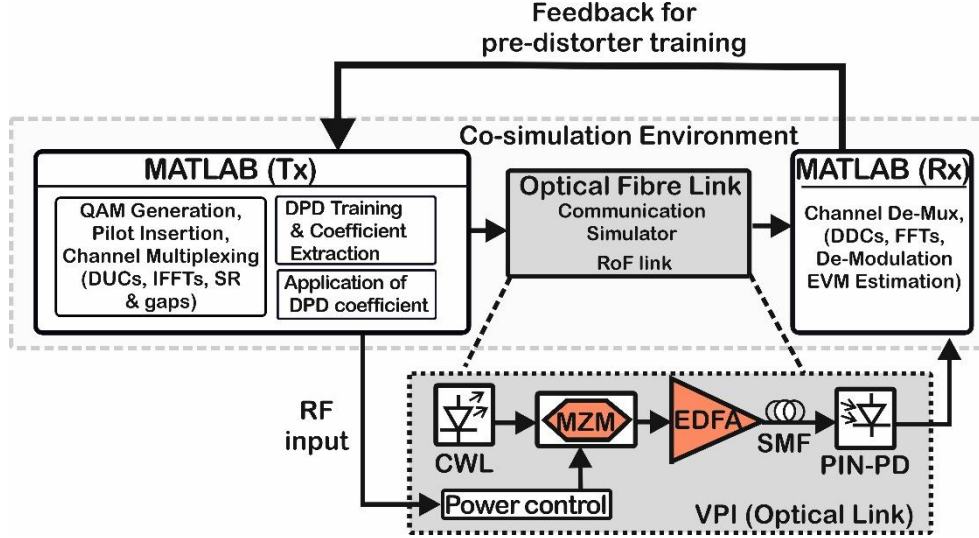
Fig. 4. Co-simulation environment for generation and reception of composite signals/multiplexes, DPD coefficient estimation and predistortion. MZM, Mach-Zehnder Modulator; EDFA, Erbium-Doped Fiber Amplifier; SMF, Single-Mode Fiber; CWL, Continuous-Wave Laser, PD, Photo Diode.
