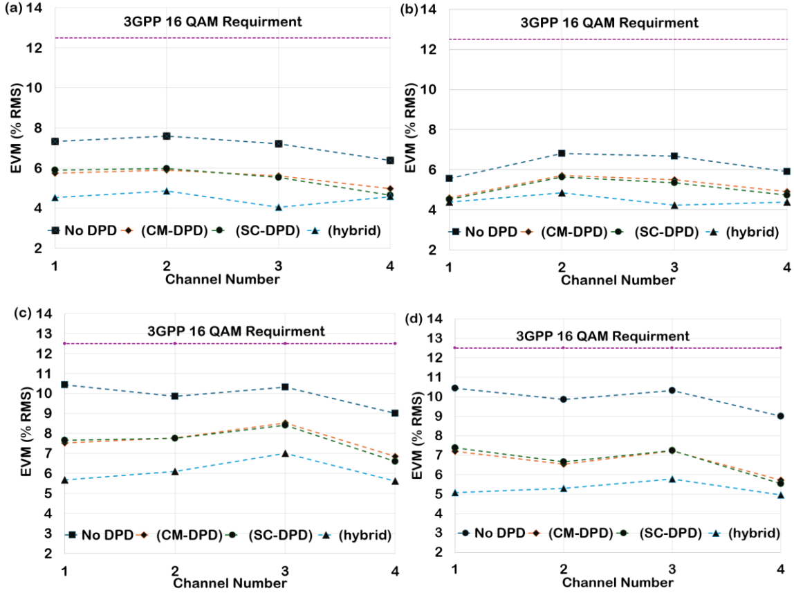
Fig. 5. Per-channel Error Vector Magnitude (EVM, % RMS) for 16 QAM modulation, before and after DPD for a signal multiplex comprising four channels, with a total input power ( P_{in} ) of 19 dBm. (a) 100 MHz channel bandwidths, with the first channel centered at 50 MHz. (b) 100 MHz channel bandwidths, with the first channel centered at 1200 MHz. (c) 400 MHz channel bandwidths, with the first channel centered at 200 MHz. (d) 400 MHz channel bandwidths, with the first channel centered at 1200 MHz. Dashed lines are used only to associate results for similar systems and do not indicate trends between adjacent points.
