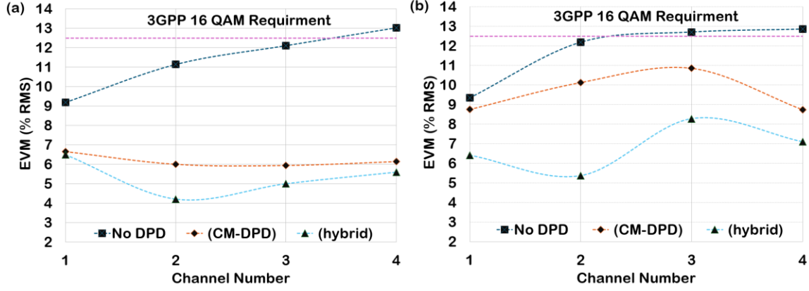
Fig. 7. Per-channel Error Vector Magnitude (EVM, % RMS) measurement results for 16 QAM modulation, before and after DPD for a signal multiplex, comprising four channels, at an input power of 10 dBm. (a) 74.38 MHz channel bandwidth, and (b) 100 MHz channel bandwidth. In both cases, the first channel is centered at 50 MHz. Dashed lines are used only to associate results for similar systems and do not indicate trends between adjacent points.
