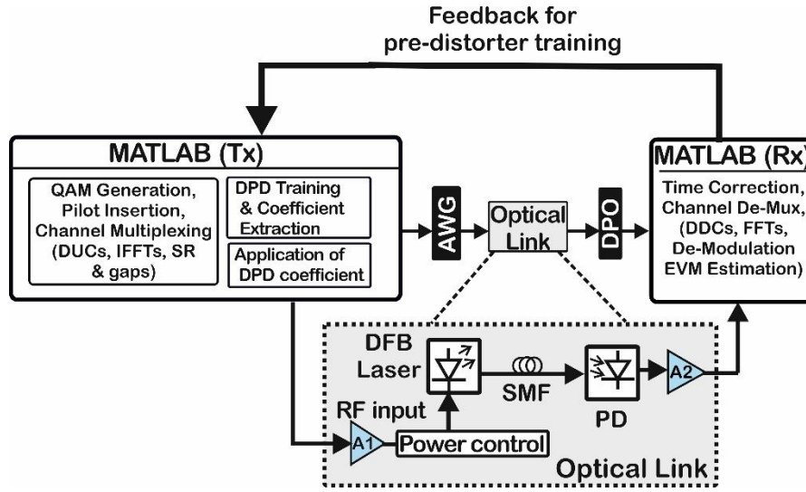
Fig. 6. Experimental setup for EVM measurements. AWG, Arbitrary Waveform Generator; DPO, Digital Phosphor Oscilloscope; DFB, Distributed Feedback Laser; A1, Electronic Amplifier 1; SMF, Single-Mode Fiber; PD, Photodiode; A2, Electronic Amplifier 2.
