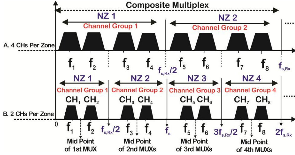
Fig. 8. Conceptual depiction of NZ-based mapping at the transmitter side, for an 8-channel multiplex showing two mapping examples, with two and four NZs, respectively. The f_{s,Rx} is the sampling rate employed at the receiver side DDC.
