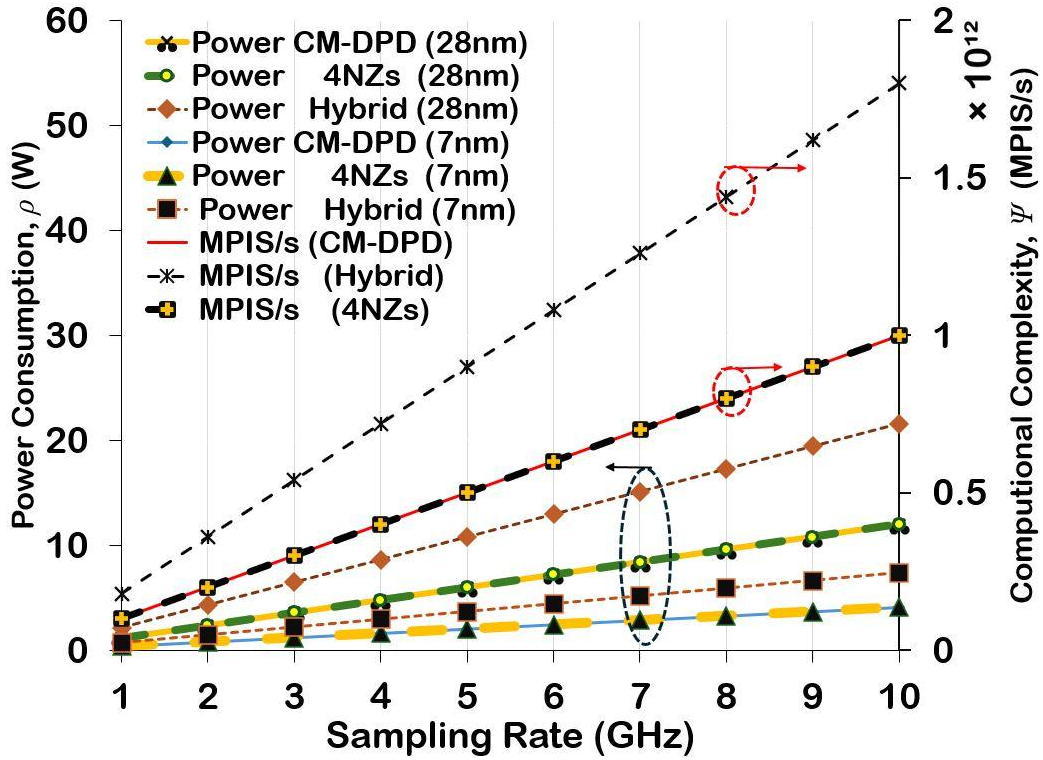
Fig. 10. DPD power consumption (left y-axis) and Multiplications per Input Sample per second (MPIS/s) (right y-axis) versus sampling rate for an eight-channel multiplex. The 28-nm and 7-nm labels refer to CMOS technologies implemented with 28-nm and 7-nm process nodes, respectively.
