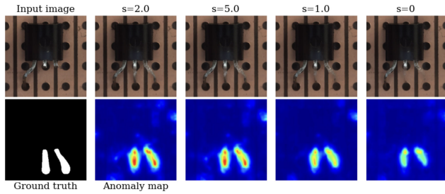
FIGURE 5. Qualitative results of anomaly detections of ProtoDiffAD depending on the guidance scale s .
