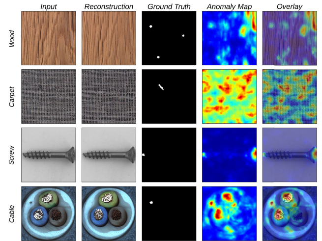
FIGURE 6. Examples of failure cases for ProtoDiffAD's anomaly detection.
