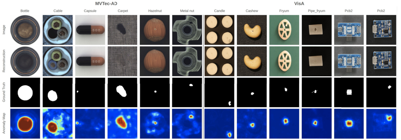
FIGURE 1. Qualitative results of ProtoDiffAD on the MVTec-AD and VisA datasets.
