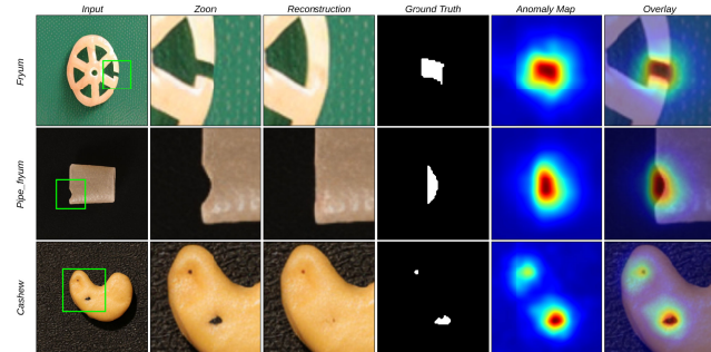
FIGURE 2. Anomaly detection results of ProtoDiffAD for samples having a tiny-sized anomaly area. The VisA dataset is used for the experiments.
