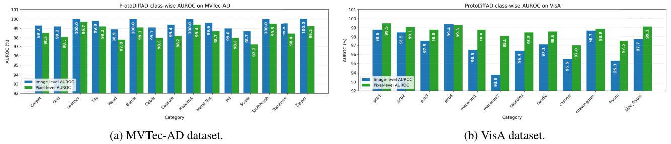
FIGURE 7. Class-wise image-level detection and pixel-level AUROCs of ProtoDiffAD on the MVTec-AD and VisA datasets.
