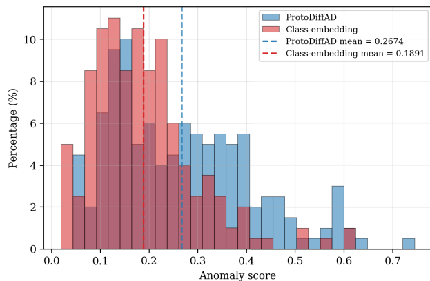
FIGURE 4. Anomaly score distribution of the ‘Class embedding’ with LDM and ProtoDiffAD.
