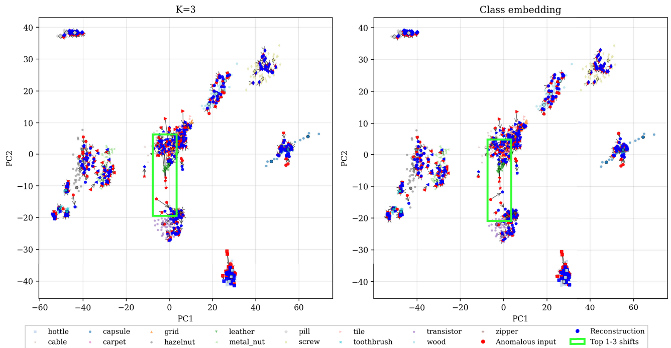
FIGURE 3. Latent feature distribution of each category depending on the conditioning approach on the MVTec-AD datasets. We compare ‘Class embedding’, which is a naive LDM conditioned with explicit class context, and ProtoDiffAD with K = 3 . We apply PCA to the output of \mathcal{E}_\phi(x) for dimension reduction. The 15 samples that produce the top 15 differences between anomalous and reconstruction results are connected by arrow lines.
