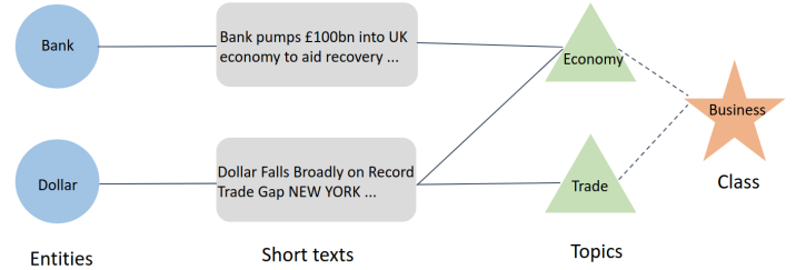
Fig. 1. Example Snippet from a Heterogeneous Graph Structure
