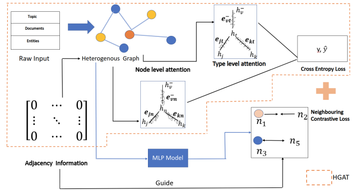
Fig. 2. Illustration of our NC-HGAT model
