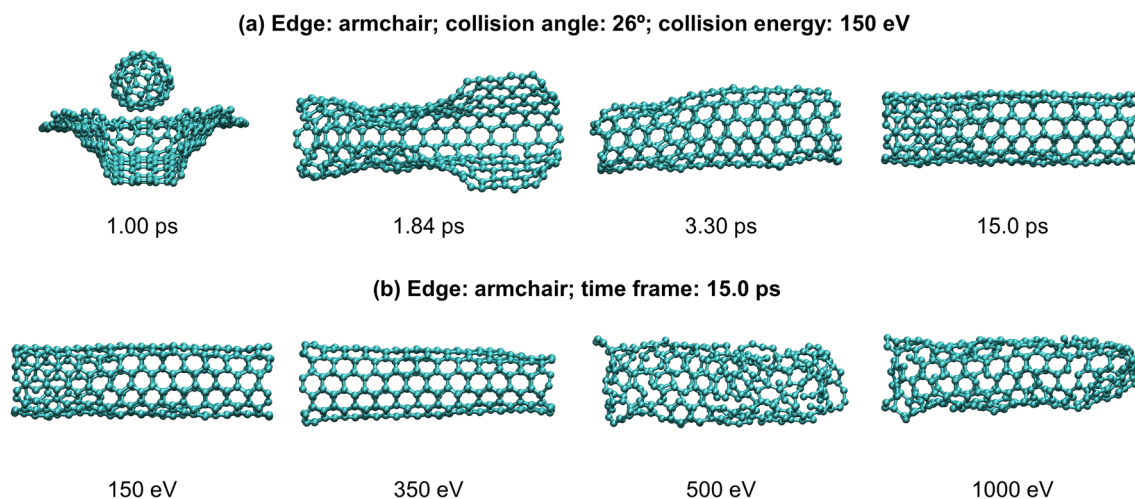
Fig. 6 Mechanism of edge-mediated topological closure of a graphene nanoflake from a fullerene collision aimed at the armchair edge of a C_{296} graphene nanoflake following ballistic impact. a Time-resolved snapshots for a representative trajectory at an incidence angle of 26^\circ and a collision energy of 150 eV, illustrating the sequence from initial edge contact and grazing penetration of the C_{60} projectile, through local bending and progressive, zipper-like seam formation between opposing zigzag edges, to the emergence of a fully connected nanotube by t = 15.0 ps. The simulation snapshot at intermediate instant ( t \approx 1.84 ps) highlights the systematic propagation of edge-to-edge bonding away from the impact region. b Final morphologies obtained at increasing collision energies (150, 350, 500, and 1000 eV) for the same edge orientation, showing the transformation from open-ended nanotubes at lower energies to closed, cage-terminated nanotubes at higher energies, driven by enhanced post-closure energy redistribution and secondary bond reorganisation at the tube extremities
