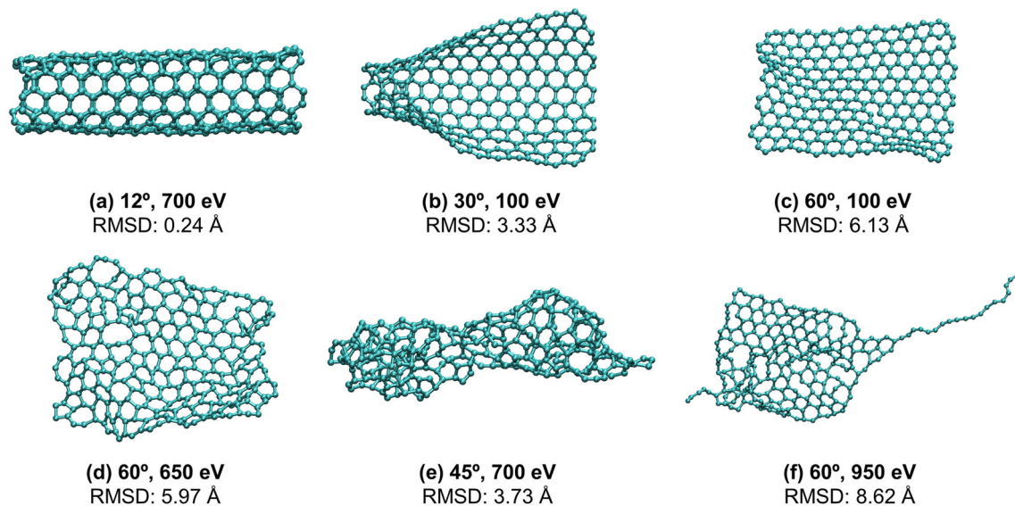
Fig. 2 Representative structural outcomes obtained from collision-driven transformations towards the armchair edge of C_{296} graphene nanoflakes, illustrating selected metastable morphologies with distinct topologies. The incidence angle \theta and collision energy E for each trajectory are indicated. a Fully stitched nanotube exhibiting minimal deviation from the reference tubular geometry. b Partially closed tubular segment with incomplete seam propagation and one open end. c Non-planar nanoflake formed through bending without edge-to-edge bonding. d Non-planar flake with pronounced local defects and non-hexagonal ring motifs near the impact region. e Amorphous aggregate characterised by dense three-dimensional packing and loss of extended sheet or tubular topology. f Amorphous structure featuring extended, undercoordinated linear carbon tails protruding from a disordered core. RMSD values are reported relative to the corresponding reference nanotube geometry
