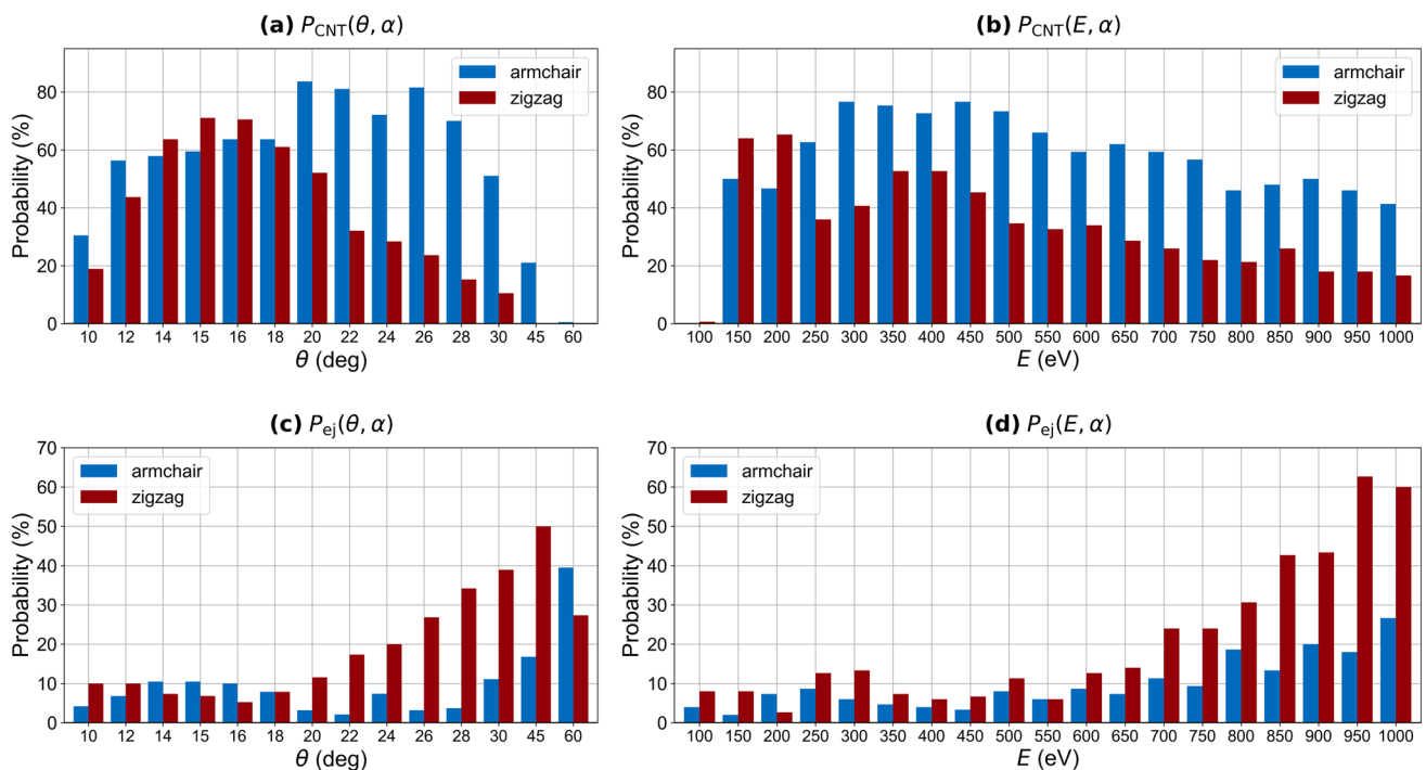
Fig. 3 Statistical characterisation of collision outcomes for C_{60} impacts on armchair and zigzag edges of C_{296} graphene nanoflakes. Panels a and b report the angle- and energy-resolved probabilities of nanotube-like formation, P_{CNT}(\theta, \alpha) and P_{CNT}(E, \alpha) . Panels c and d show the corresponding probabilities of atom-ejection events, P_{ej}(\theta, \alpha) and P_{ej}(E, \alpha) . Blue and red bars denote armchair and zigzag edge-oriented collisions, respectively. The four panels highlight the distinct response of the two edge topologies, including the broader angular and energetic window for nanotube-like formation in armchair-directed collisions and the higher probability for atom ejection in the zigzag counterpart
