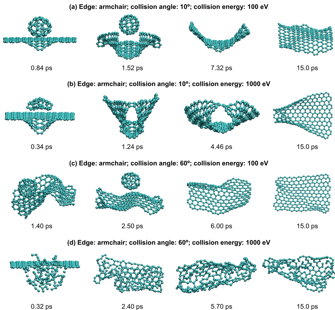
Fig. 5 Representative armchair edge-aimed collision-induced outcomes in regimes that do not lead to the formation of nanotube-like structures. a Low incidence angle (10°) and low collision energy (100 eV): the fullerene traverses the flake, inducing transient bending and global non-planar distortion without driving the opposing edges into contact, yielding an open, deformed nanoflake. b Low incidence angle (10°) and high collision energy (1000 eV): excessive local energy deposition produces extensive bond reorganisation and the formation of a four-membered ring bridging the two sides of the flake, together with a large, irregular aperture, resulting in an asymmetric, defect-rich cluster with a partially capped and an open end. c High incidence angle (60°) and low collision energy (100 eV): the momentum is transferred into long-wavelength flexural modes, generating an S-shaped deformation and rebound of the projectile without edge-to-edge bonding. d High incidence angle (60°) and high collision energy (1000 eV): severe and irreversible disruption of both projectile and target leads to atom ejection (36 atoms removed from the nanoflake, yielding C 260 ) and the formation of a highly defective, loosely tubular cluster. Snapshots are shown at selected instants of each simulated trajectory, illustrating the progression from initial impact to the final metastable or defective morphology at 15 ps
