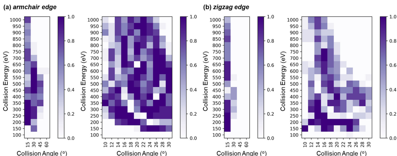
Fig. 4 Probability maps for successful transformation to nanotube-like structures, P_{CNT} , as a function of collision energy and incidence angle for (a) armchair and (b) zigzag edge orientations of the C_{296} graphene nanoflake. For each edge type, the left panel shows a coarse angular overview at representative angles of 15^\circ , 30^\circ , 45^\circ , and 60^\circ , while the right panel provides a high-resolution view of the low-angle regime ( 10^\circ – 30^\circ ) sampled at 2^\circ increments. Each bin corresponds to a single (E, \theta) parameter set and is colour-coded according to the bar scale, representing the probability of satisfying the criterion for nanotube-like structure formation, ranging from 0 (white) to 1 (dark purple). Regions of high transformation probability ( P_{CNT} \gtrsim 0.6 ) delineate intermediate-energy and low-to-moderate-angle windows—typically around E \approx 200 – 700 eV and \theta \approx 10^\circ – 30^\circ for armchair-edge impacts—in which cooperative bending, edge-to-edge contact, and subsequent seam formation are most likely to occur
