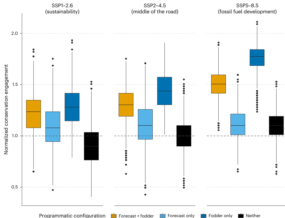
Fig. 6 | Results of experiment 3. Boxplots show the level of community engagement with the conservation initiative resulting from the last 30 iterations for each of 50 repetitions for the agent-based model run on each precipitation scenario and for each programmatic configuration. Horizontal black lines show median values. Boxes contain the inner 50% of the data, that is second and third quartiles. Whiskers show data within 1.5 times the interquartile range.
