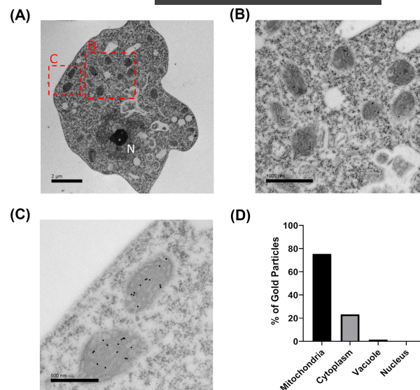
FIGURE 4 Immunoelectron microscopy reveals AOX localization within the inner mitochondrial membrane. Fixed Naegleria gruberi samples were probed for IEM to assess their localization in the mitochondria (A). The AOX signal derived by the immunogold secondary antibodies bound against AOX primary antibodies localizes predominantly inside the mitochondria (B, C). The gold particles were then quantified based on their localisation (D).
