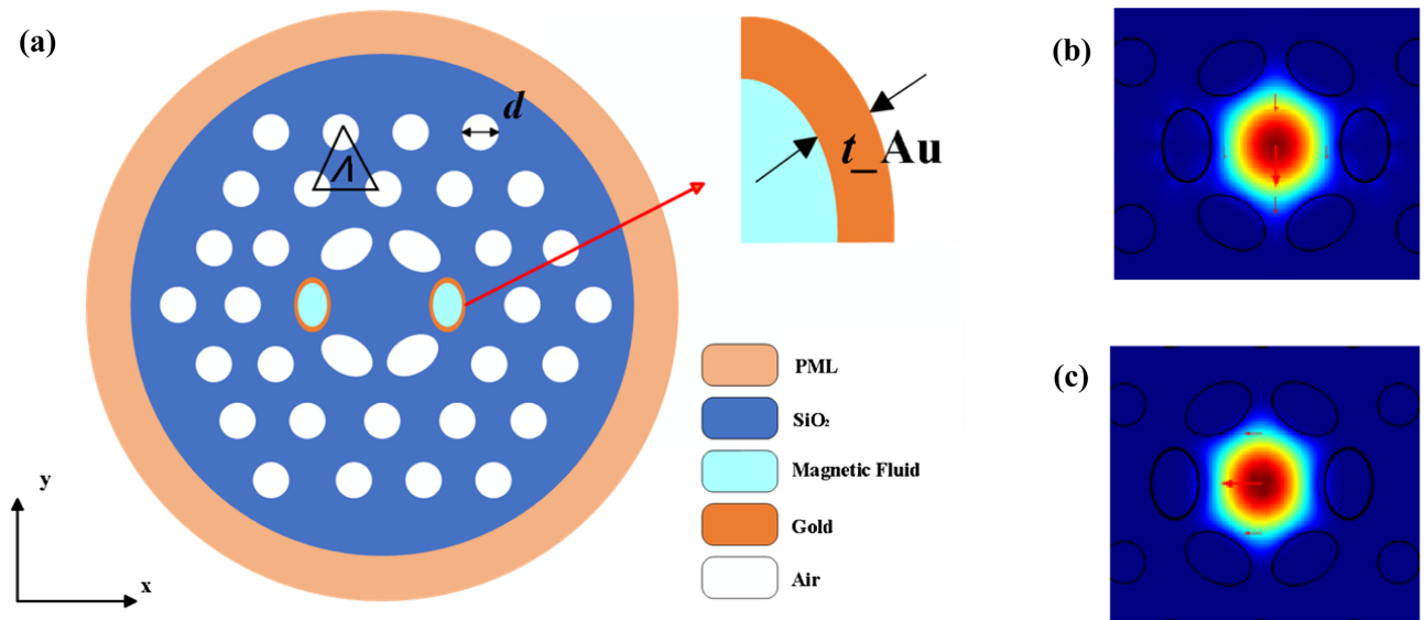
Fig. 1. (a) Cross section of the PCF-SPR sensor; (b) electric field distribution of the Y-Pol fundamental mode at 650 nm; (c) electric field distribution of the X-Pol fundamental mode at 650 nm.
