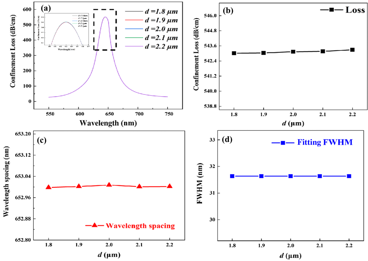
Fig. 6. (a) Influence of d on the loss spectrum; (b) peak total loss variation of the sensor when the d range is 1.8–2.2 \mu\text{m} ; (c) variation of the resonance wavelength of the sensor when d ranges from 1.8 to 2.2 \mu\text{m} ; (d) FWHM variation of the sensor when d ranges from 1.8 to 2.2 \mu\text{m} .
