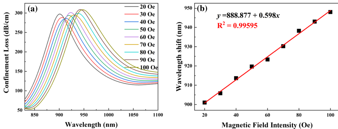
Fig. 9. (a) Effect of optimized elliptical channel fiber optic sensors on loss spectra in different magnetic fields from 20 to 100 Oe; (b) results of fitting the SPR resonance wavelength of the X-Pol core mode to the magnetic field variations in the two structures.
