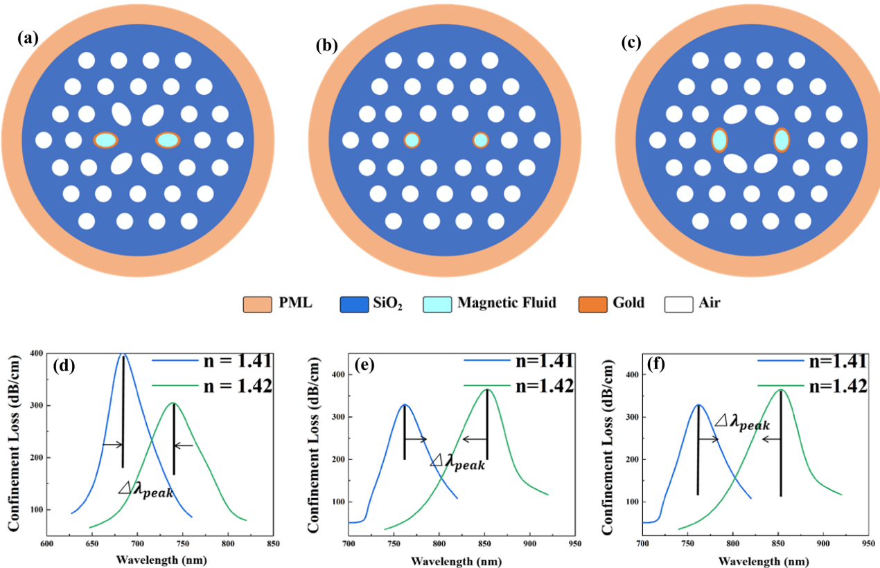
Fig. 4. Horizontal and vertical axes of elliptical channels. (a) a > b ; (b) a = b ; (c) a < b ; (d) loss spectrum under different long and short axes; (e) wavelength shift when a < b ; (f) wavelength shift when a > b .
