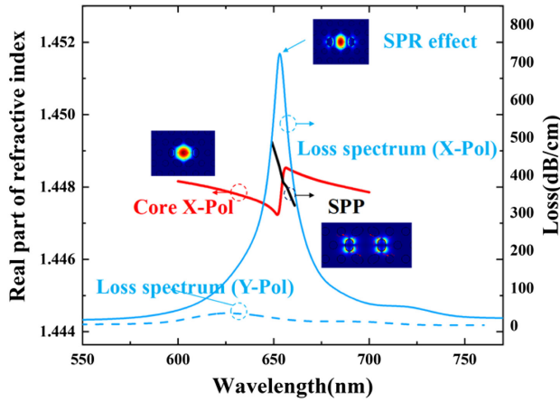
Fig. 3. Dispersion relationship between the X-Pol fiber and Y-Pol fiber core mode, SPP mode, and the loss spectrum of the PCF-SPR sensor.
