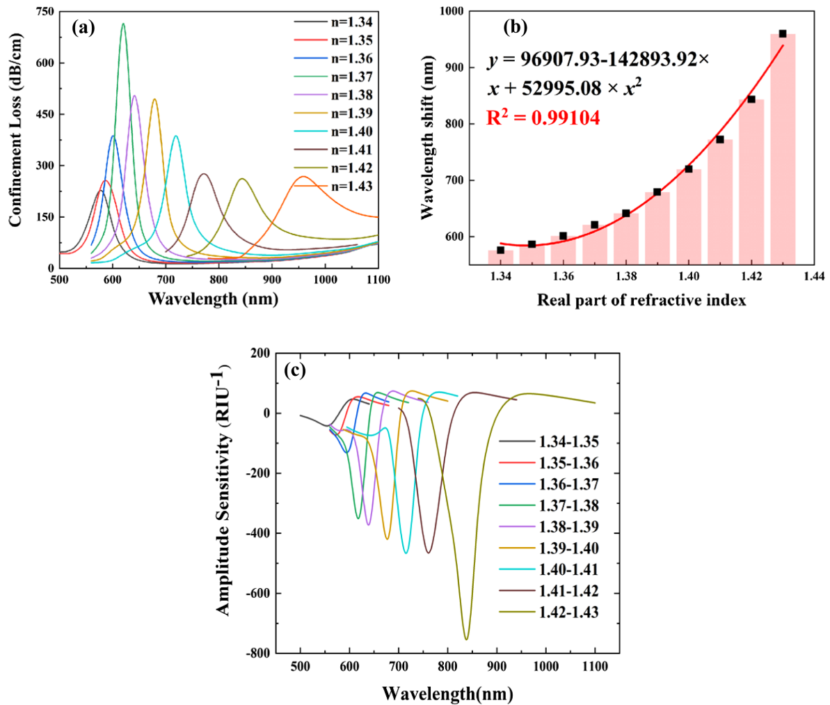
Fig. 8. (a) Influence of different RI on the loss spectrum of the optimized optical fiber sensor at the RI of 1.34–1.43; (b) fitting results of SPR resonance wavelength variation with RI of the X-Pol core mode; (c) effect of different RI on amplitude sensitivity at RI of 1.34–1.43.
