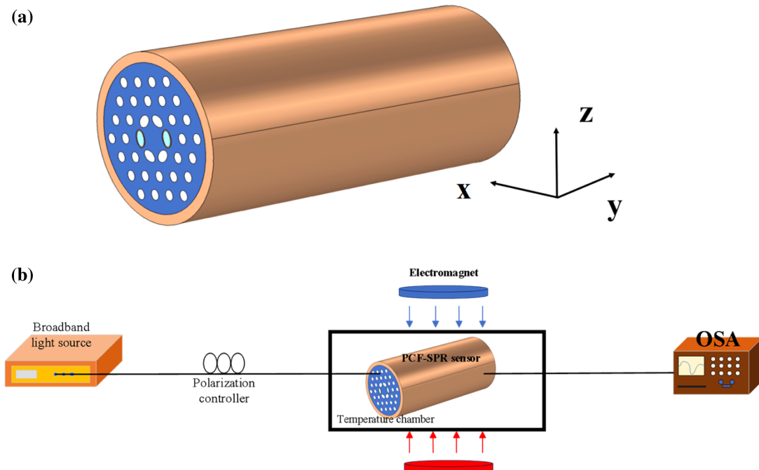
Fig. 2. (a) Schematic of the three-dimensional (3D) model of the sensor; (b) experimental device of the sensor.
