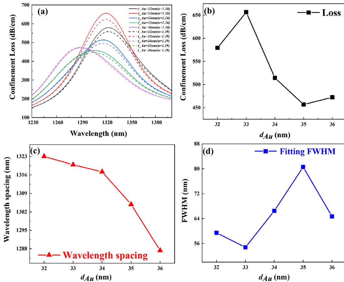
Fig. 7. (a) Influence of t_{Au} on the loss spectrum; (b) peak total loss variation of the sensor when the t_{Au} range is 32–36 nm; (c) variation of the resonance wavelength of the sensor when t_{Au} ranges from 32 to 36 nm; (d) FWHM variation of the sensor when t_{Au} ranges from 32 to 36 nm.
