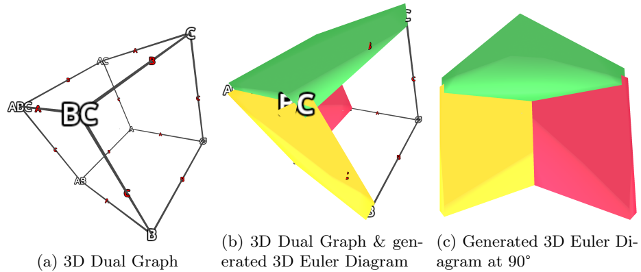
Fig. 1: Output with the abstract description: \emptyset, A, B, C, AB, AC, BC, ABC
