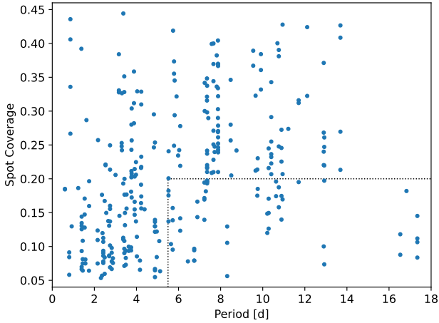
Figure 8. Stellar rotation periods vs. the coverage for all cold spots in our sample. A lack of small spots on slow rotators is evident (bounded by the black dotted lines). The typical uncertainties of the spot coverage are 0.02. The period uncertainties are typically smaller than the symbol size.
