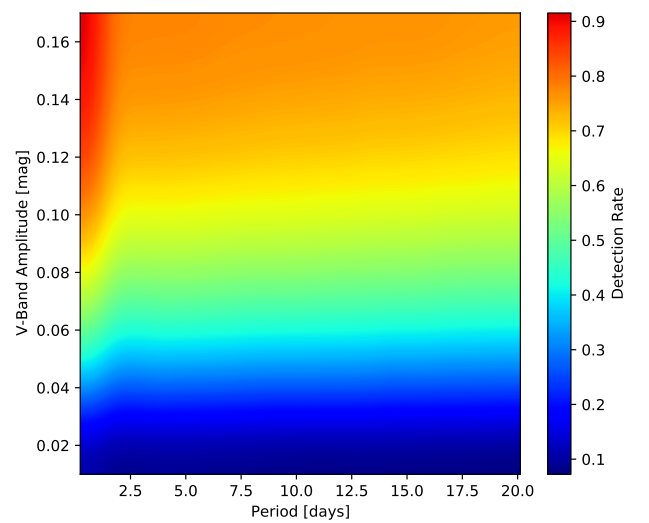
Figure 3. Simulated average detection rate in our data as described in Sect. 3.1 as a function of period and V-band amplitude.
