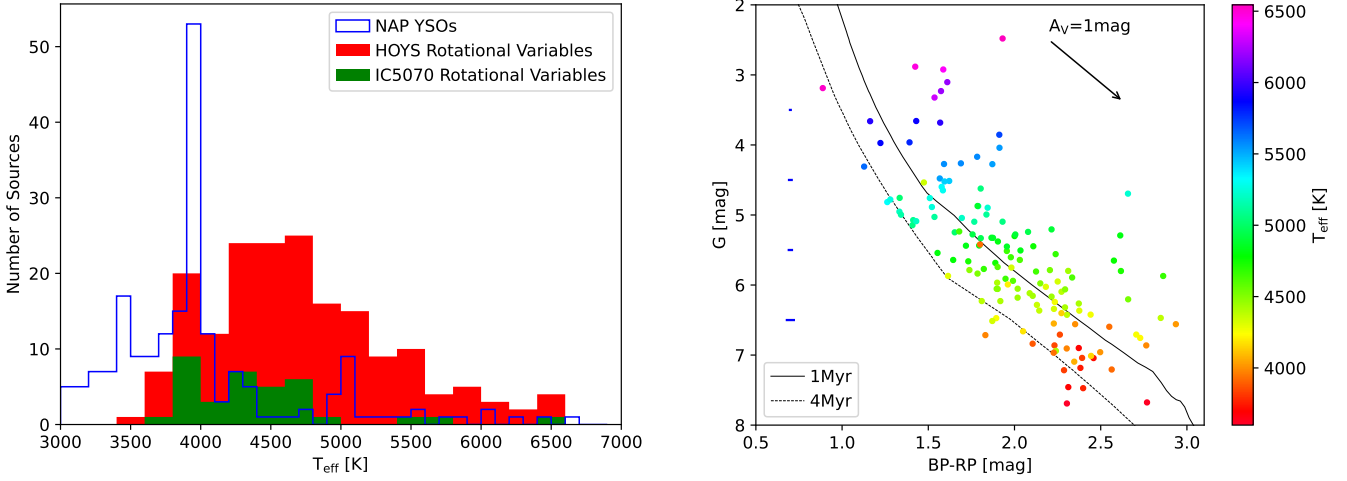
Figure 1. Left: In blue we show the T_{\text{eff}} distribution of the YSOs in the NAP region from Fang et al. (2020). In red the distribution of the fitted T_{\text{eff}} values for the rotational variables in all HOYS fields is displayed, while in green the subsample of sources in IC 5070 is shown. Right: A Gaia colour vs. absolute Gmag diagram of the rotational variables in our sample. The symbols are colour coded with the fitted T_{\text{eff}} values. Typical Gaia colour errors are indicated as blue lines on the left hand side. An extinction vector and 1 Myr and 4 Myr PARSEC isochrones from Bressan et al. (2012) are over plotted for reference.
