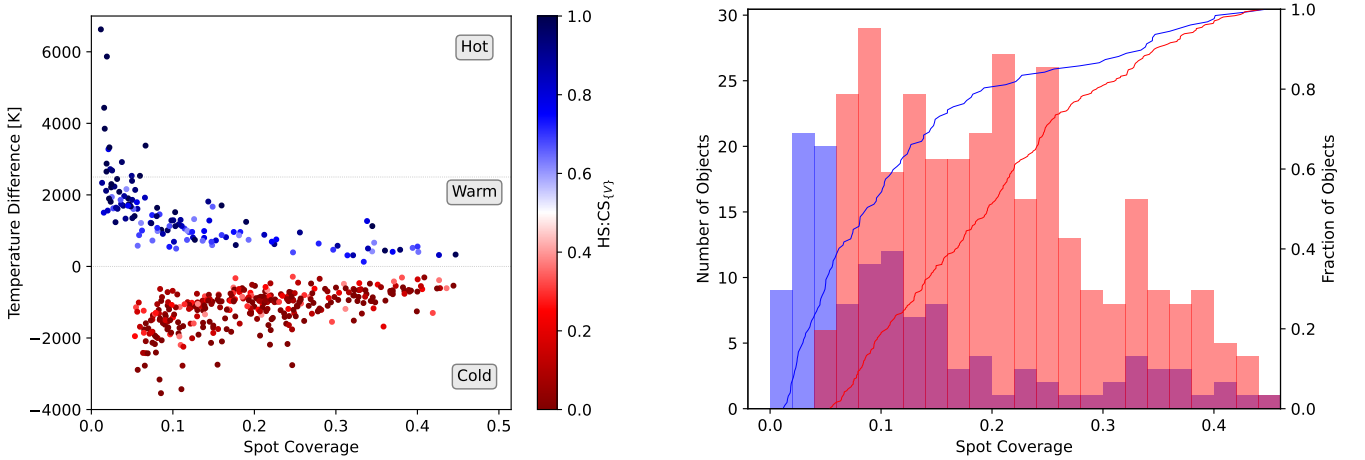
Figure 7. Left: Spot temperature difference T_S - T_\star versus spot coverage for the entire sample of rotational variables. Horizontal dotted lines mark T_S - T_\star = 0 K and T_S - T_\star = 2500 K, which separate the cold, warm and hot spot solutions. The symbols are colour coded according to the \text{HS:CS}_{(V)} ratio, our spot property quality indicator. Values close to zero indicate well constrained cold spot properties. Values near one indicate well constrained warm/hot spot properties. Values near 0.5 correspond to increasingly degenerate hot and cold spot solutions (see Herbert et al. 2024 , for details). The typical uncertainties of the spot coverage and temperature differences are 0.02 and 250 K, respectively. Right: Distribution of spot coverage of hot/warm (blue), and cold spots (red). The solid lines are the CDFs of the hot/warm (blue) and the cold spots (red).
