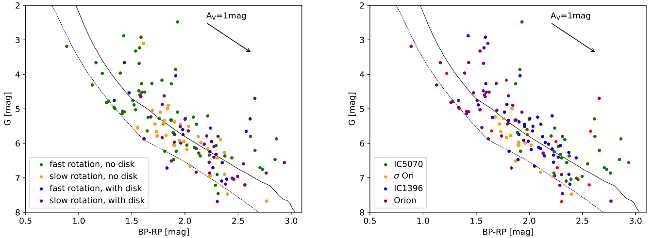
Figure 5. Gaia absolute magnitude vs. colour of the rotational variables. In the left panel the objects are colour coded based on their distribution in the period vs. K - W2 colour plot, and in the right panel according to the star formation region they are in. In all panels the solid black line is a 1 Myr PARSEC isochrone and the dashed black line a 4 Myr isochrone (Bressan et al. 2012).
