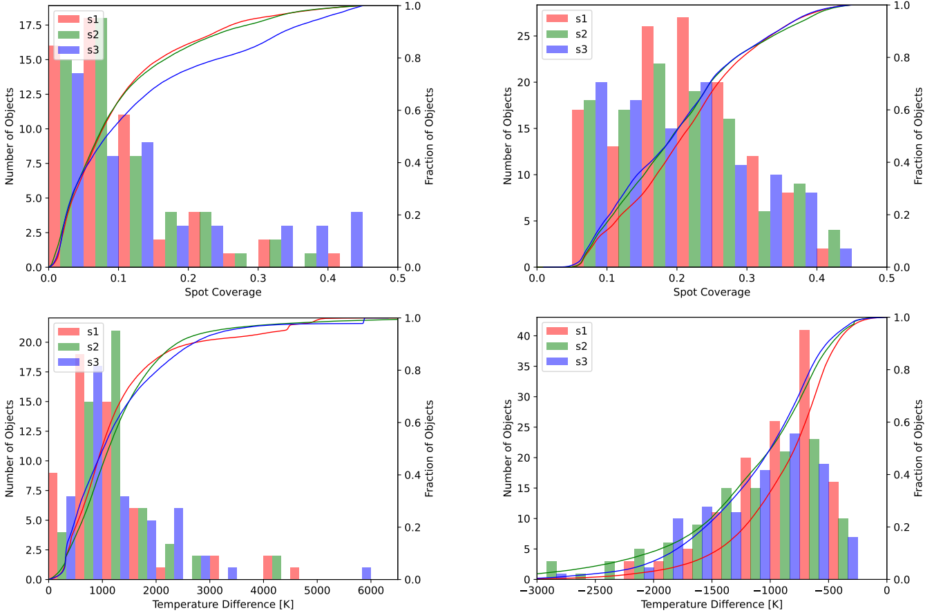
Figure 6. Comparison of spot property distributions from Herbert et al. (2024) and this work for IC 5070. Sample 1 is the original sample from Herbert et al. (2024) . In sample 2 we used the same amplitudes but our fitted values of T_{\text{eff}} . Sample 3 represents this work. Warm spot properties are in the left column, cold spot properties in the right. The top row shows the coverage distribution and the bottom row the star-spot temperature difference distribution.
