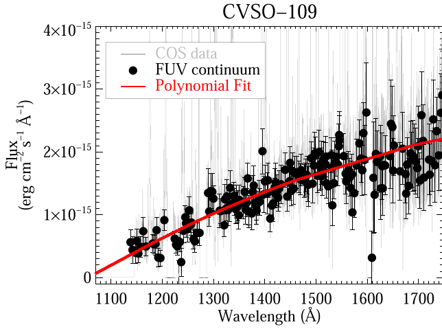
Figure 11. The FUV continuum spectrum of CVSO 109A. The full COS spectrum is shown in gray while the black filled circles are the average fluxes in 0.75 Å bins selected to exclude bright stellar and disk emission lines. A second-order polynomial fit is shown in red.
