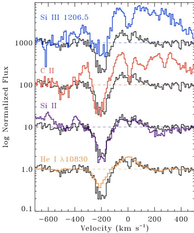
Figure 9. Wind profiles from lines of Si II (co-added), C II (co-added), Si III \lambda 1206.5 , and He I \lambda 10830 (colors), normalized to the surrounding continuum. Each profile includes a co-added profile (thin black spectrum) that combines the Si II and C II lines to help guide the eye. Narrow absorption features near 0 \text{ km s}^{-1} trace either interstellar or circumstellar material. All co-added profiles are combined in flux space.
