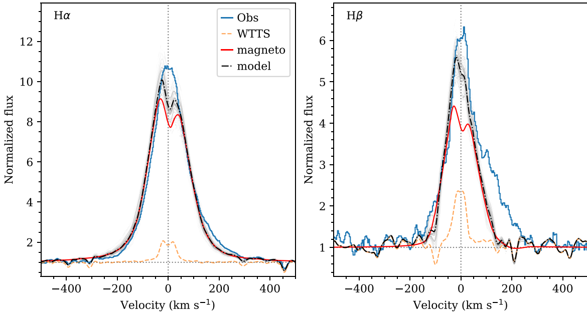
Figure 8. The extended accretion flow model fit to CHIRON spectrum of CVSO 109 in H \alpha (left) and H \beta (right) observed on MJD = 59181.70. The observation is shown in blue. The template photosphere and chromosphere, shown as dashed orange lines, are from UVES observation of the M0 WTTS TWA 25. The light gray lines are 100 best fits, and the red lines and the dashed-dotted black lines are the average magnetospheric profiles and the total magnetosphere + chromosphere + photosphere model profiles, respectively.
