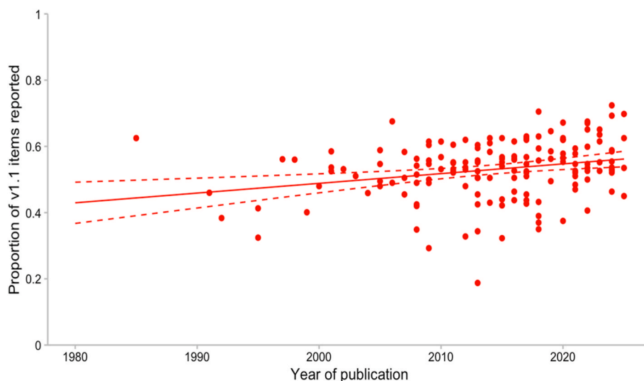
Fig. 4. Reporting completeness over time, defined as the proportion of TMS-RAT v1.1 items reported per study. The solid line shows the linear trend, and the dashed lines indicate the 95% CI. N = 153 studies with double ratings. For each article, the graph shows the mean proportions across two raters' ratings.
