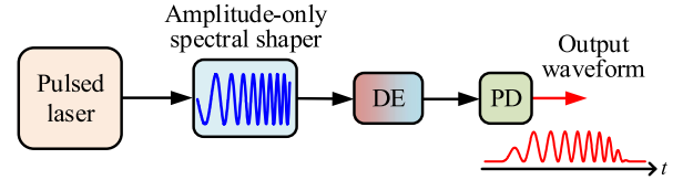
FIGURE 8. Chirped microwave waveform generation using an amplitude-only spectral shaper based on a spatial light modulator (SLM) (DE: dispersive element; PD: photodetector).
