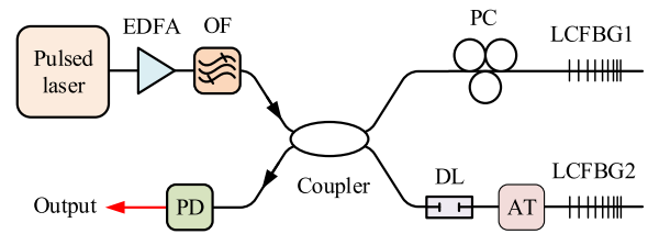
FIGURE 3. Photonic generation of a linearly chirped microwave waveform using a pair of LCFBGs with slightly different chirp rate (EDFA: erbium-doped fiber amplifier; OF: optical filter; PC: polarization controller; CFBG: chirped fiber Bragg grating; DL: delay line; AT: attenuator; PD: photodetector) [16].
