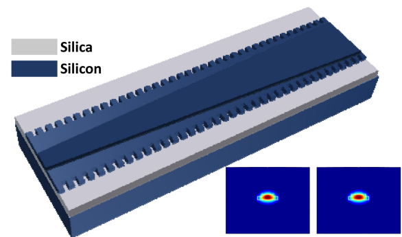
FIGURE 20. Perspective view of an integrated chirped grating. Inset: Simulated fundamental TE mode profile of the rib waveguide with the rib width of 500 nm (left) and 650 nm (right).
