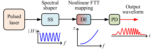
FIGURE 12. Generation of a chirped microwave waveform based on uniform spectral shaping and nonlinear FTT mapping (using a nonlinear group delay dispersive element).
