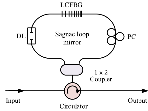
FIGURE 5. Spectral shaper based on a Sagnac loop mirror incorporating an LCFBG (LCFBG: linearly chirped fiber Bragg grating; DL: delay line; PC: polarization controller) [19].
