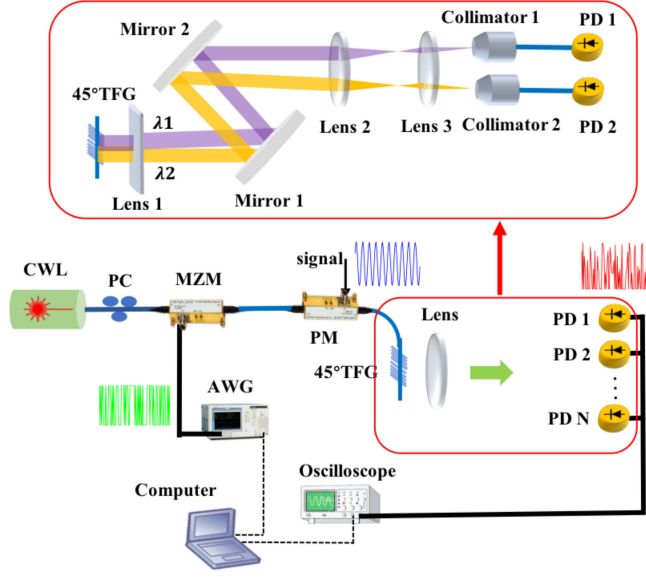
Fig. 2. Schematic of the proposed FSO communication system. FSO: free-space optical; CWL: continuous wavelength laser; PC: polarization controller; MZM: Mach-Zehnder modulator; AWG: arbitrary wavelength generator; PM: phase modulator; TFG: tilted fiber grating; PD: photo-detector.
