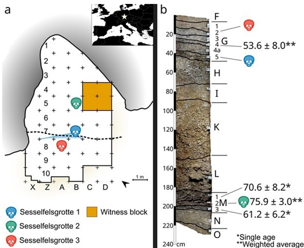
Figure 2. Stratigraphic context of skeletal and dental Neanderthal remains at Sesselfelsgrötte. (a) Planimetry of the cave in its current state, showing the location of the Neanderthal remains Sesselfelsgrötte 1 to 3. The white star in the upper right panel indicates the geographic location of the rock shelter. (b) Stratigraphic log from the witness block in square C5 displaying the vertical position of Neanderthal fossils together with available geochronological data, based on published, but recalculated, thermoluminescence results [19]. The recalculated thermoluminescence dates exclude samples that Richter [78] considered as not indicative of Neanderthal occupation.
