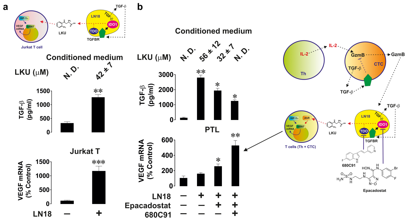
Figure 4. LKU downregulates HIF-1 activity in primary human T cells interacting with cancer cells. (a) Jurkat T cells (which do not express AhR) were co-cultured for 16 h with LN18 cells at a ratio of 1:1. VEGF mRNA levels in Jurkat T cells and TGF- \beta as well as LKU levels were then measured in the conditioned medium. (b) Primary human CD3-positive T cells (express AhR) were co-cultured for 16 h with LN18 cells at a ratio of 1:1 in the absence or presence of 1 \mu M epacadostat (IDO1 inhibitor) or combination of 1 \mu M epacadostat and 1 \mu M 680C91 (TDO inhibitor). VEGF mRNA levels in T cells and TGF- \beta as well as LKU levels were then measured in the conditioned medium. Quantitative data are shown as mean values \pm SEM of four independent experiments. * p < 0.05 and ** p < 0.01 vs control.
