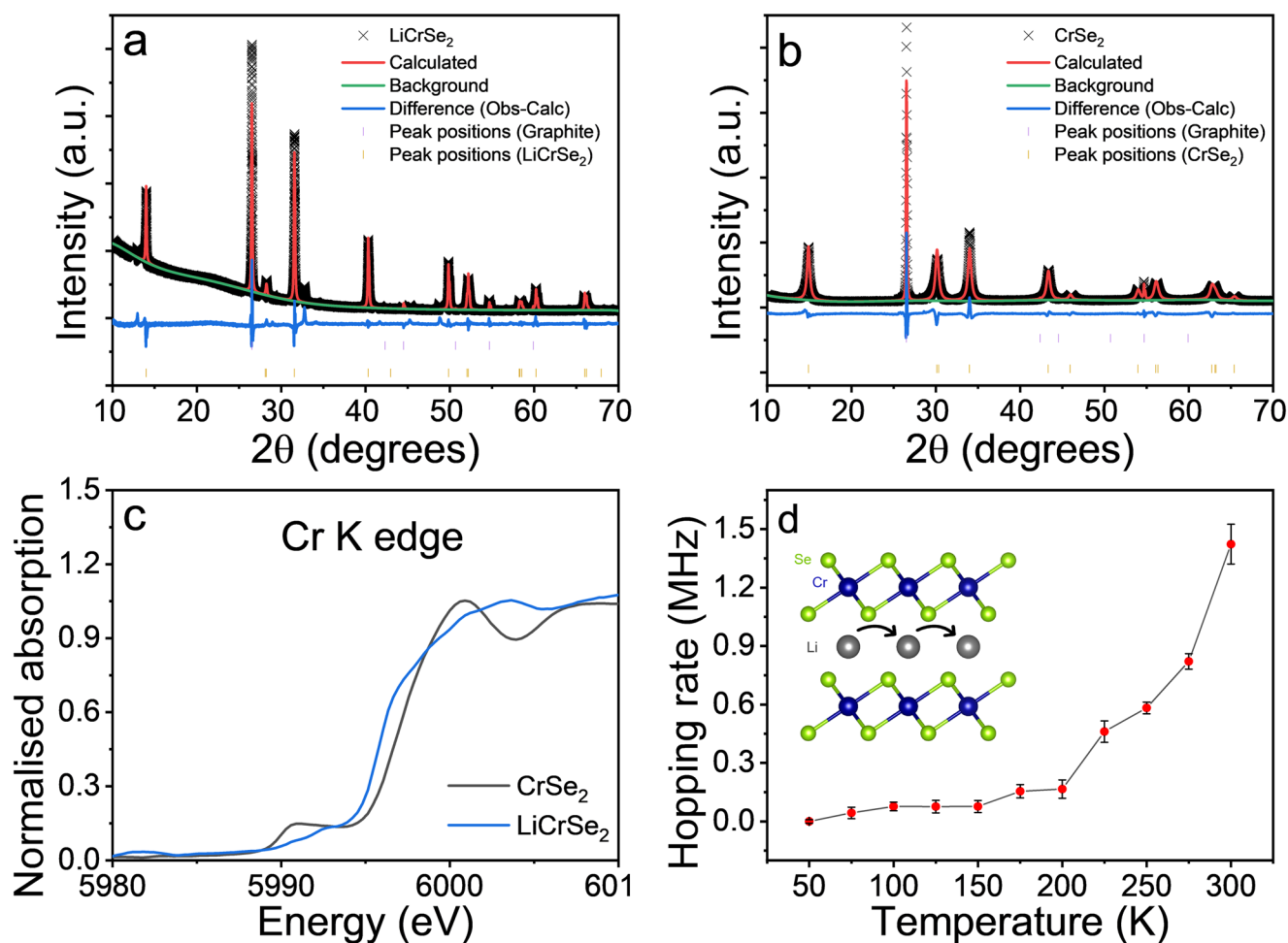
FIGURE 2 | Le Bail refinements of experimental PXR patterns (Cu K\alpha ) for (a) LiCrSe 2 and (b) CrSe 2 . Measured data are shown as black crosses, calculated profiles as red lines, and different curves as blue lines. Magenta vertical bars indicate the expected Bragg reflection positions of the phase, (c) Cr K-edge XANES profile of CrSe 2 and LiCrSe 2 , and (d) Temperature dependence of the Li-ion hopping rate ( \nu_{Li} ) from \mu^+ SR measurements.
