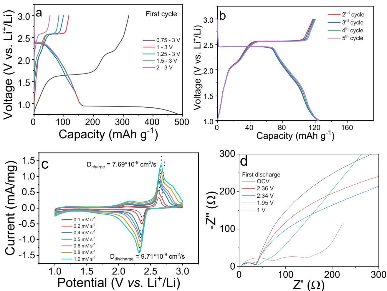
FIGURE 3 | (a) GCD profiles for the 1st cycle of \text{CrSe}_2 recorded at different lower cut off voltages (0.75, 1, 1.25, 1.5, and 2 V), (b) GCD curves (from 2nd cycle) of \text{CrSe}_2 within the voltage window of 1–3 V at 0.1C, (c) CV curves of \text{CrSe}_2 at various scan rates ( 0.1\text{--}1\text{ mV s}^{-1} ) in the voltage range of 1–3 V, with calculated diffusion coefficients for charge and discharge processes. And (d) Electrochemical impedance spectrum measured at different potentials.
