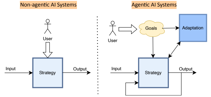
Fig. 1. Reactive non-agentic AI versus Goal-driven agentic AI
